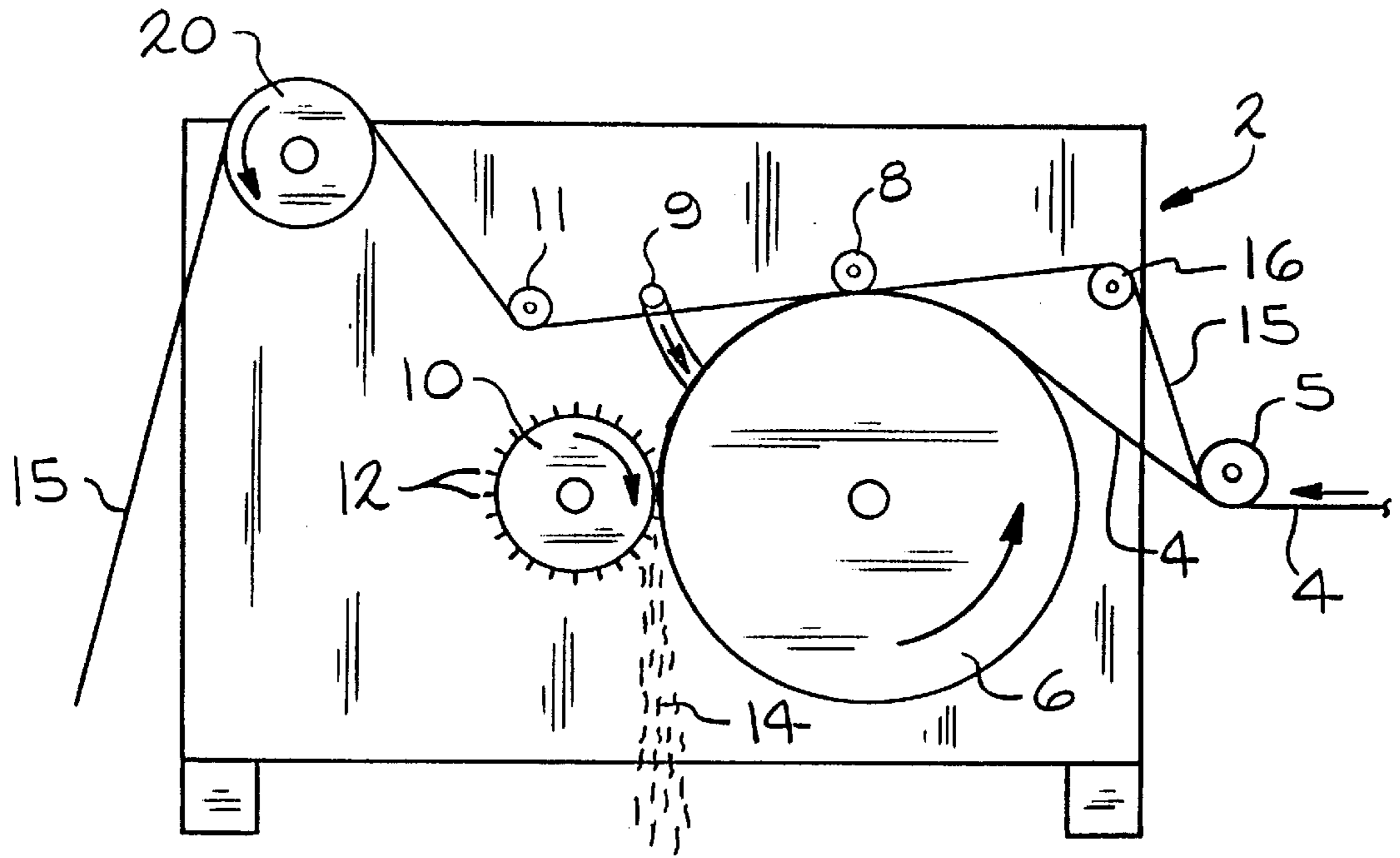
FIG. 1 (PRIOR ART)
