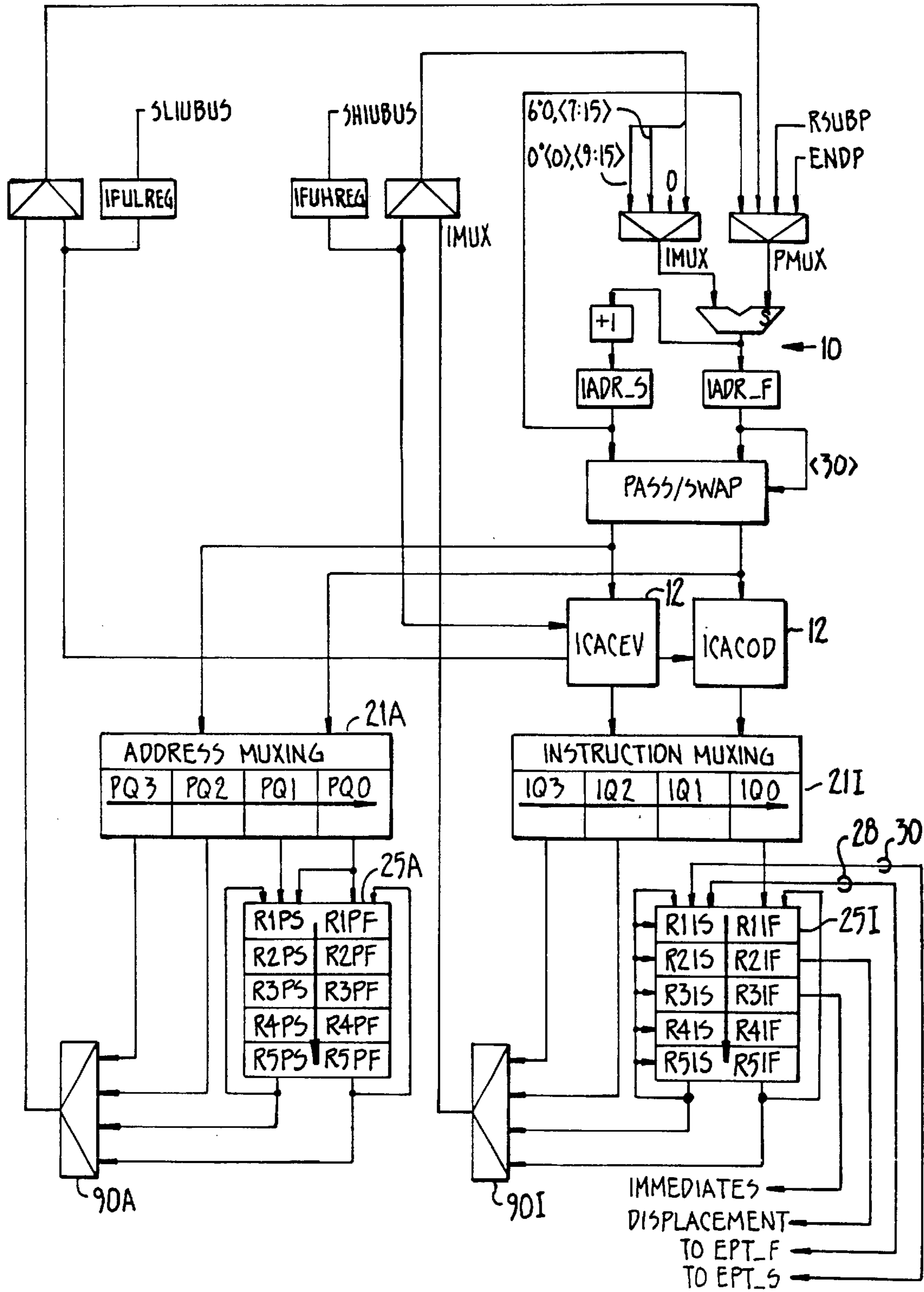
INSTRUCTION CACHE, QUEUE, AND PIPELINE
