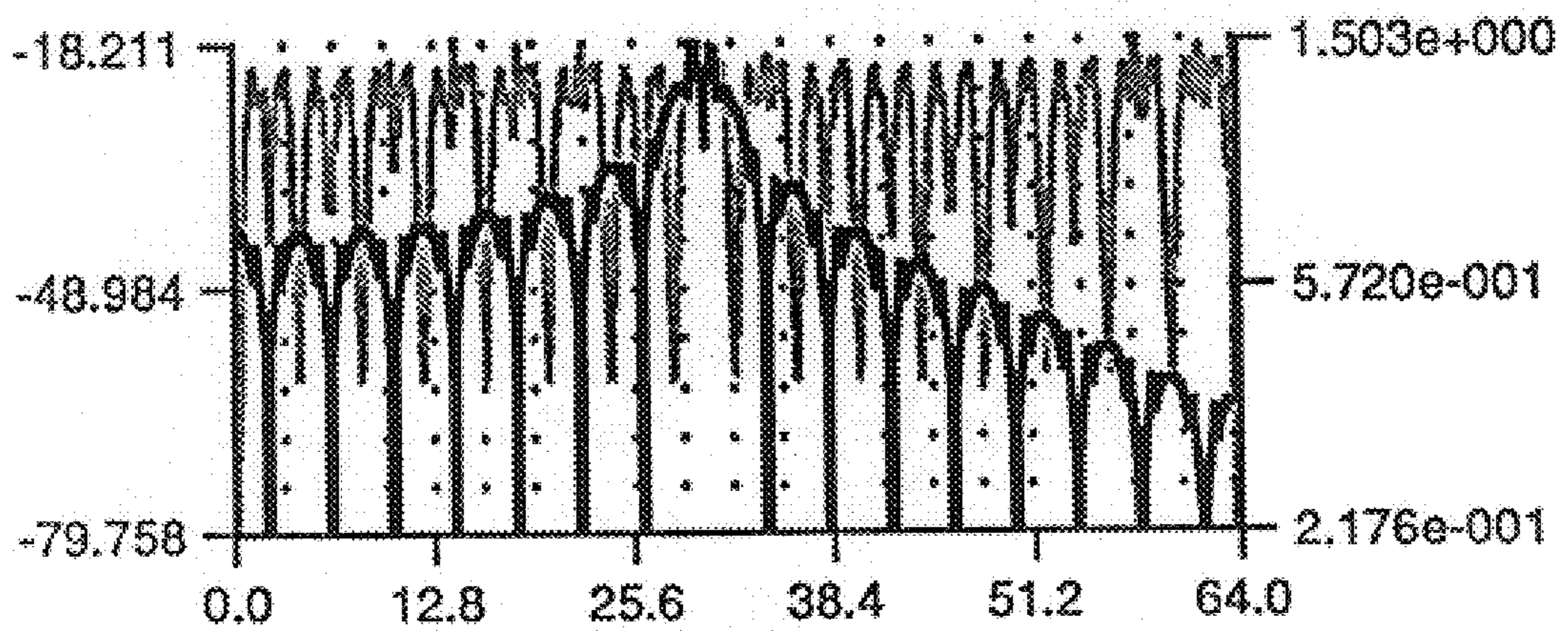
AMPLITUDE ON-OFF PLUS BIPHASE CARRIER MODULATION SPECTRUM
