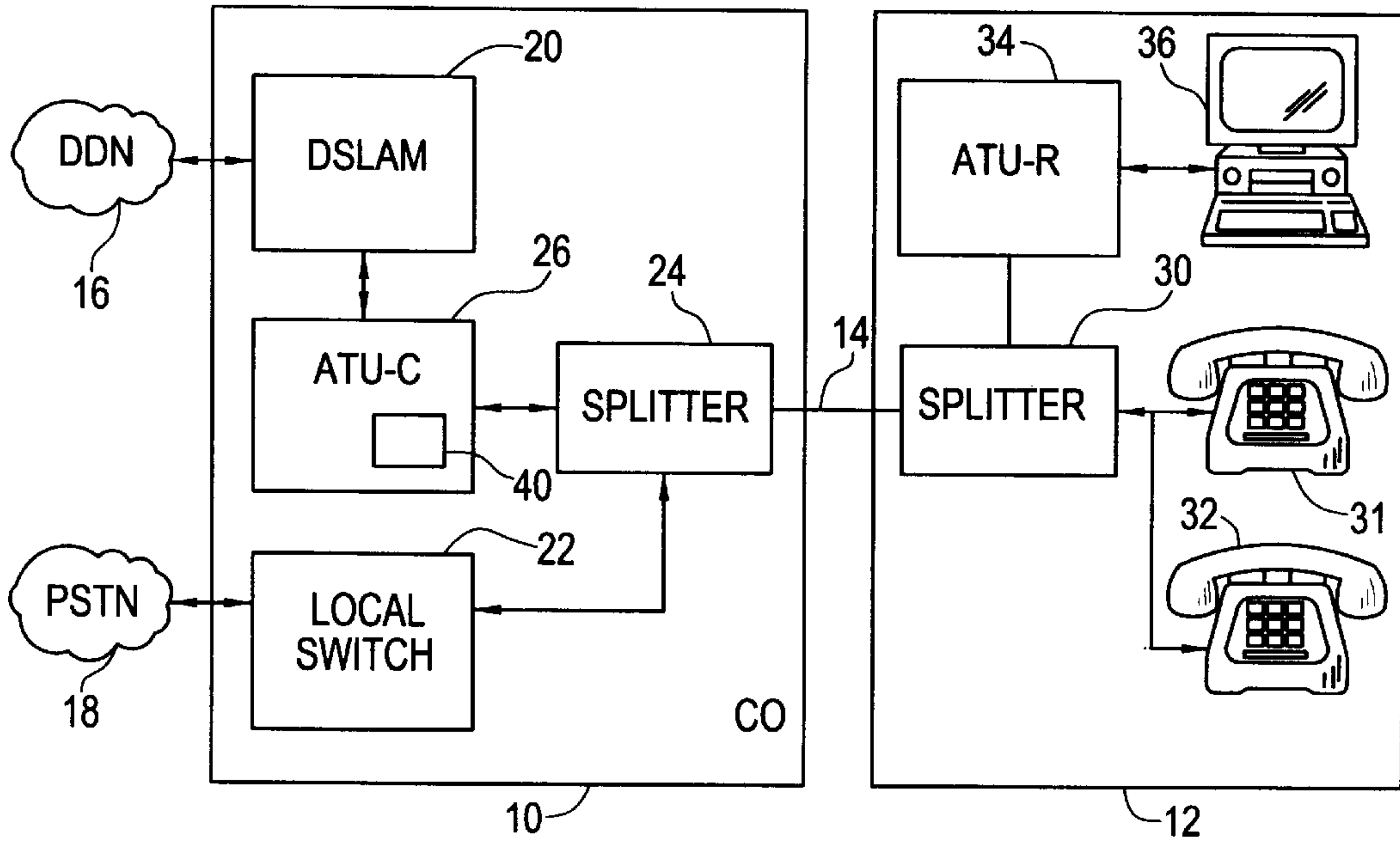
FIG. 2 PRIOR ART
