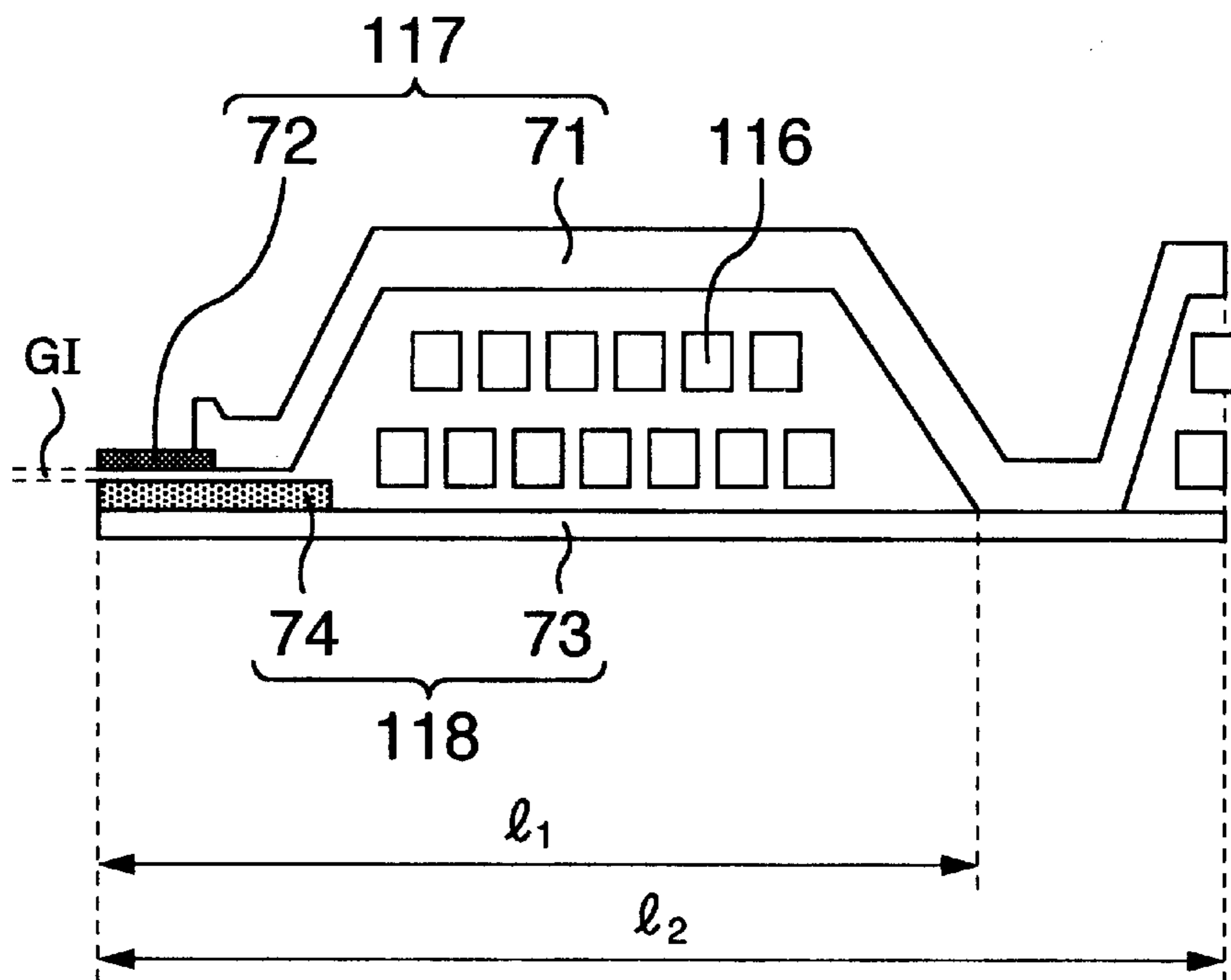
CROSS SECTION
