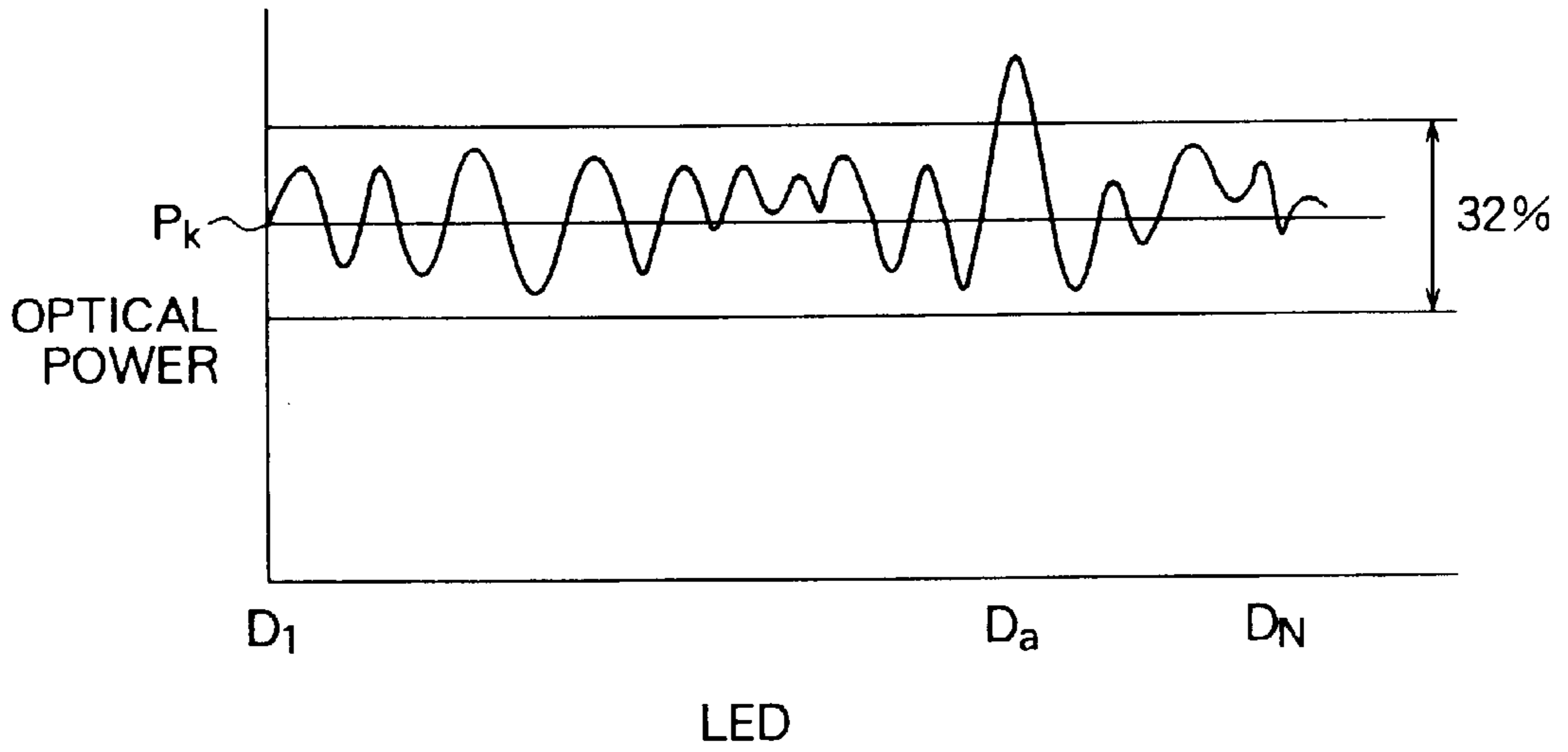
FIG. 3 PRIOR ART
