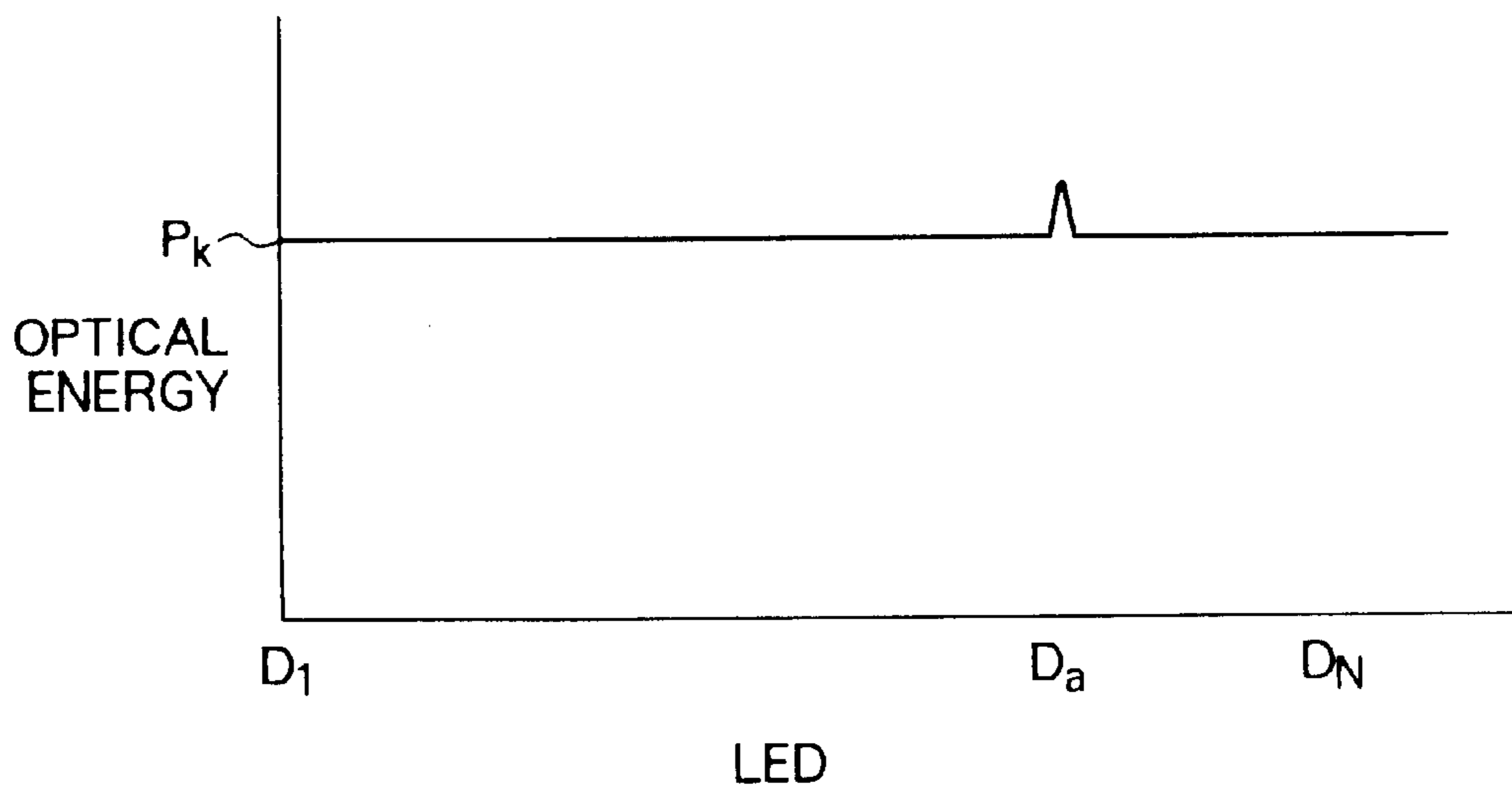
FIG. 4 PRIOR ART
