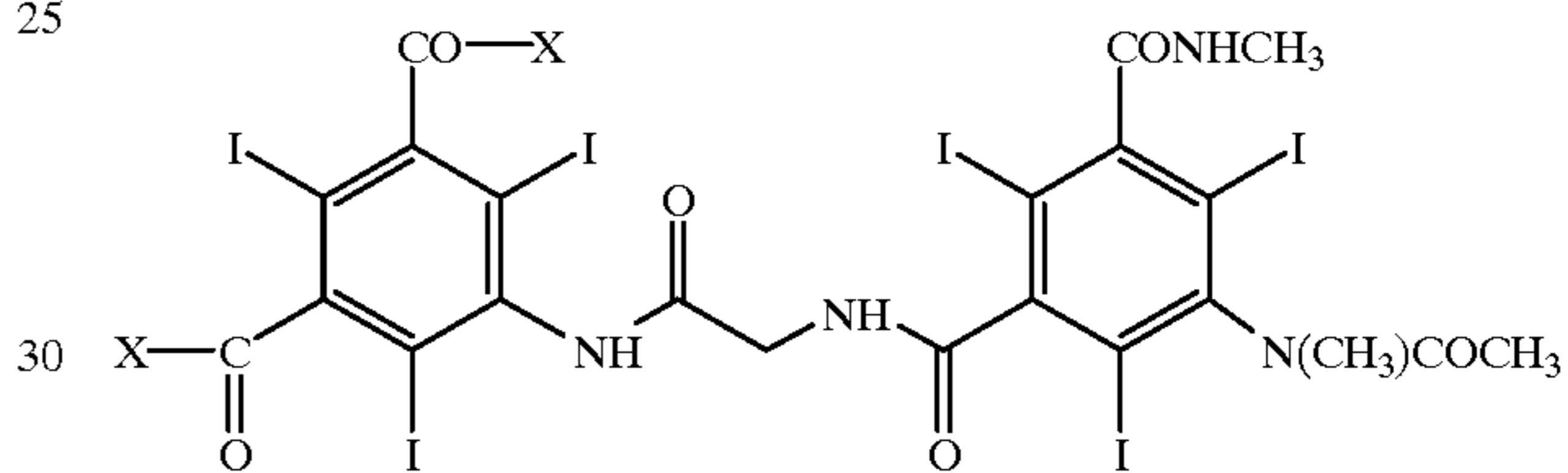
Compound 13
