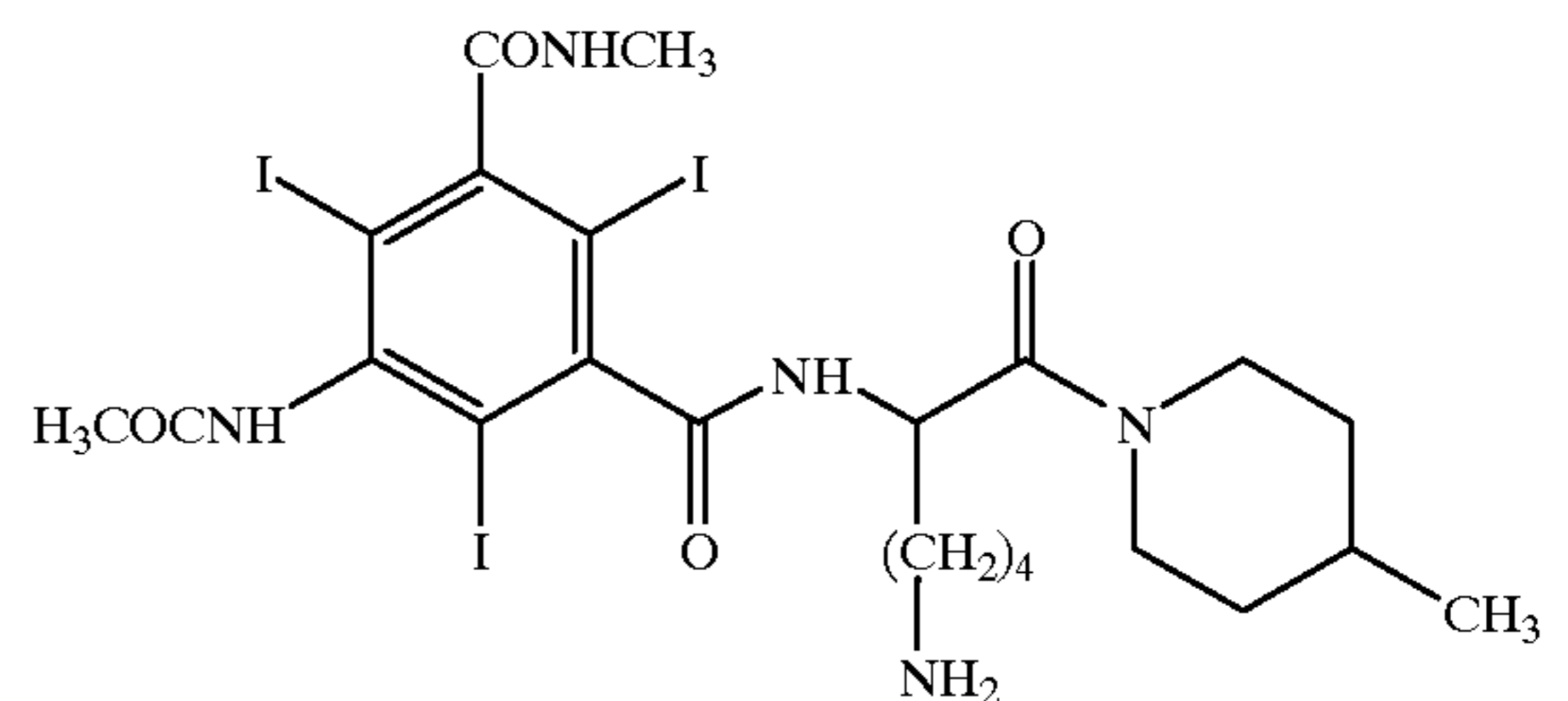
Compound 10
