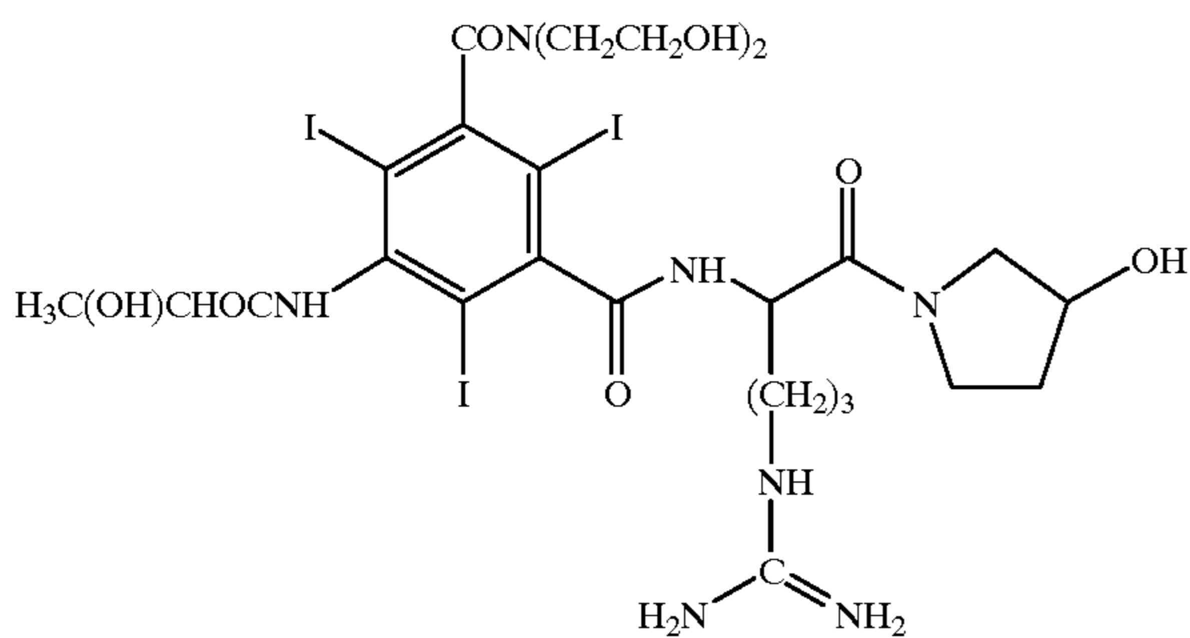
Compound 13
