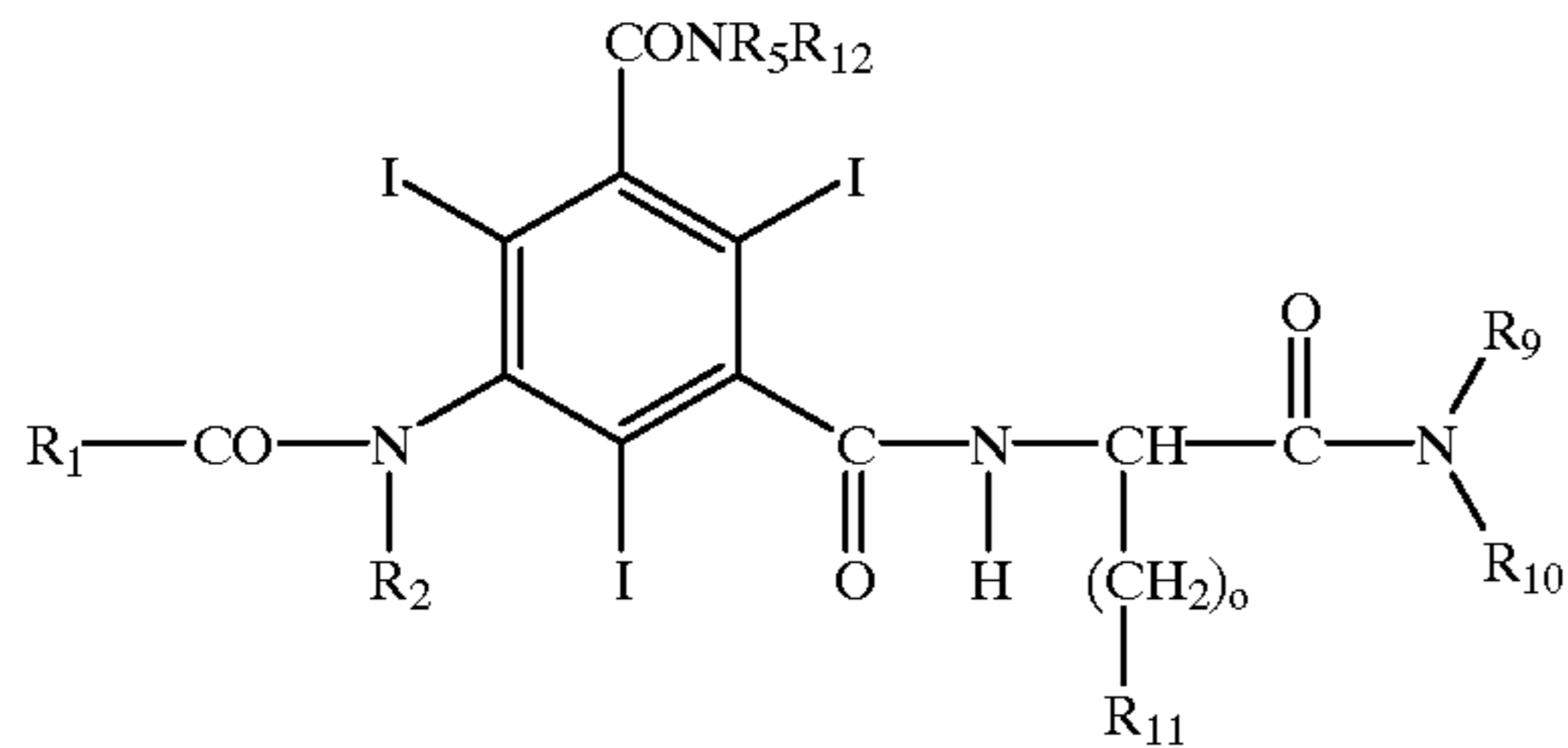
Formula II
