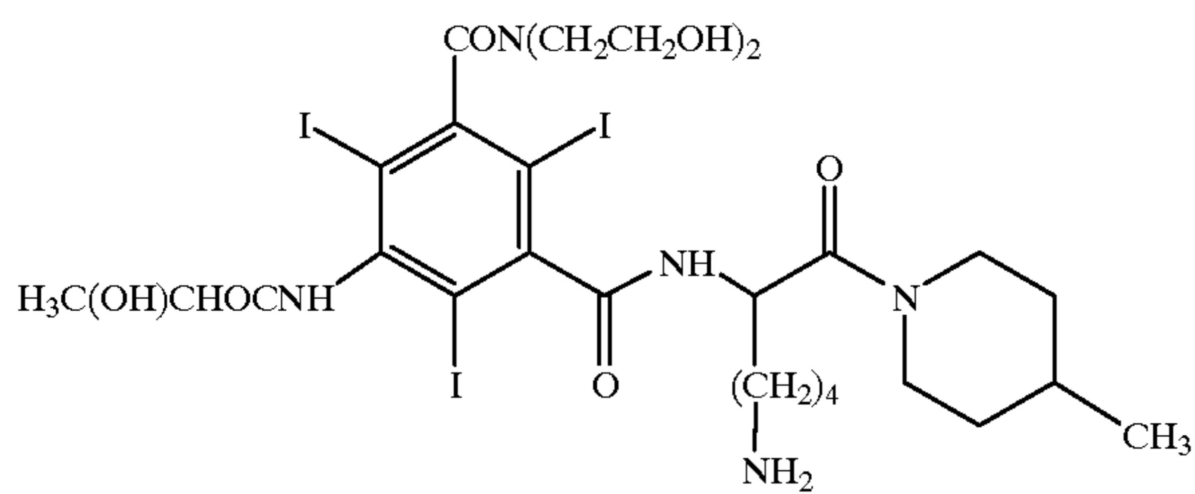
Compound 11
