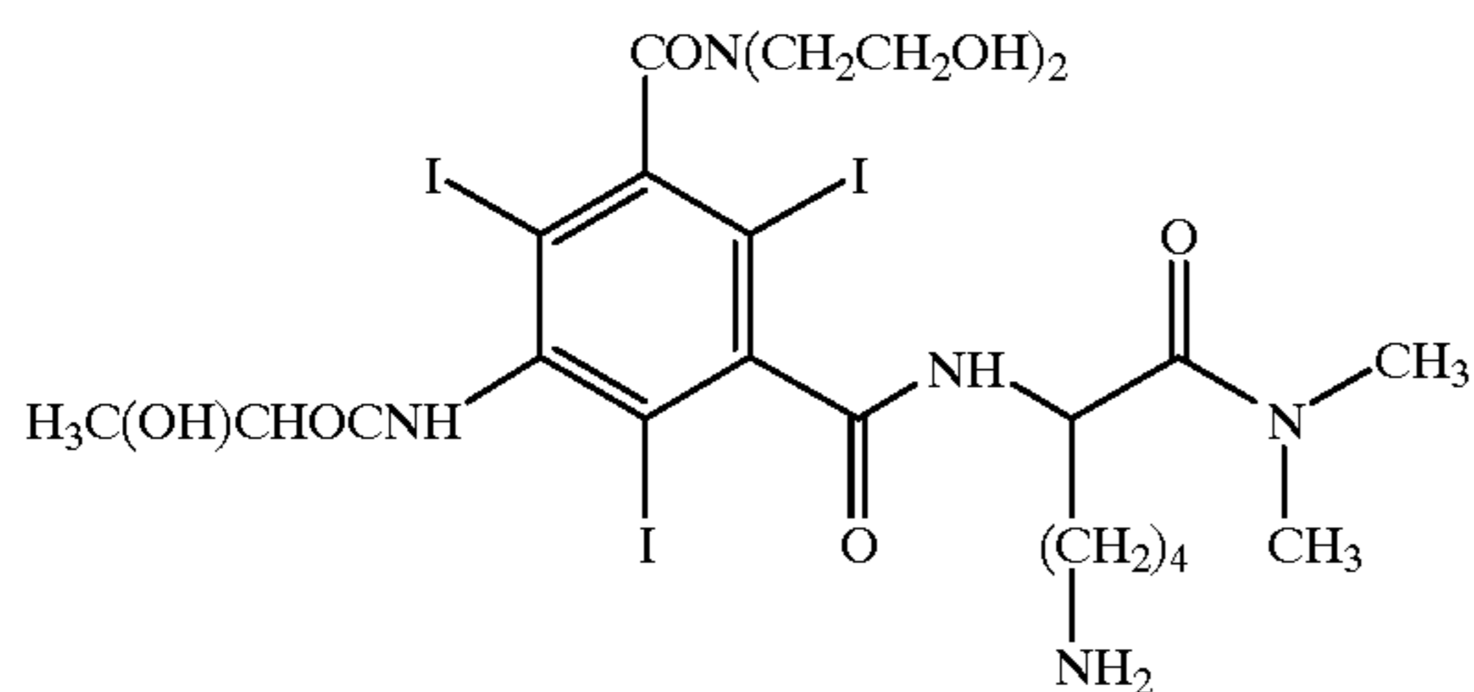
Compound 12
