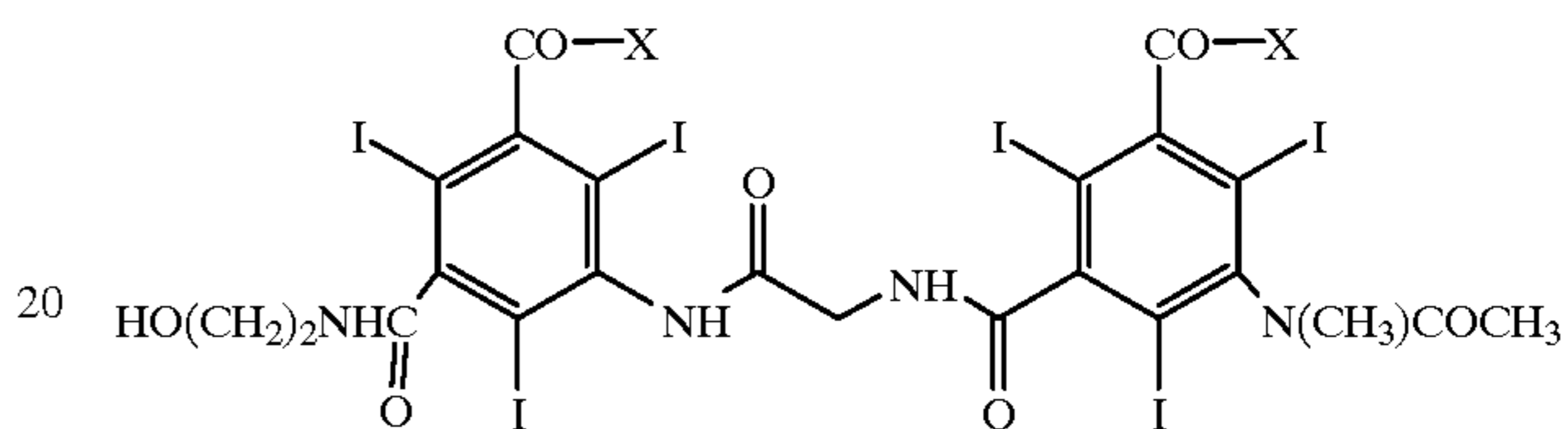
Compound 12
