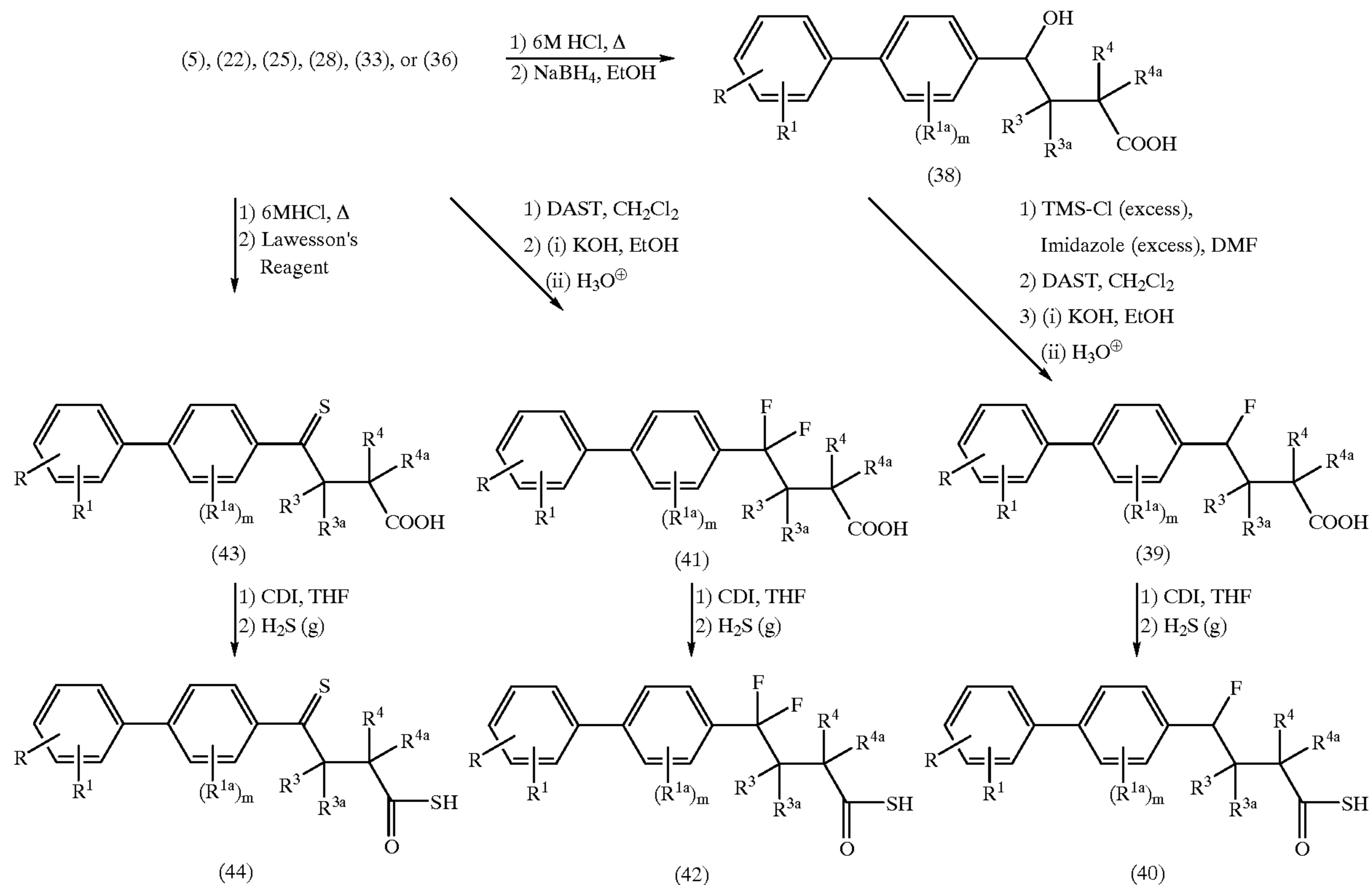
SCHEME 5
