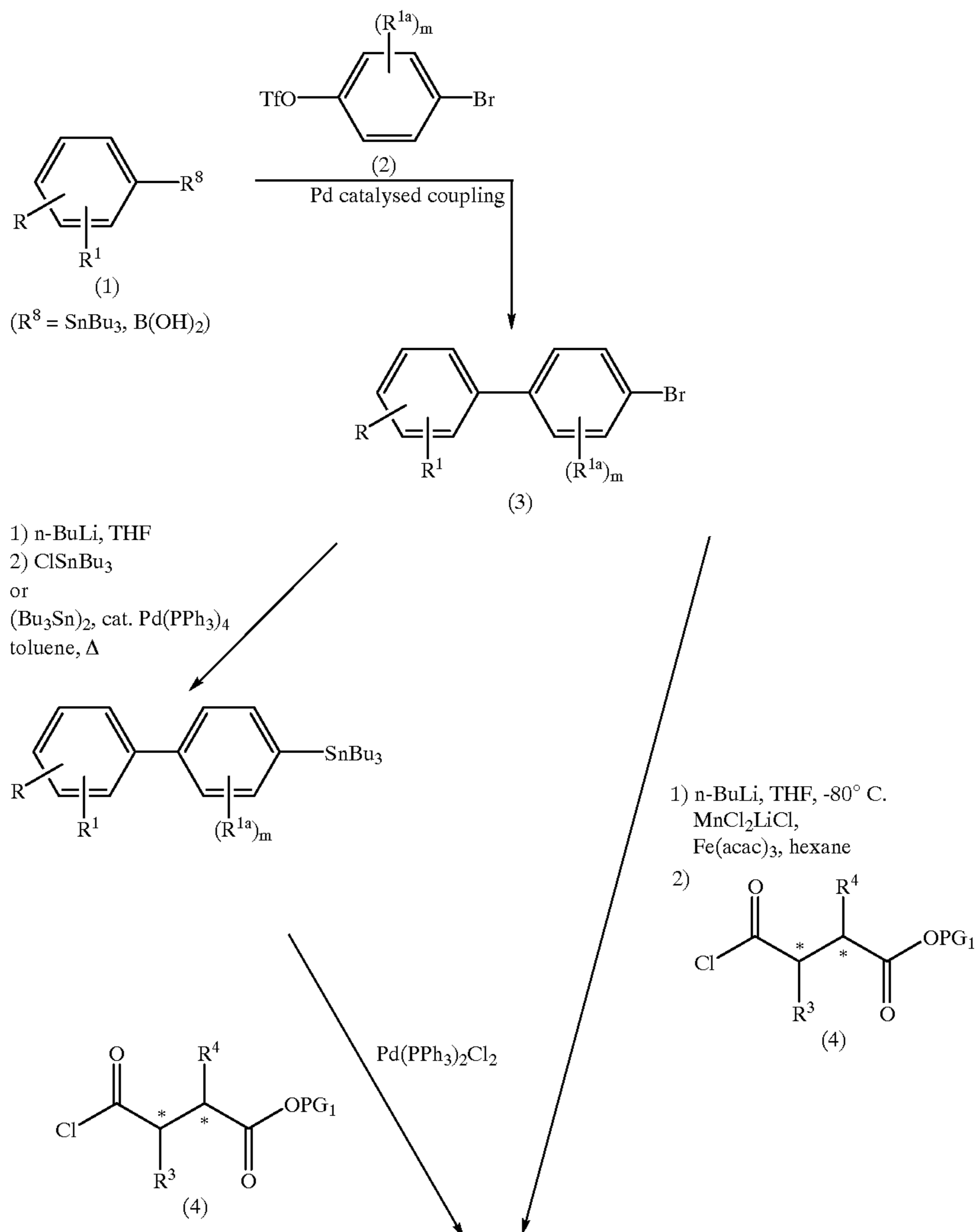
SCHEME 1
