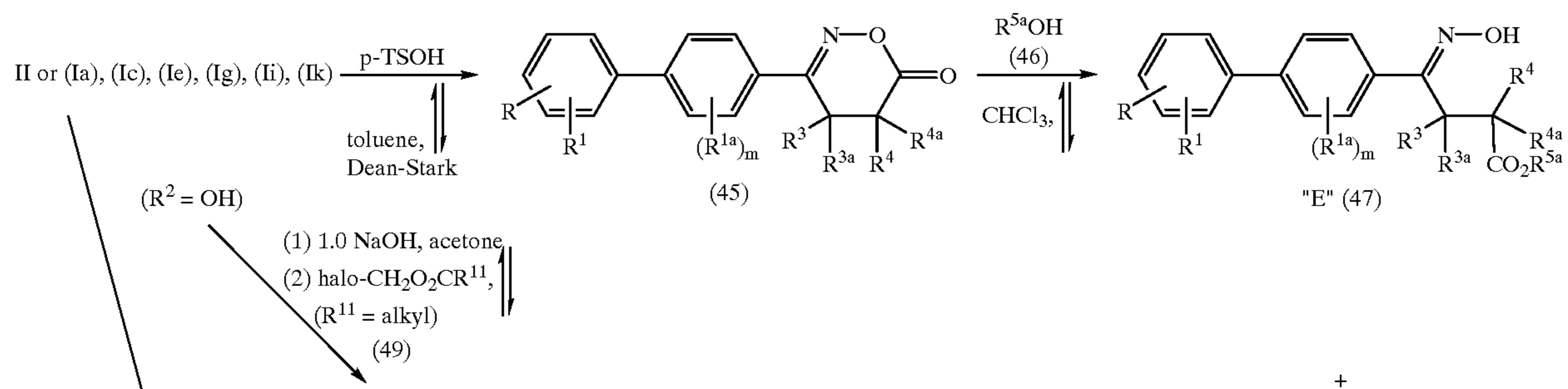
SCHEME 6
