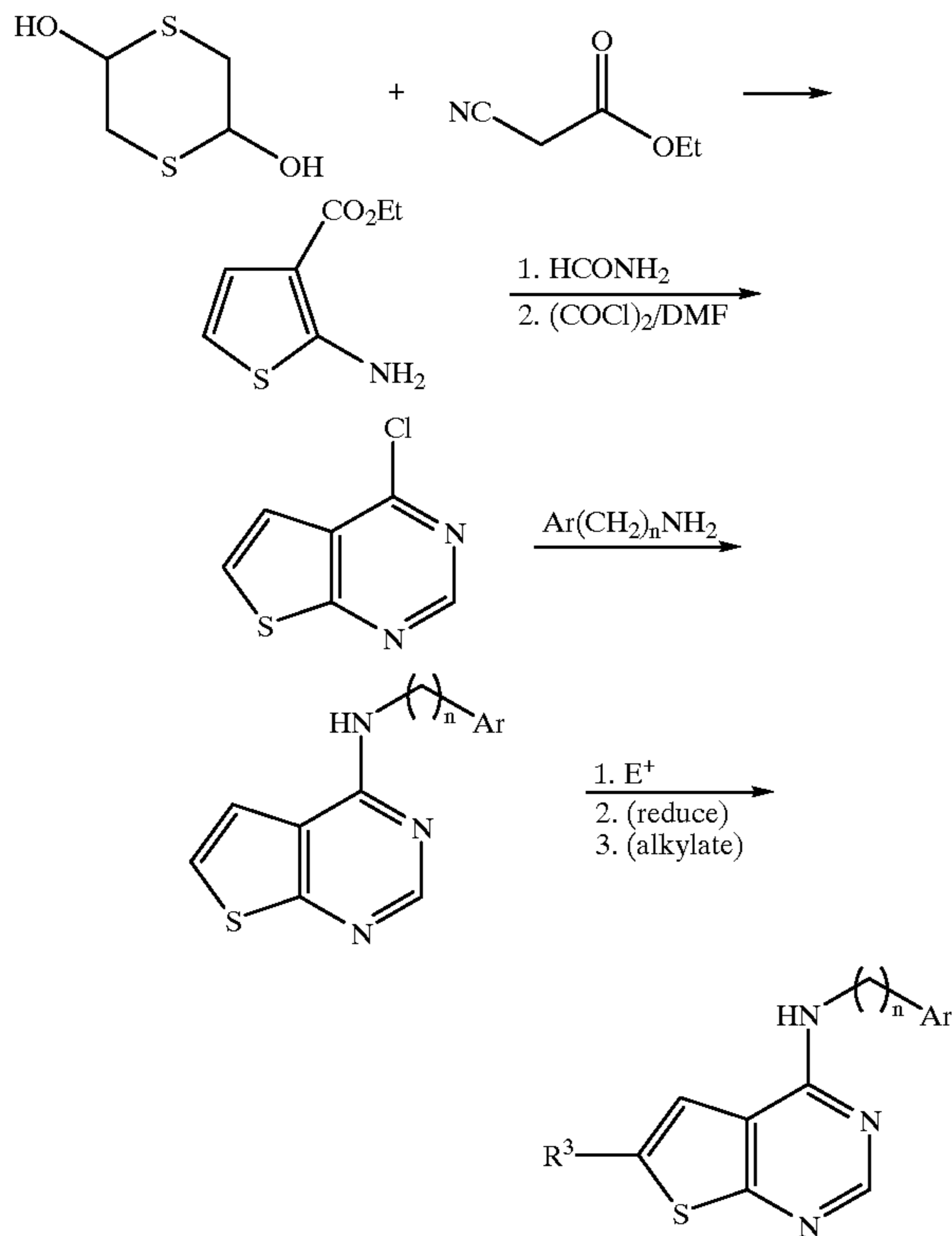
Scheme 18 Synthesis of Preferred Group 41; [2,3-d] ring fusion
