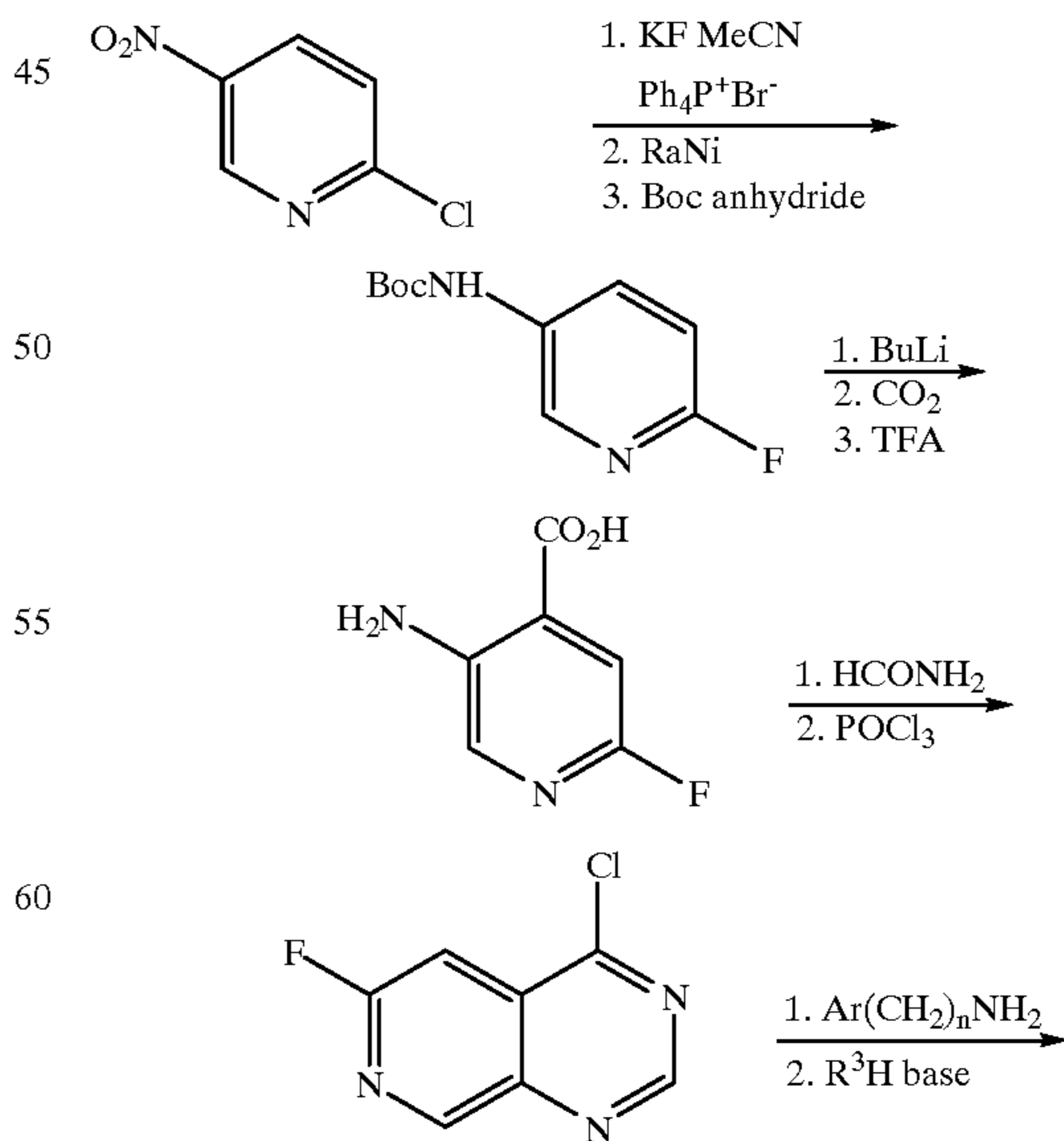
Scheme 8 Synthesis of Preferred Groups 17-21.
