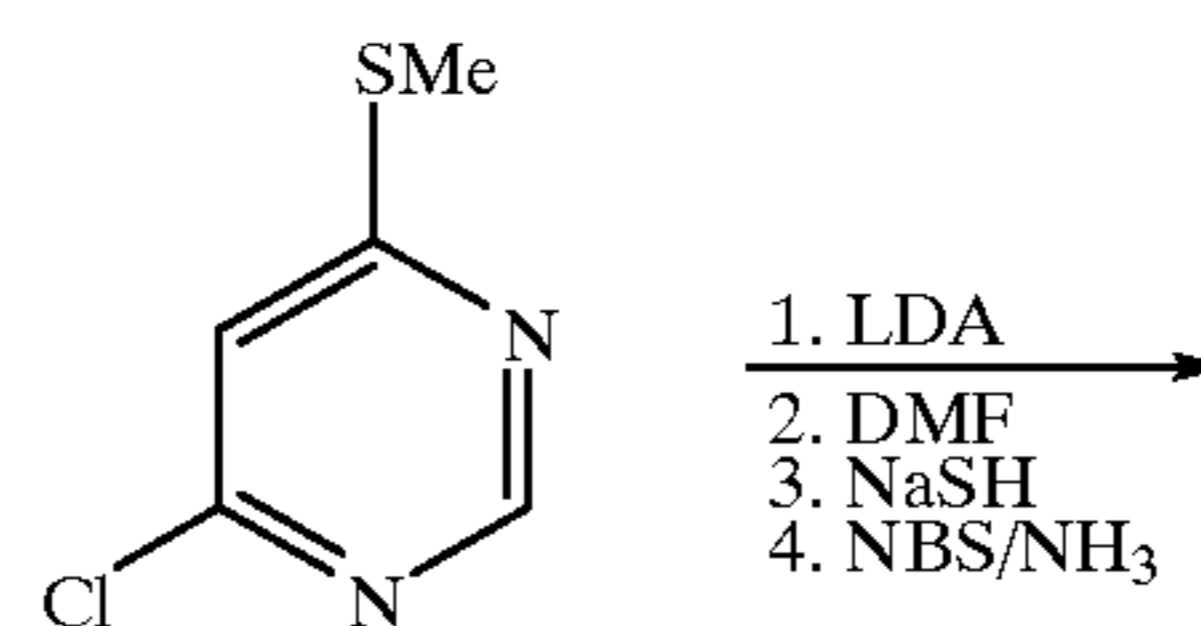
Scheme 30 Synthesis of Preferred Group 48; [5,4-d] ring fusion.
