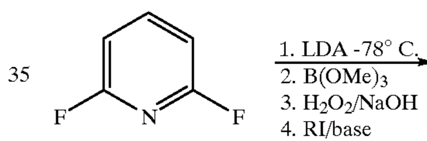
Scheme 11 Synthesis of Preferred Groups 27 & 29–31: R 3 = RO
