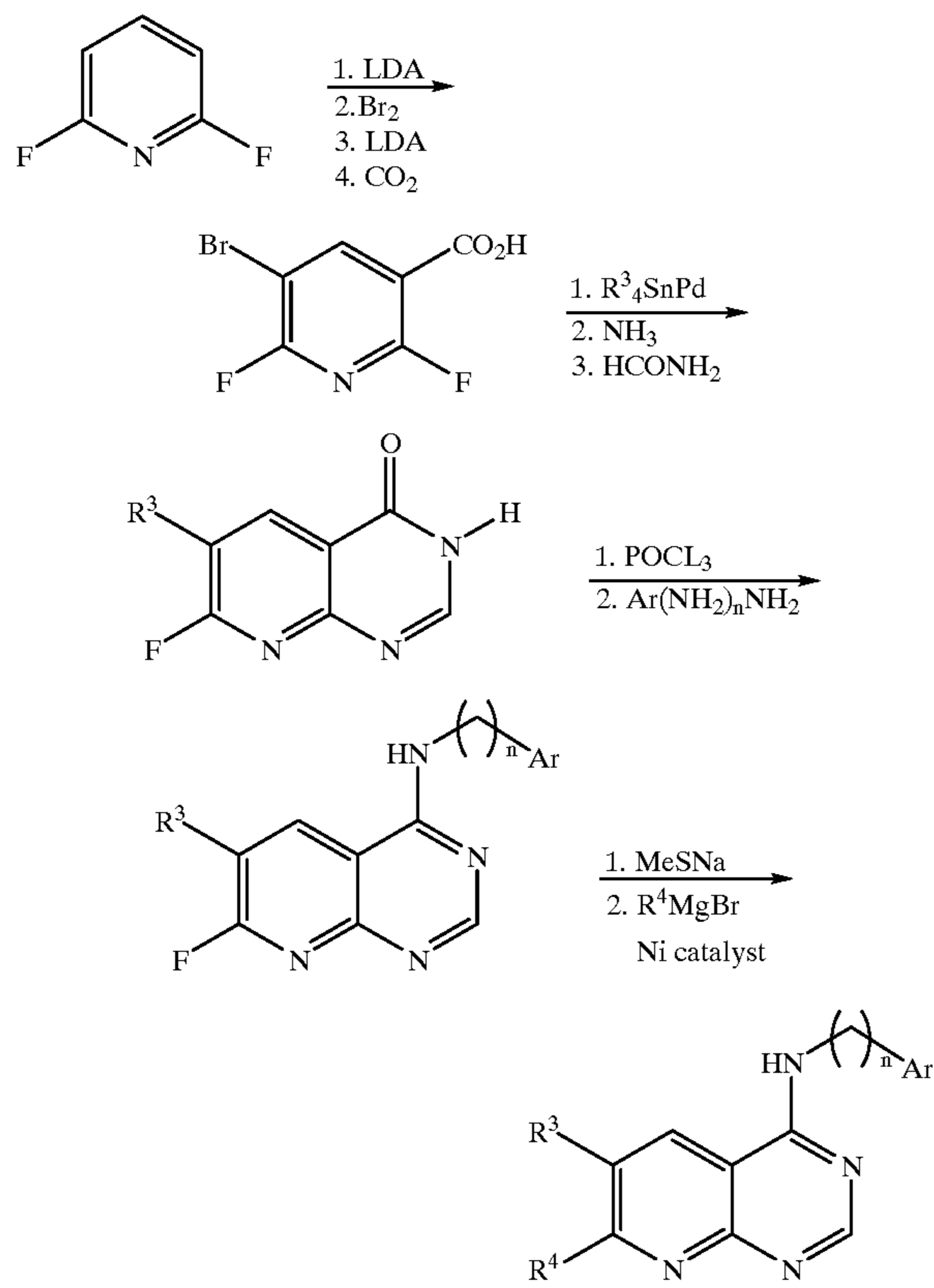
Scheme 12 Synthesis of Preferred Groups 28
