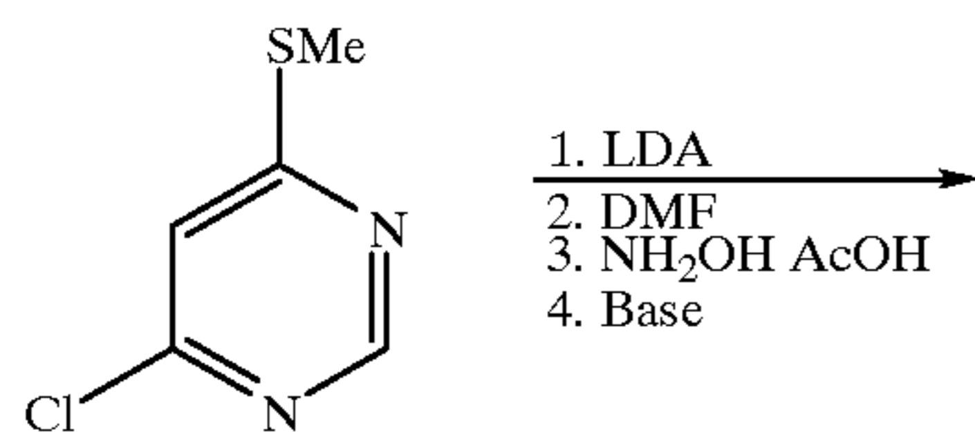
Scheme 28 Synthesis of Preferred Group 47; [5,4-d] ring fusion
