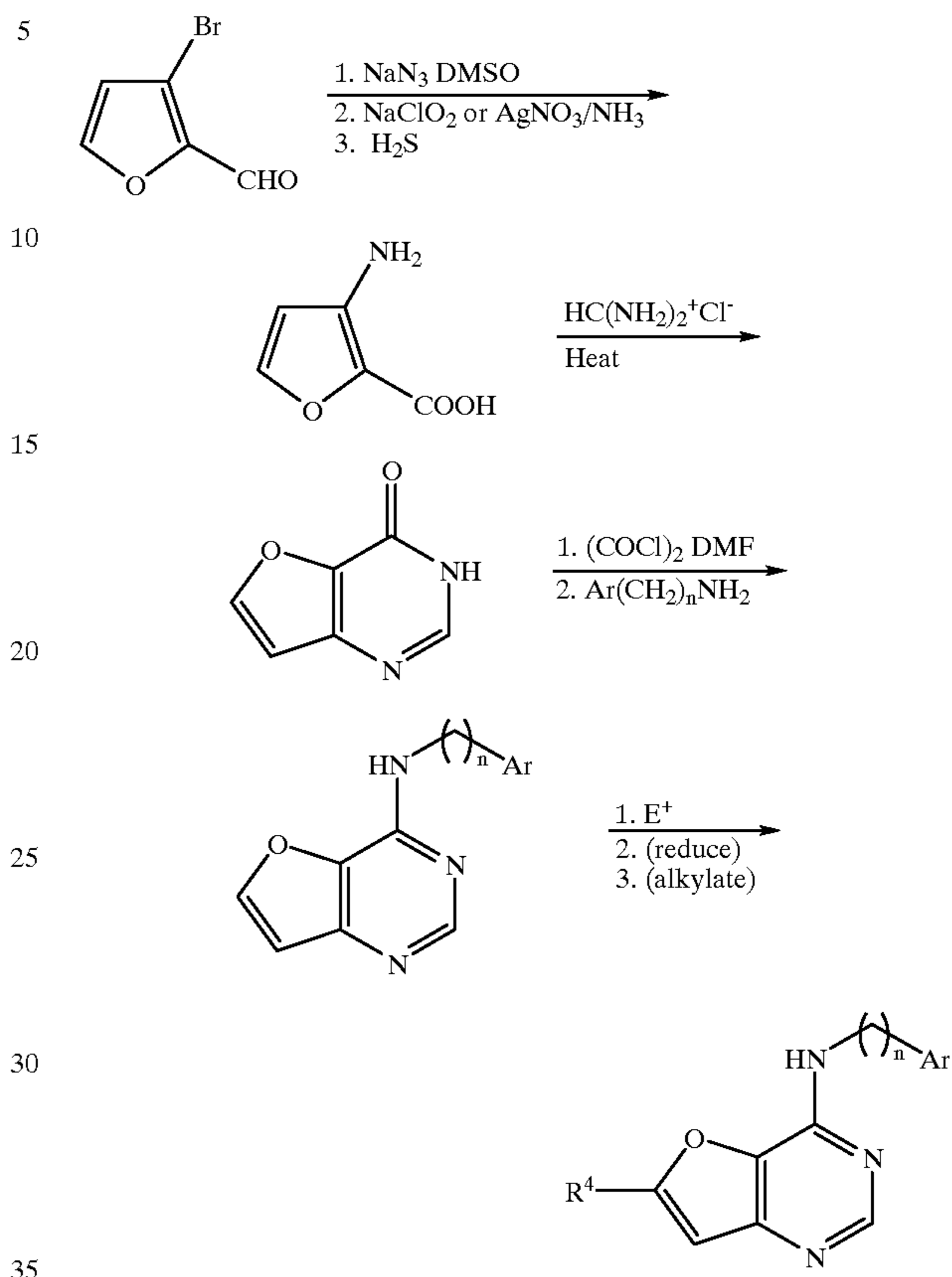
Scheme 19 Synthesis of Preferred Group 42; [3,2-d] ring fusion
