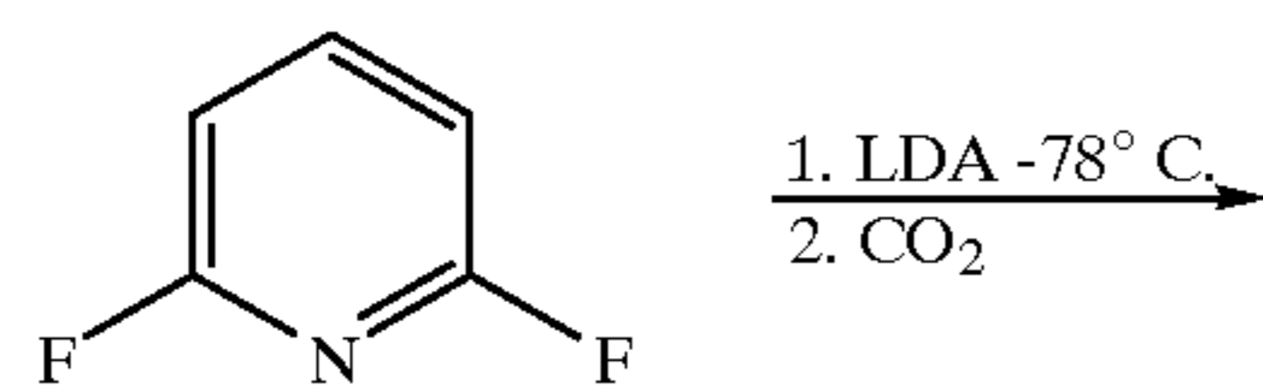
Scheme 10 Synthesis of Preferred Groups 22–26: R 3 = H.
