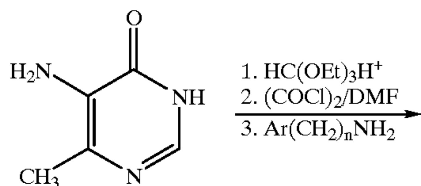
Scheme 22 Synthesis of Preferred Group 43; [3,2-d] ring fusion
