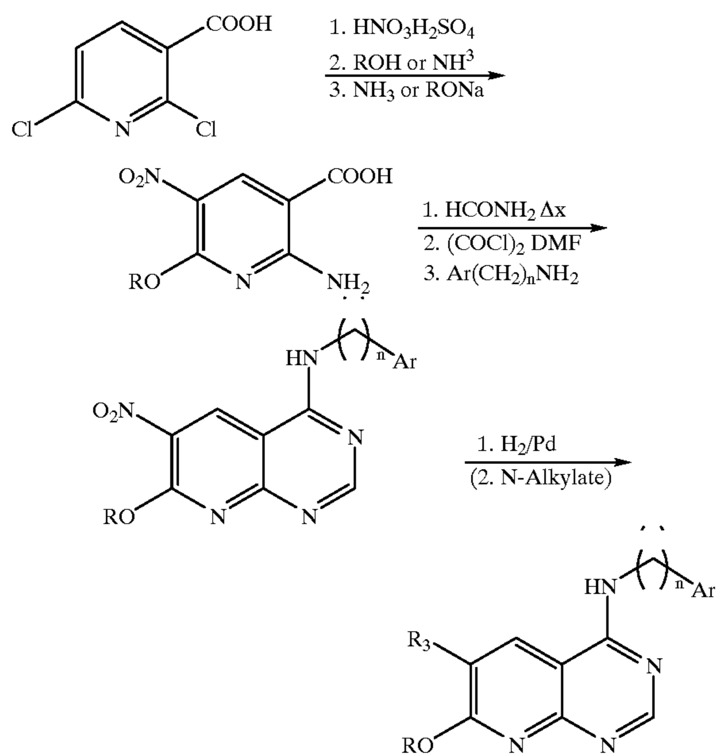
Scheme 13 Synthesis of Preferred Groups 29 & 30: R^4 = OR
