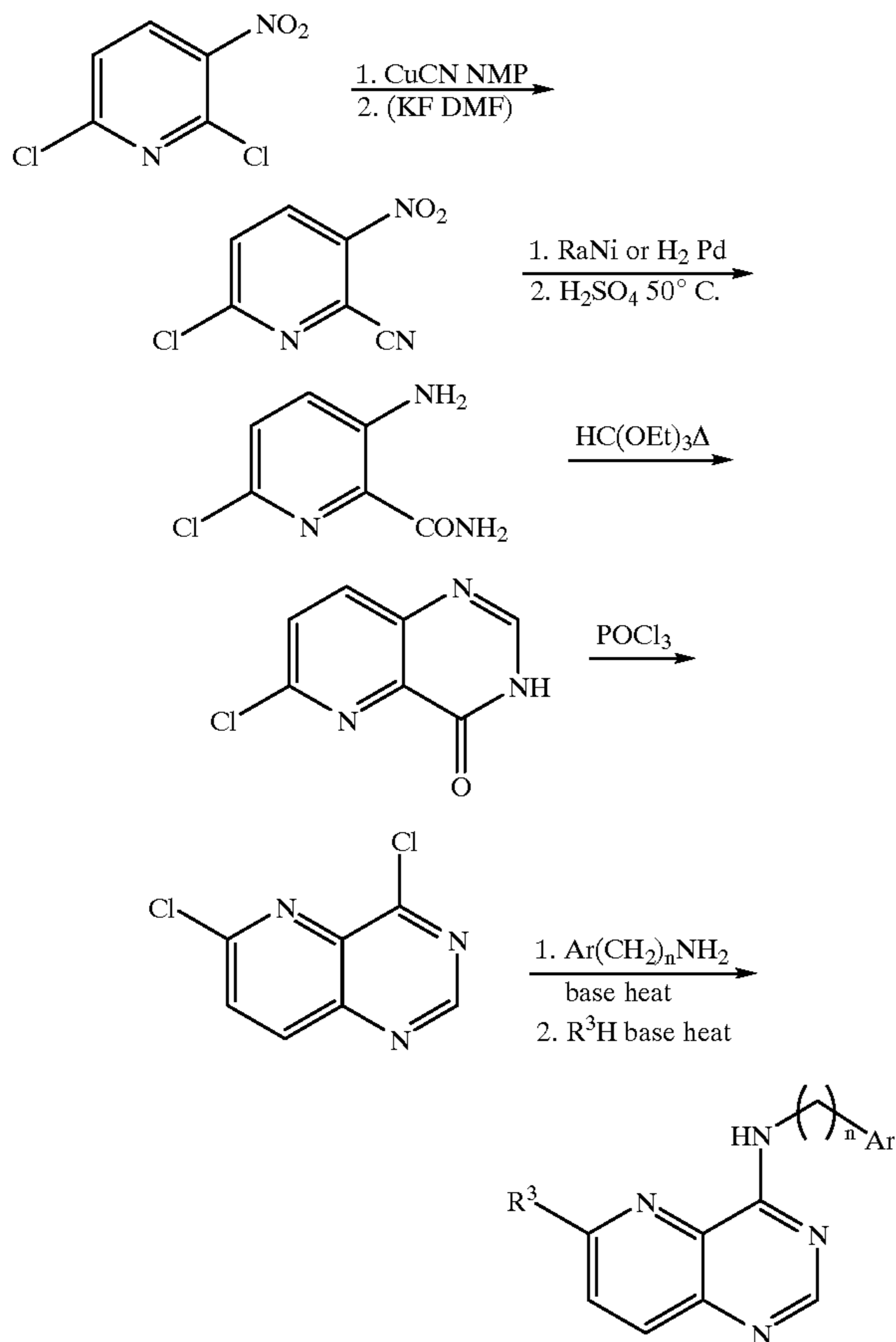
Scheme 1 Synthesis of Preferred Groups 1-5: R 4 = H
