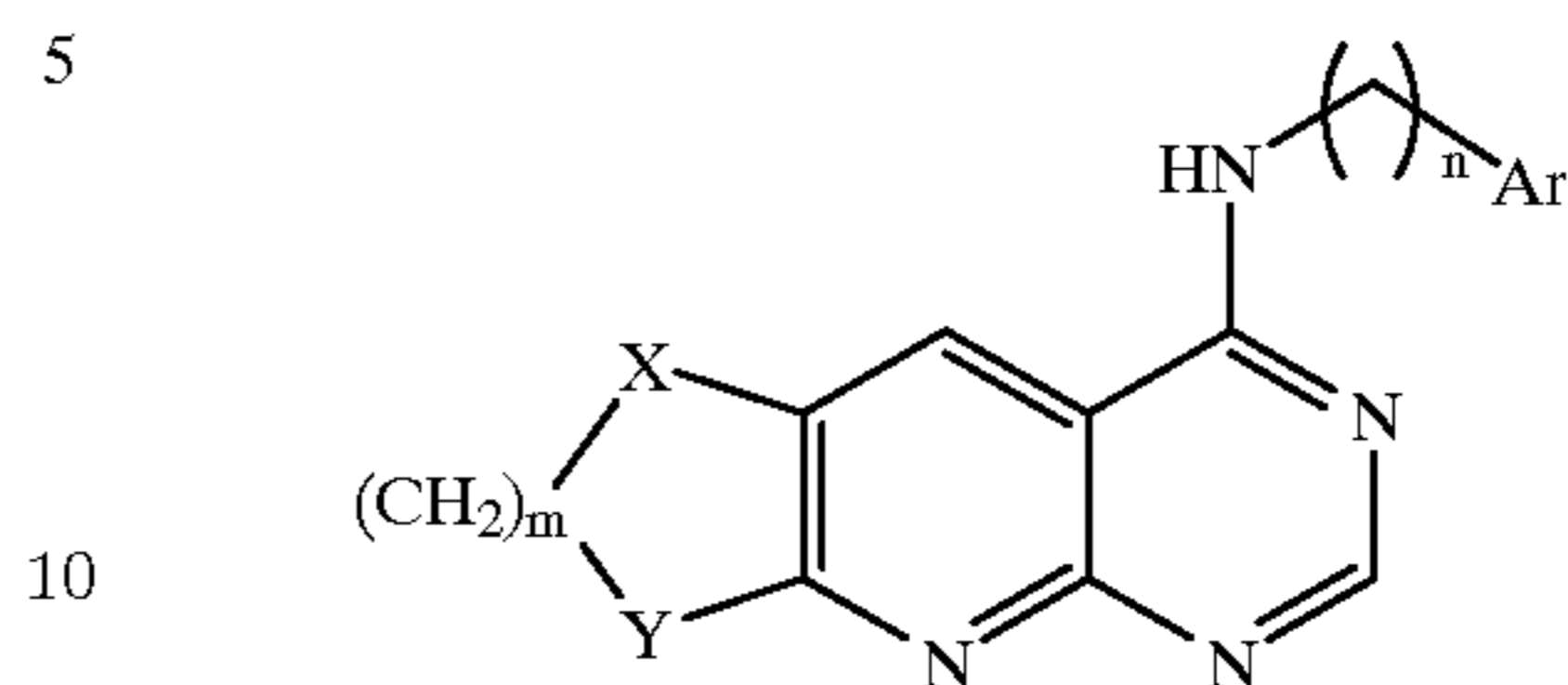
Scheme 14 Preferred Group 32.
