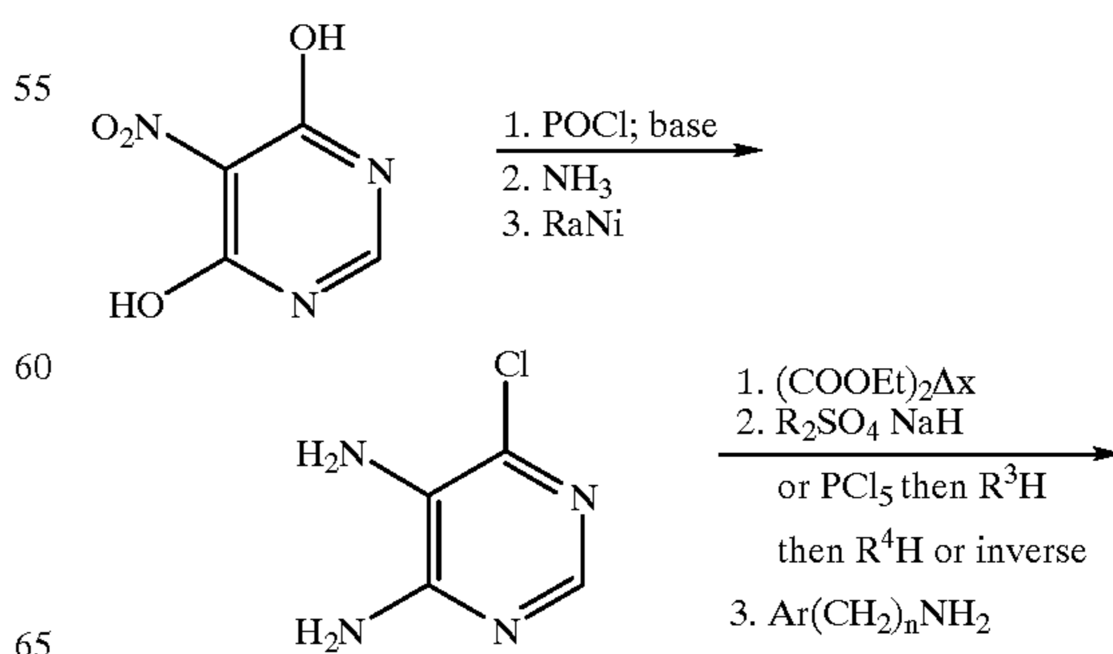
Scheme 16 Synthesis of Preferred Group 37–40
