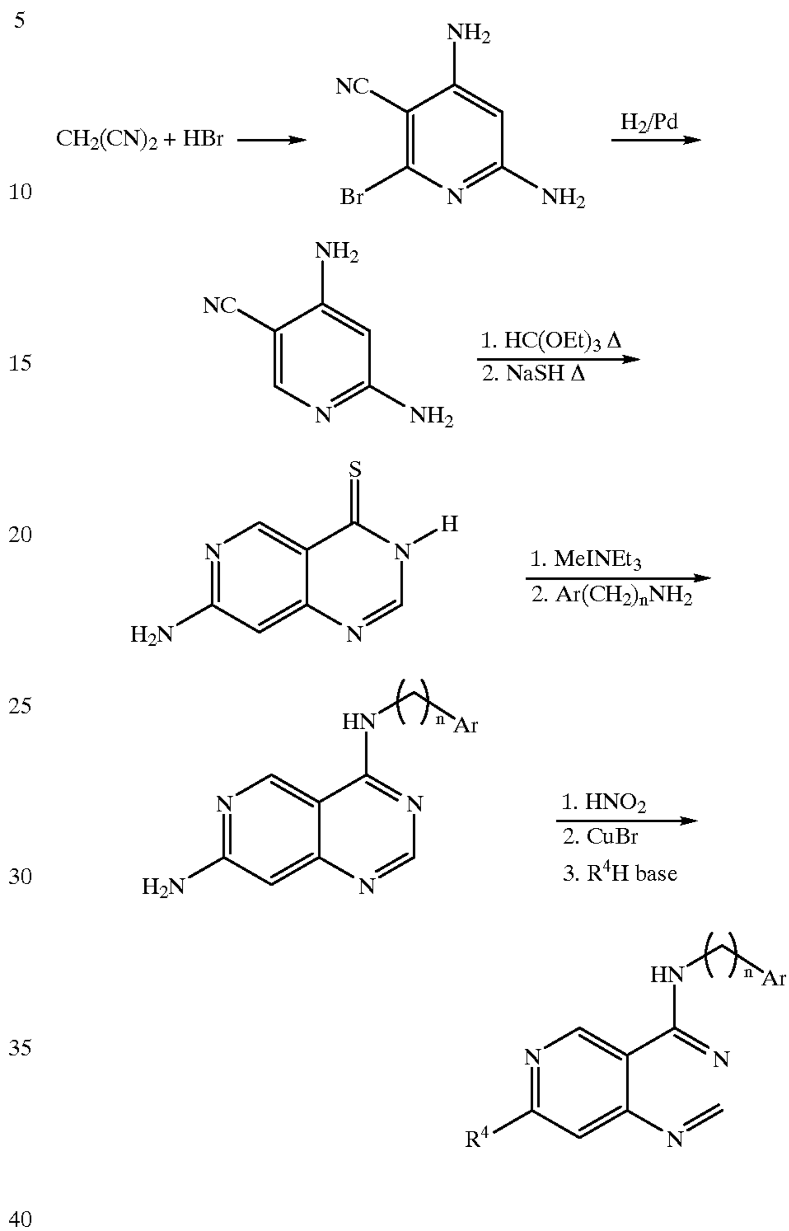
Scheme 8 Synthesis of Preferred Groups 17-21.
