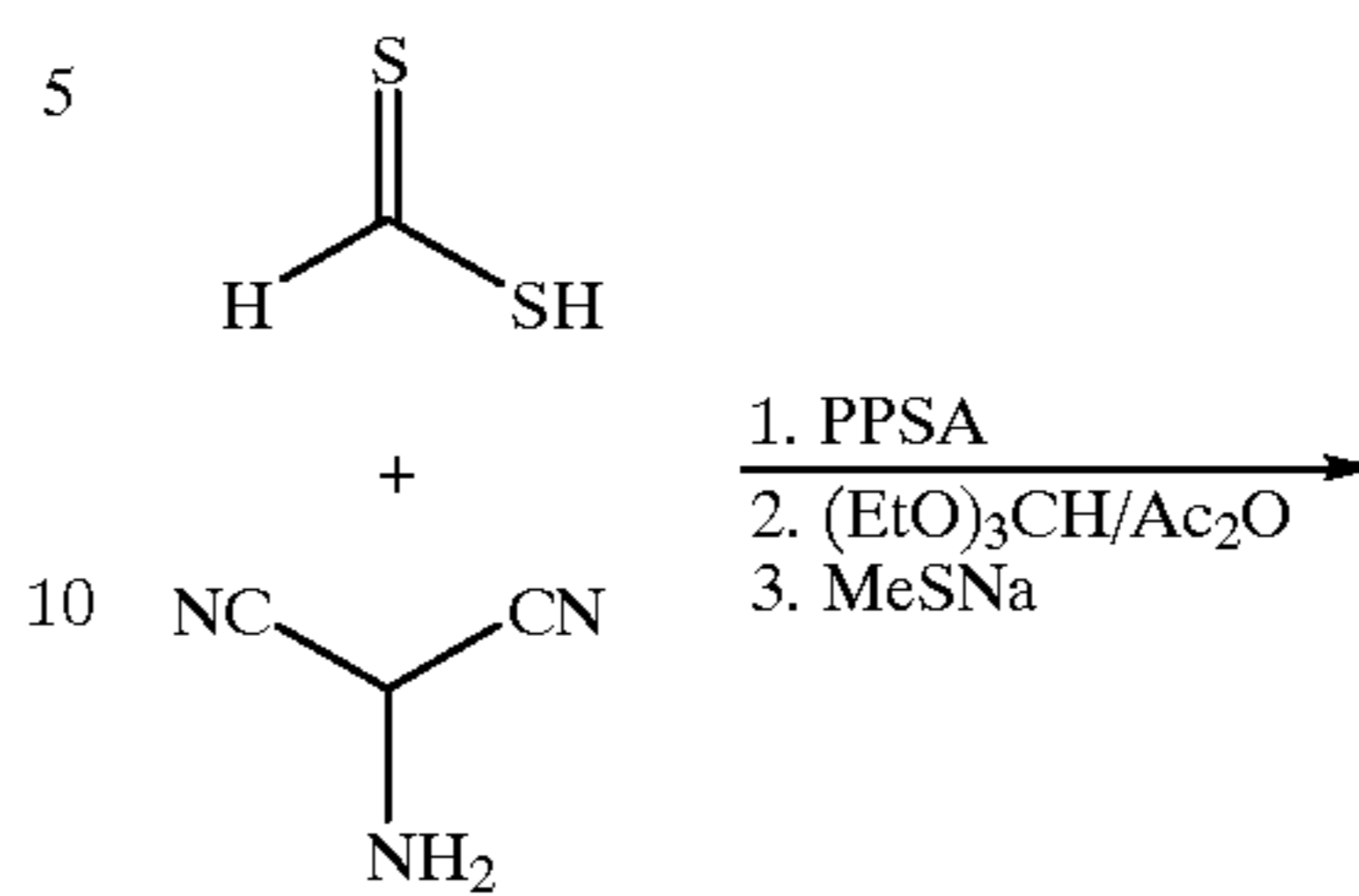
Scheme 23 Synthesis of Preferred Group 44; [5,4-d] ring fusion
