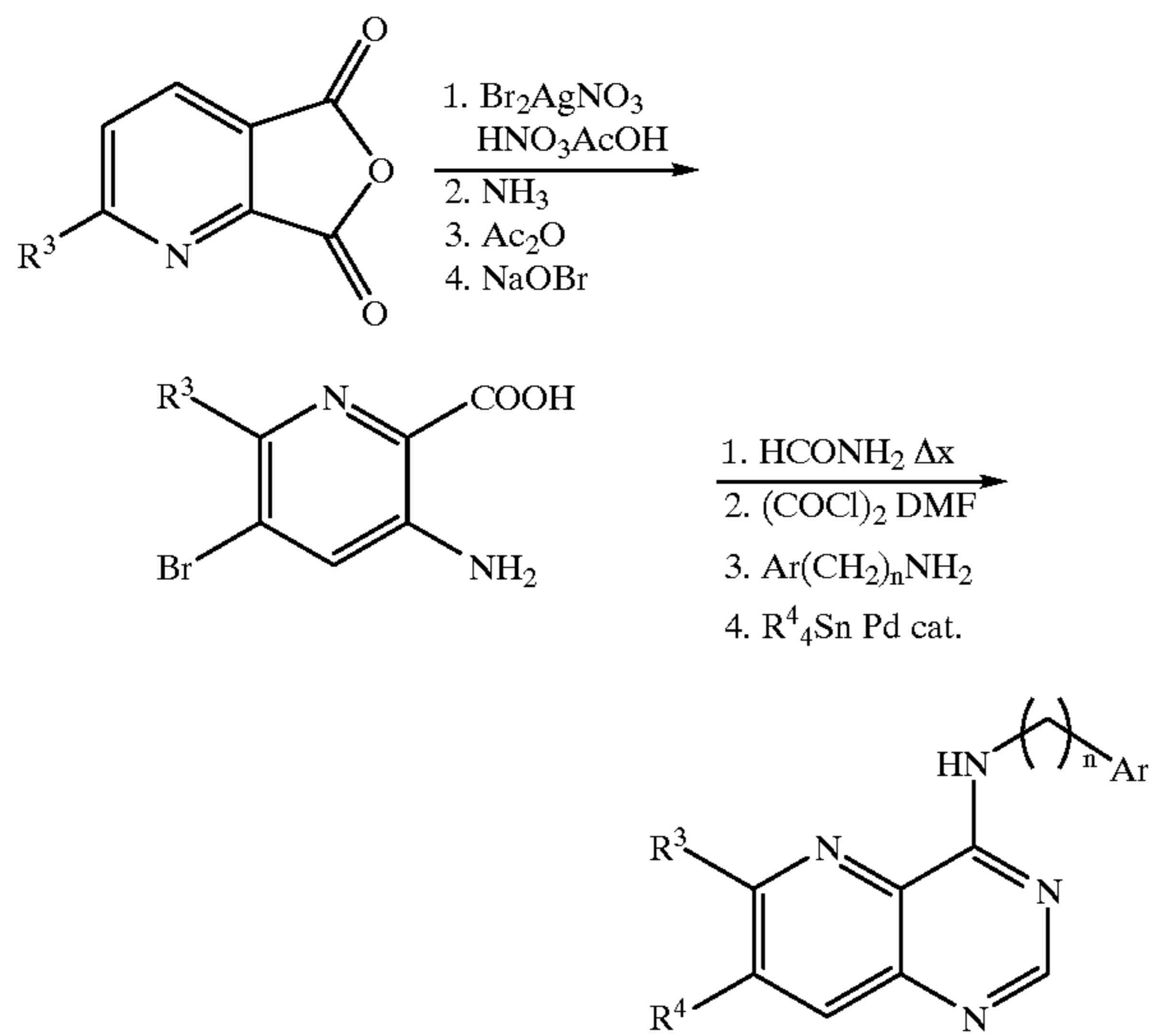
Scheme 4 Synthesis of Preferred Group 7.
