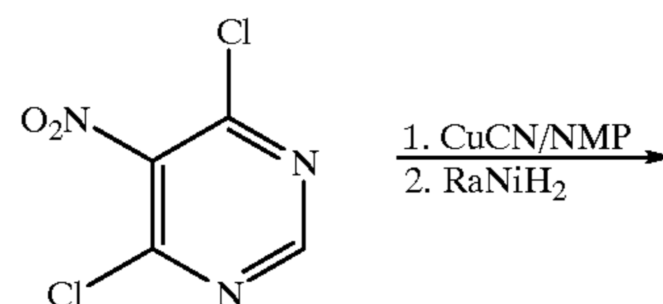
Scheme 29 Synthesis of Preferred Group 47; [4,5-d] ring fusion.
