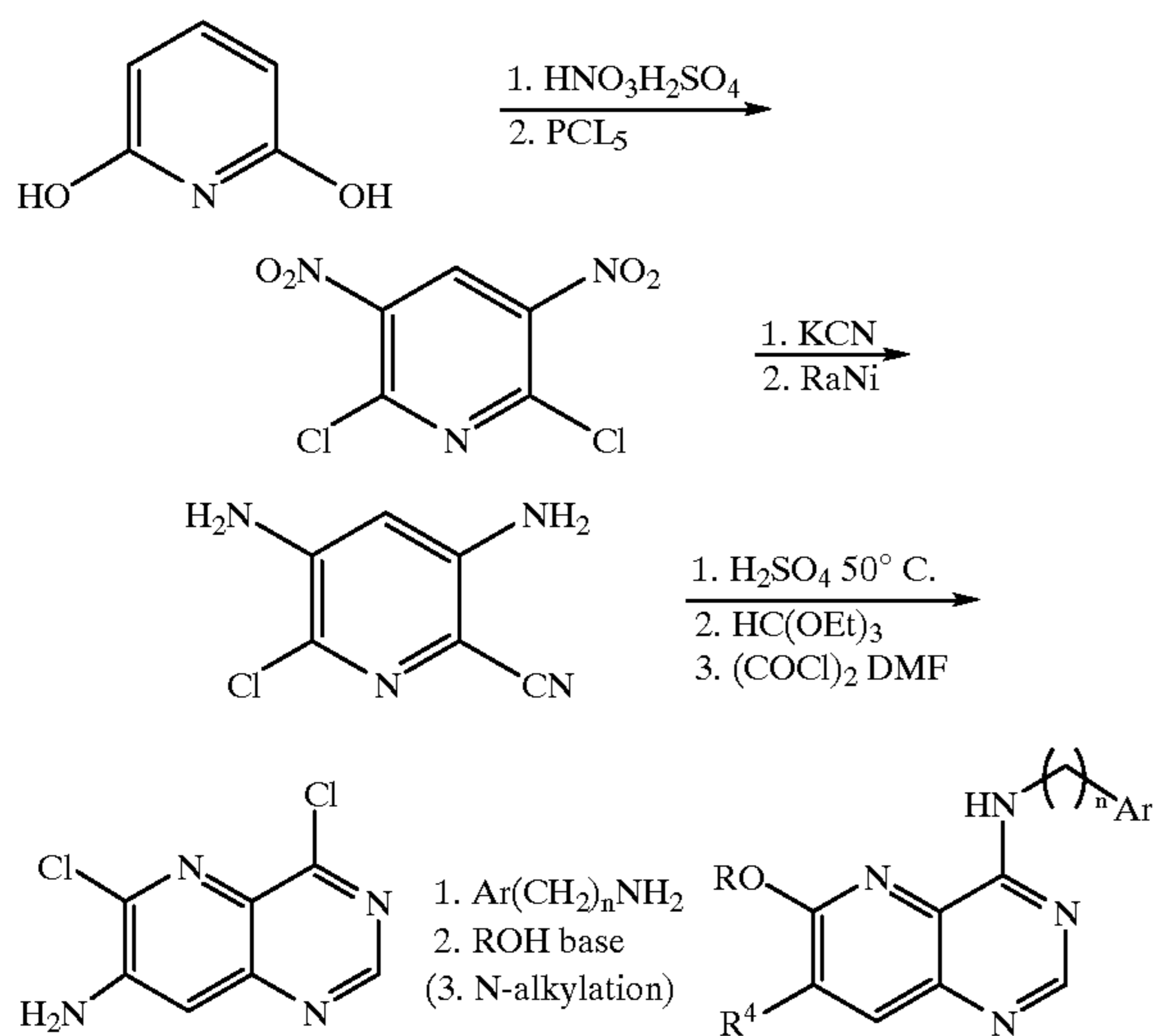
Scheme 5 Synthesis of Preferred Groups 8 & 9: \text{R}^3 = \text{OR.}
