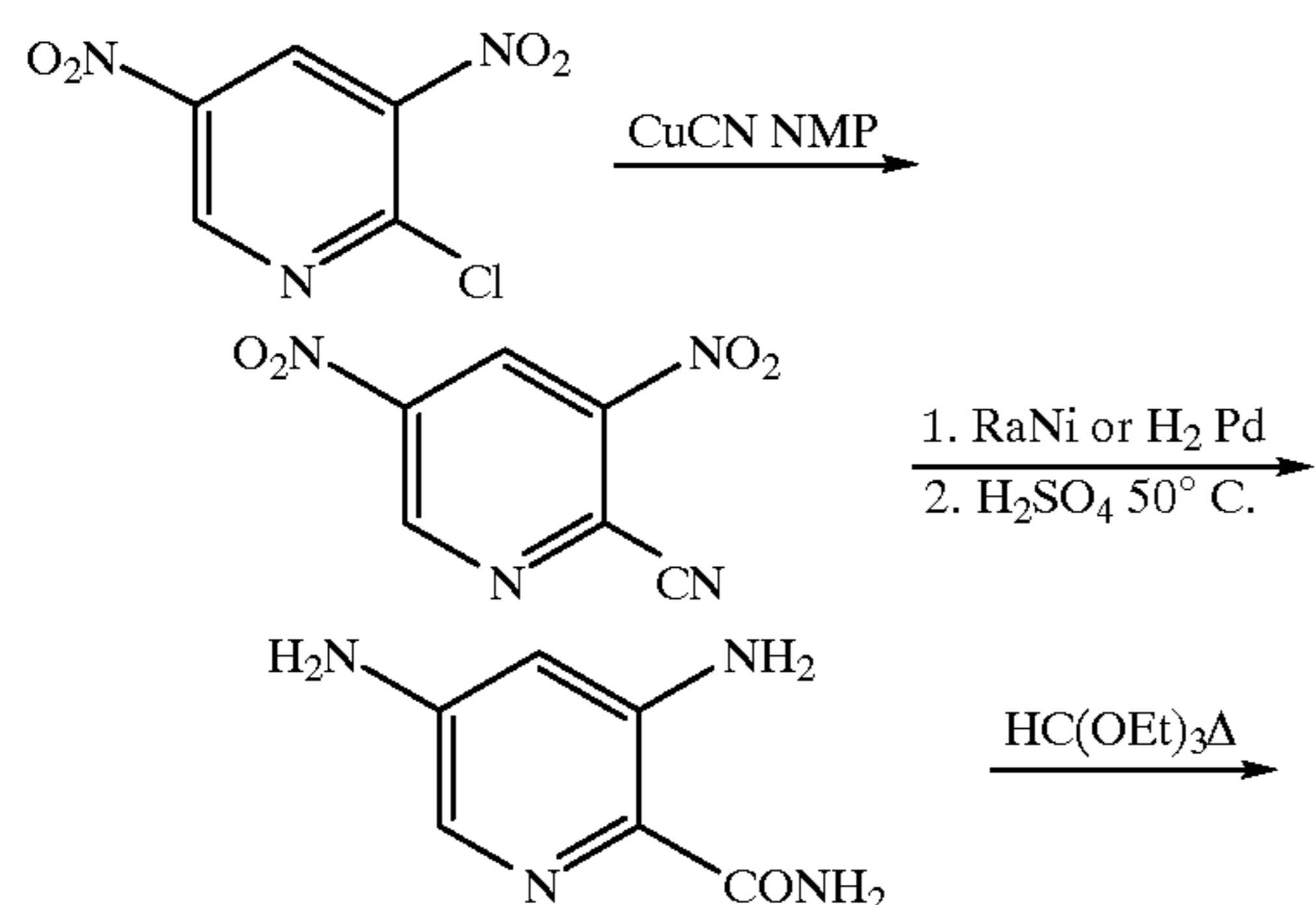
Scheme 2 Synthesis of Preferred Groups 1-5: R 3 = H
