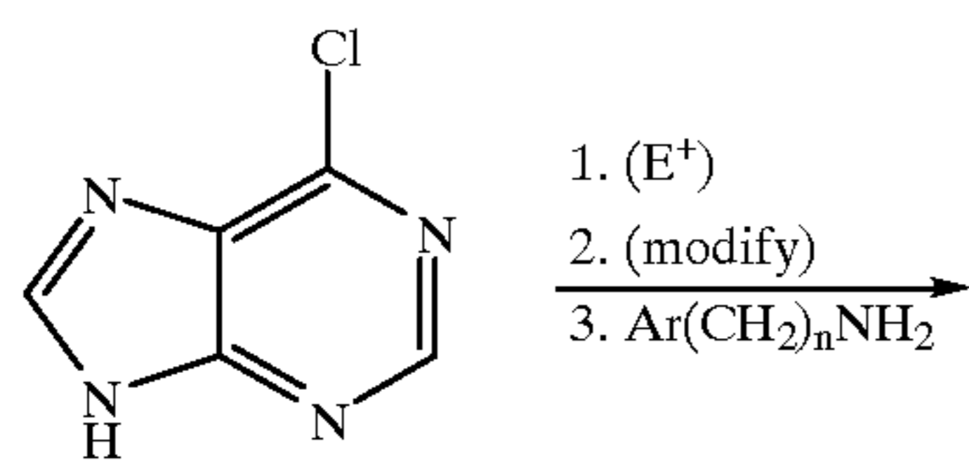
Scheme 27 Synthesis of Preferred Group 46
