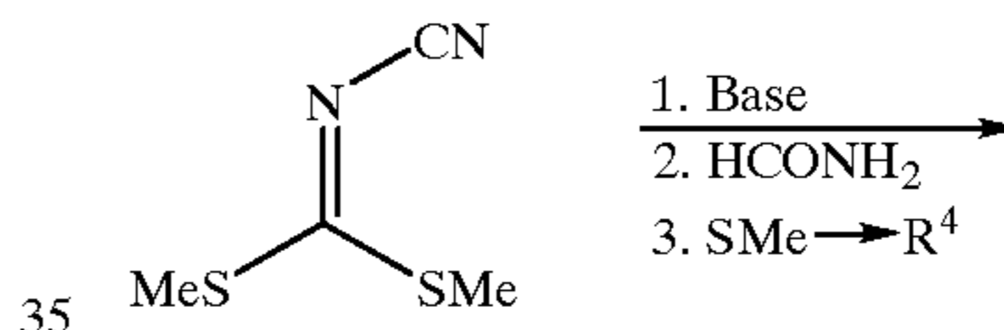
Scheme 24 Synthesis of Preferred Group 44; [4,5-d] ring fusion
