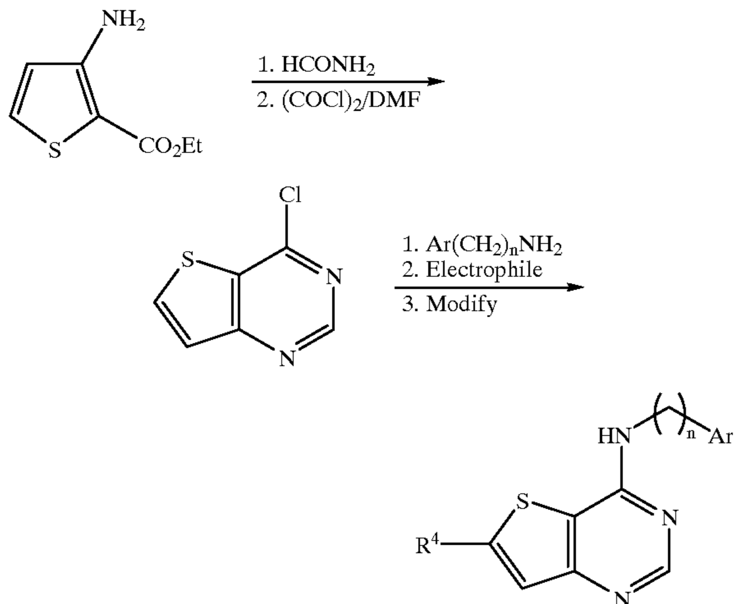
Scheme 17 Synthesis of Preferred Group 41; [3,2-d] ring fusion
