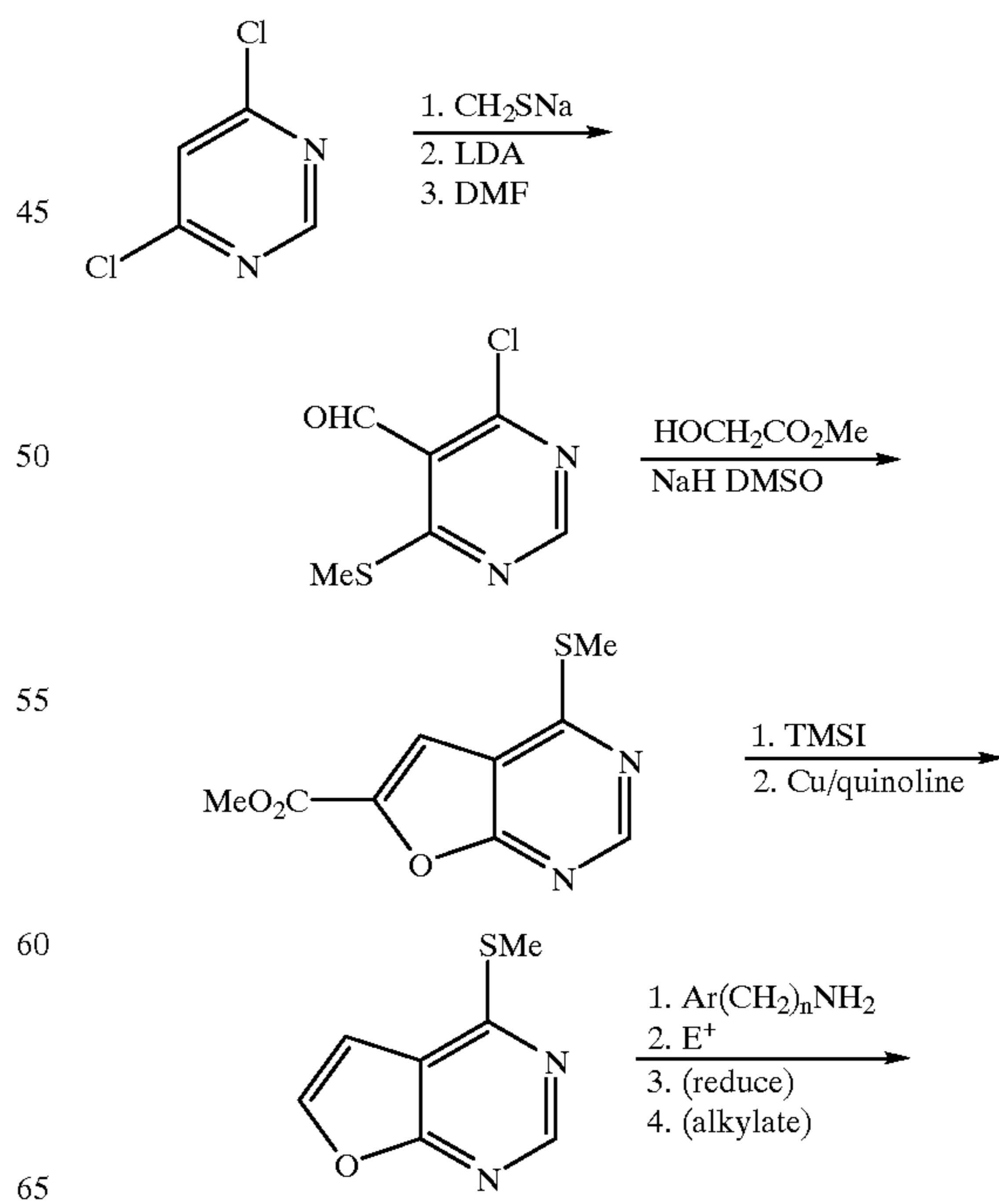
Scheme 20 Synthesis of Preferred Group 42; [2,3-d] ring fusion
