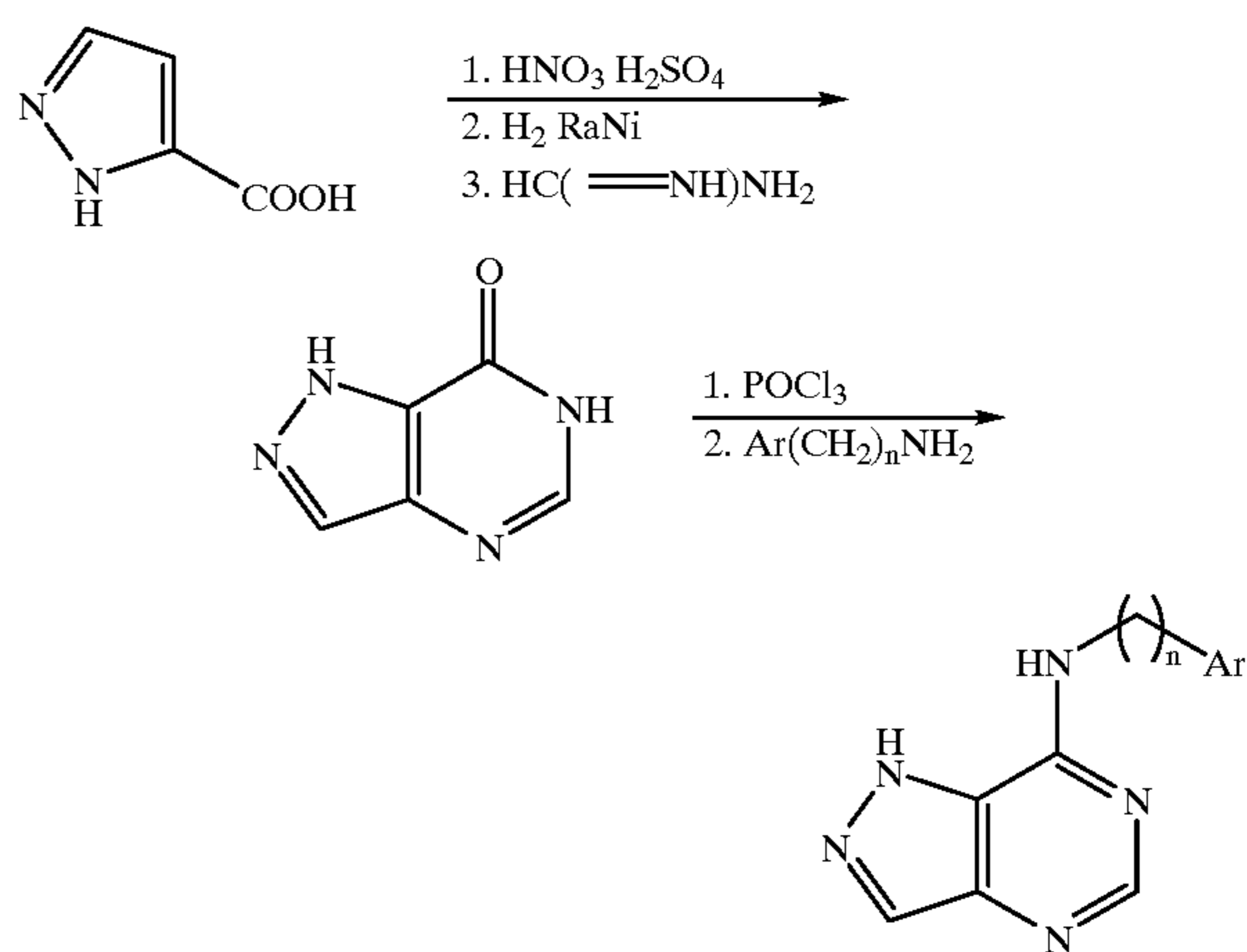
Scheme 33 Synthesis of Preferred Group 49; [4,3-d] ring fusion
