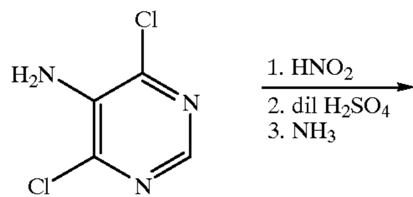
Scheme 26 Synthesis of Preferred Group 45; [4,5-d] ring fusion
