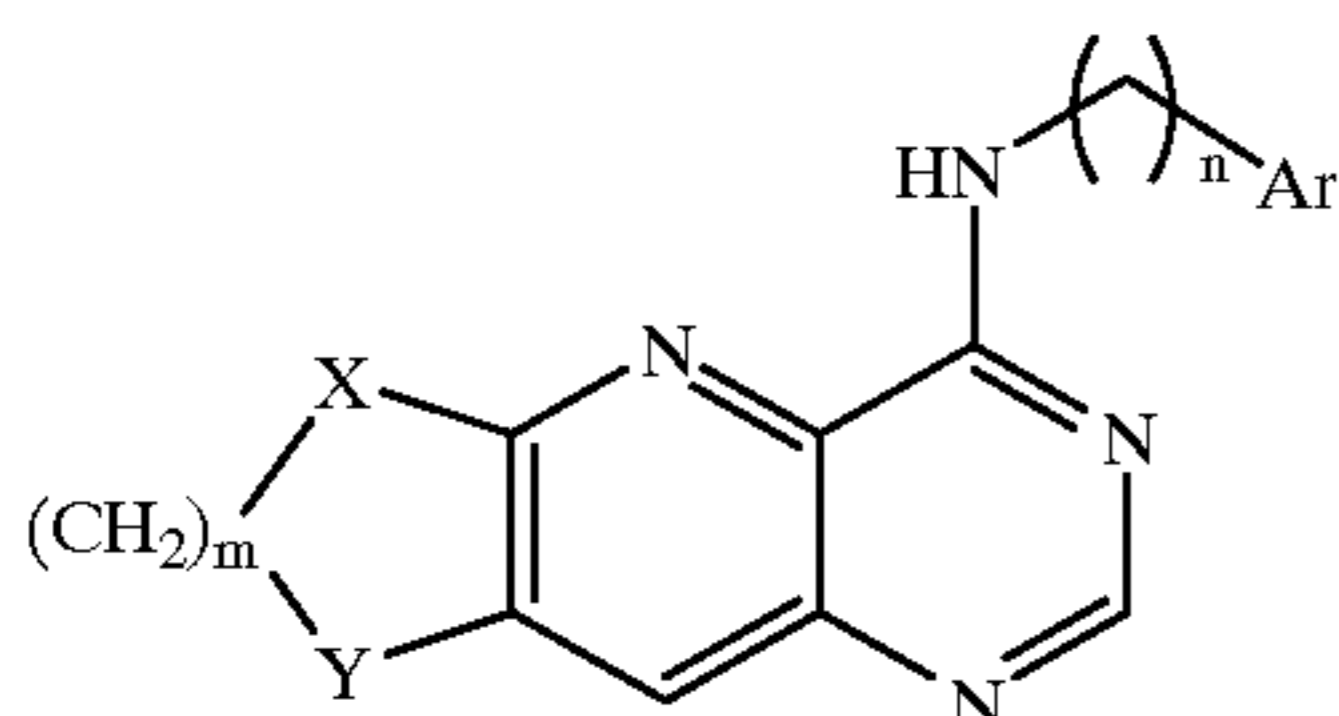
Scheme 6 Preferred Group 11.
