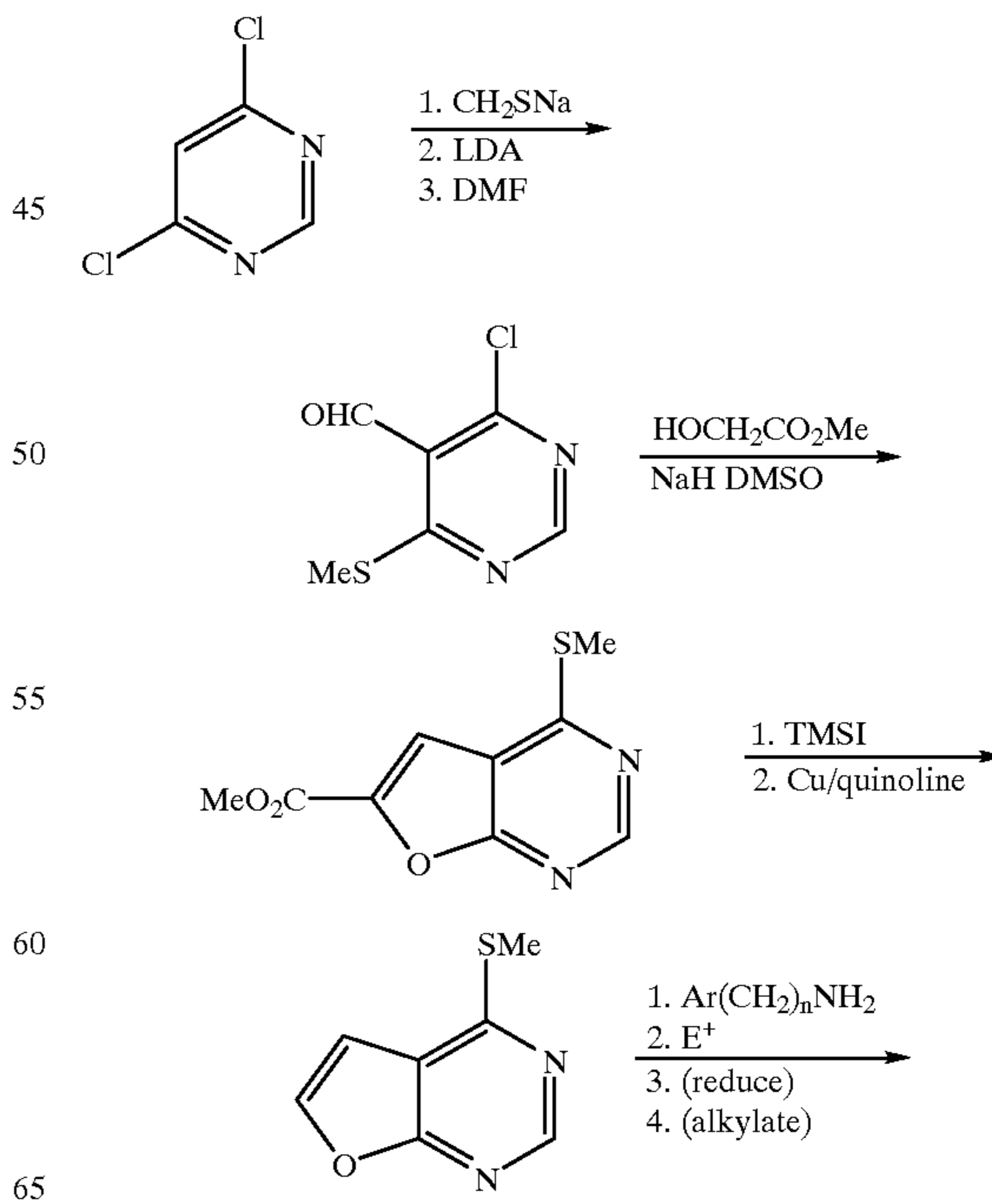
Scheme 20 Synthesis of Preferred Group 42; [2,3-d] ring fusion
