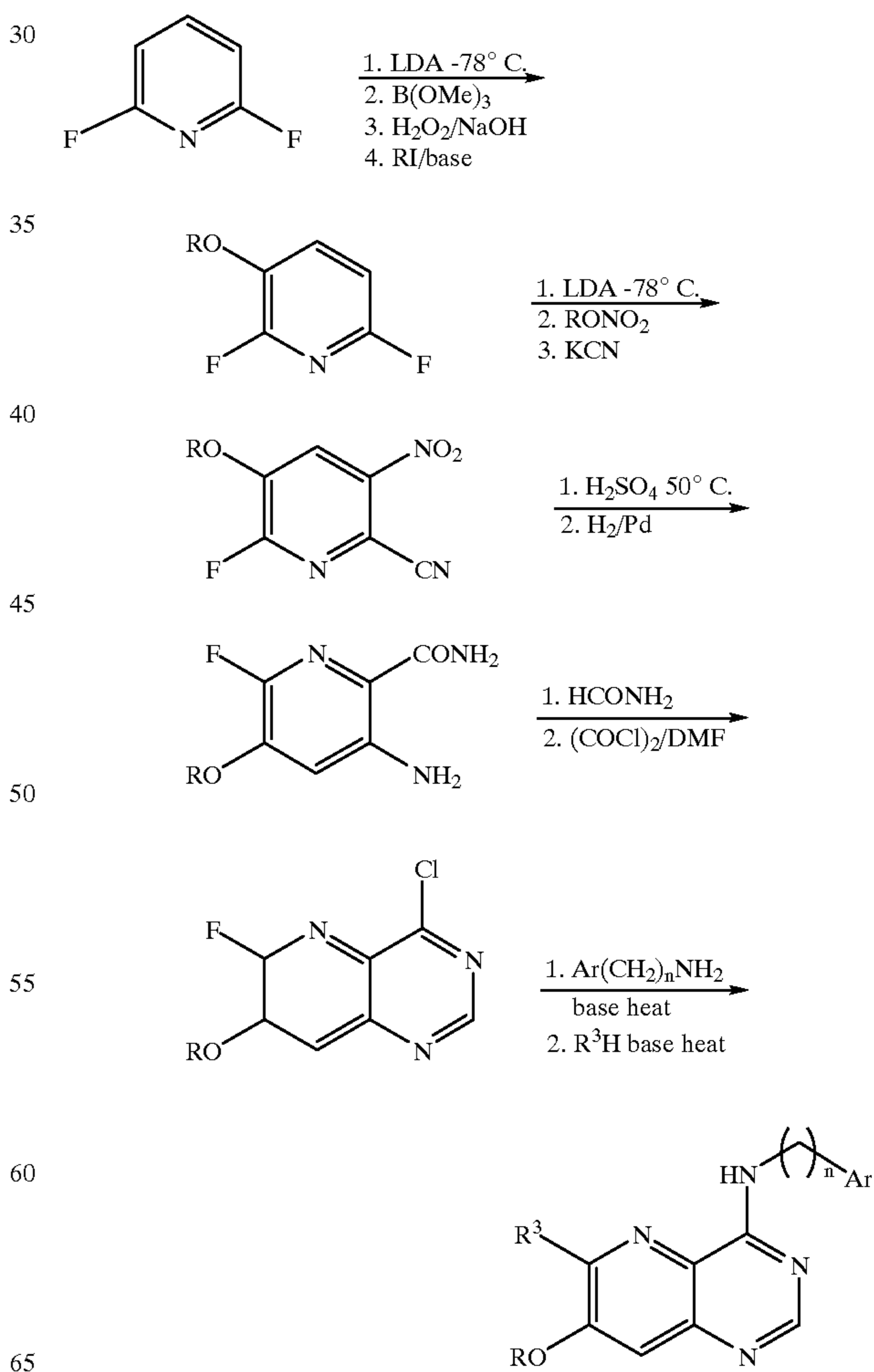
Scheme 3 Synthesis of Preferred Groups 6 and 8-10: R 4 = RO
