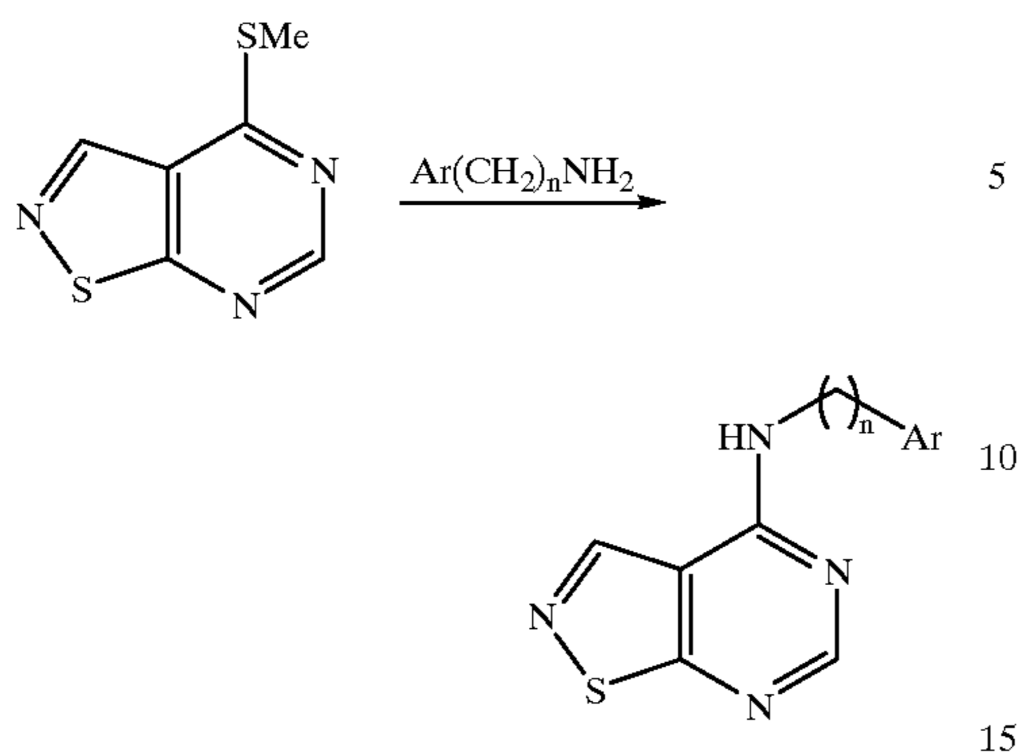
Scheme 31 Synthesis of Preferred Group 48; [4, 5-d] ring fusion.
