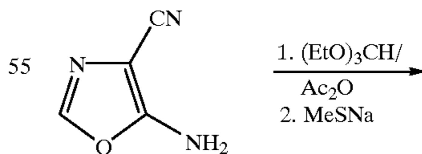
Scheme 25 Synthesis of Preferred Group 45; [5,4-d] ring fusion
