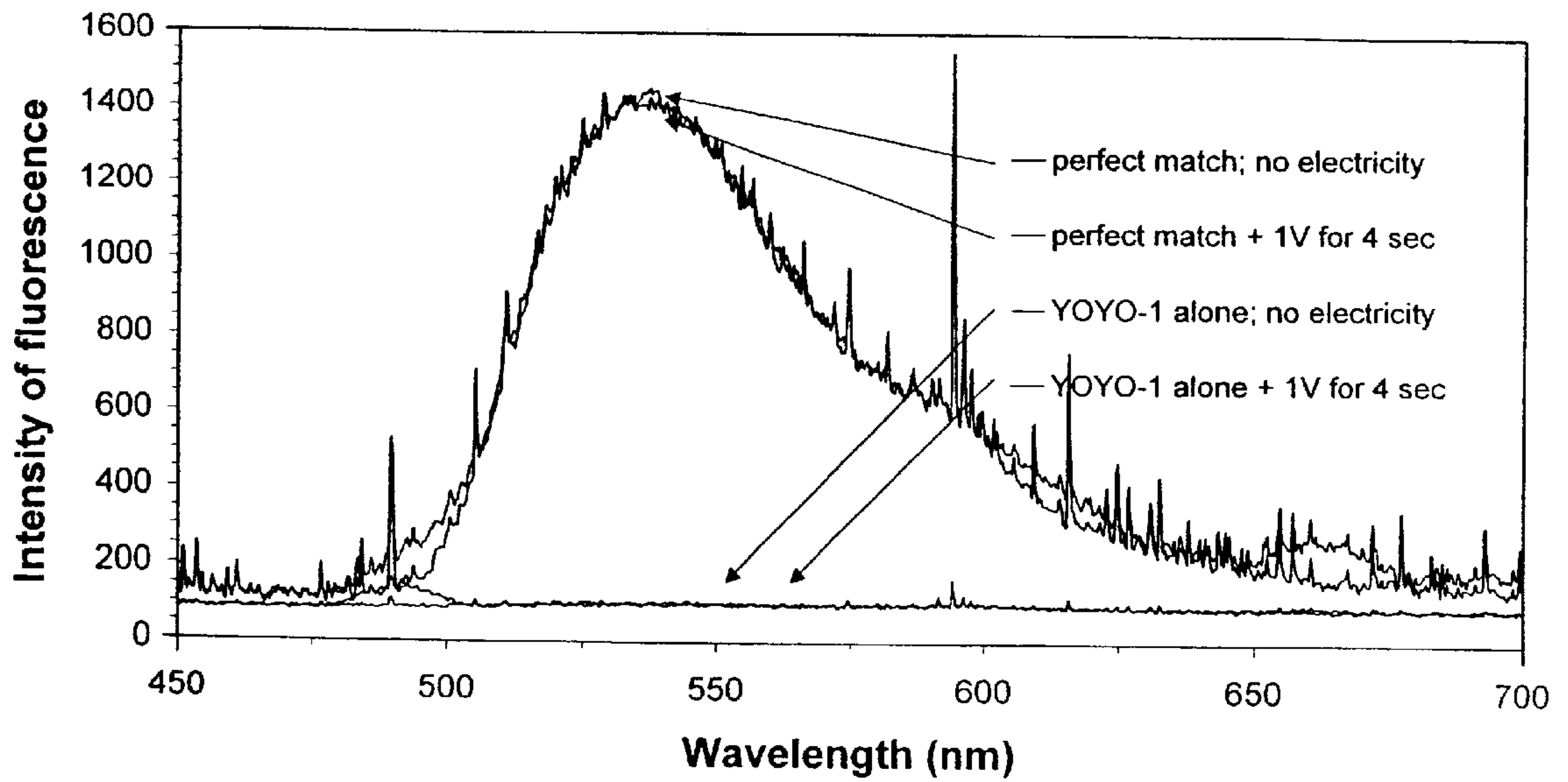
Figure 5B (PNA:DNA 1bp mismatch; 65°C)
