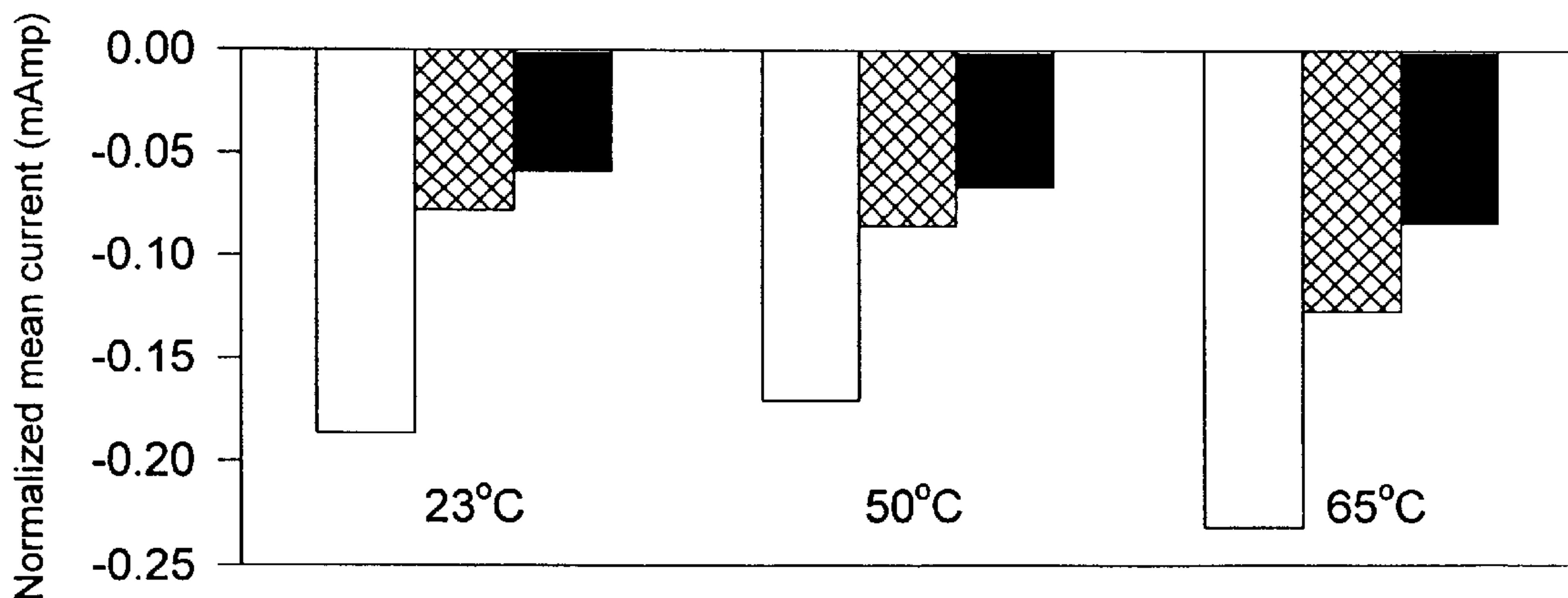
Figure 2C (5V; parallel PNA probe; 65°C treatment)
