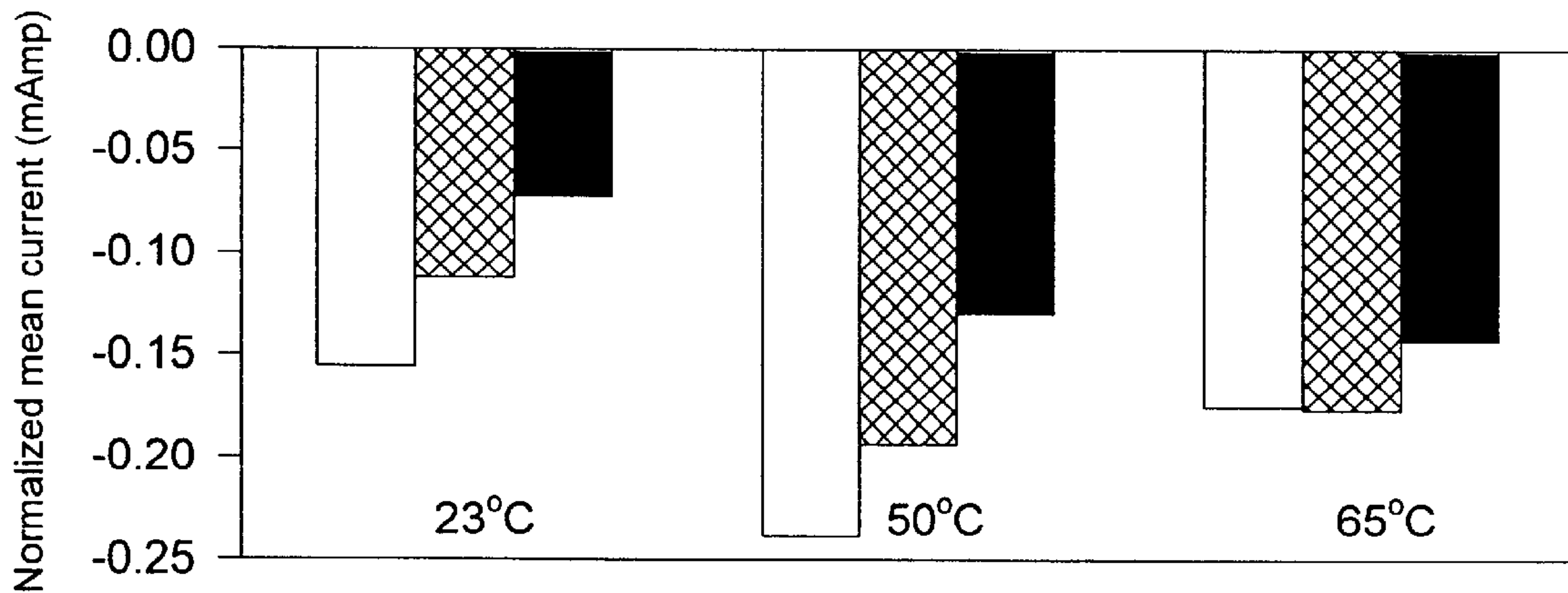
Figure 2B (5V; parallel PNA probe)
