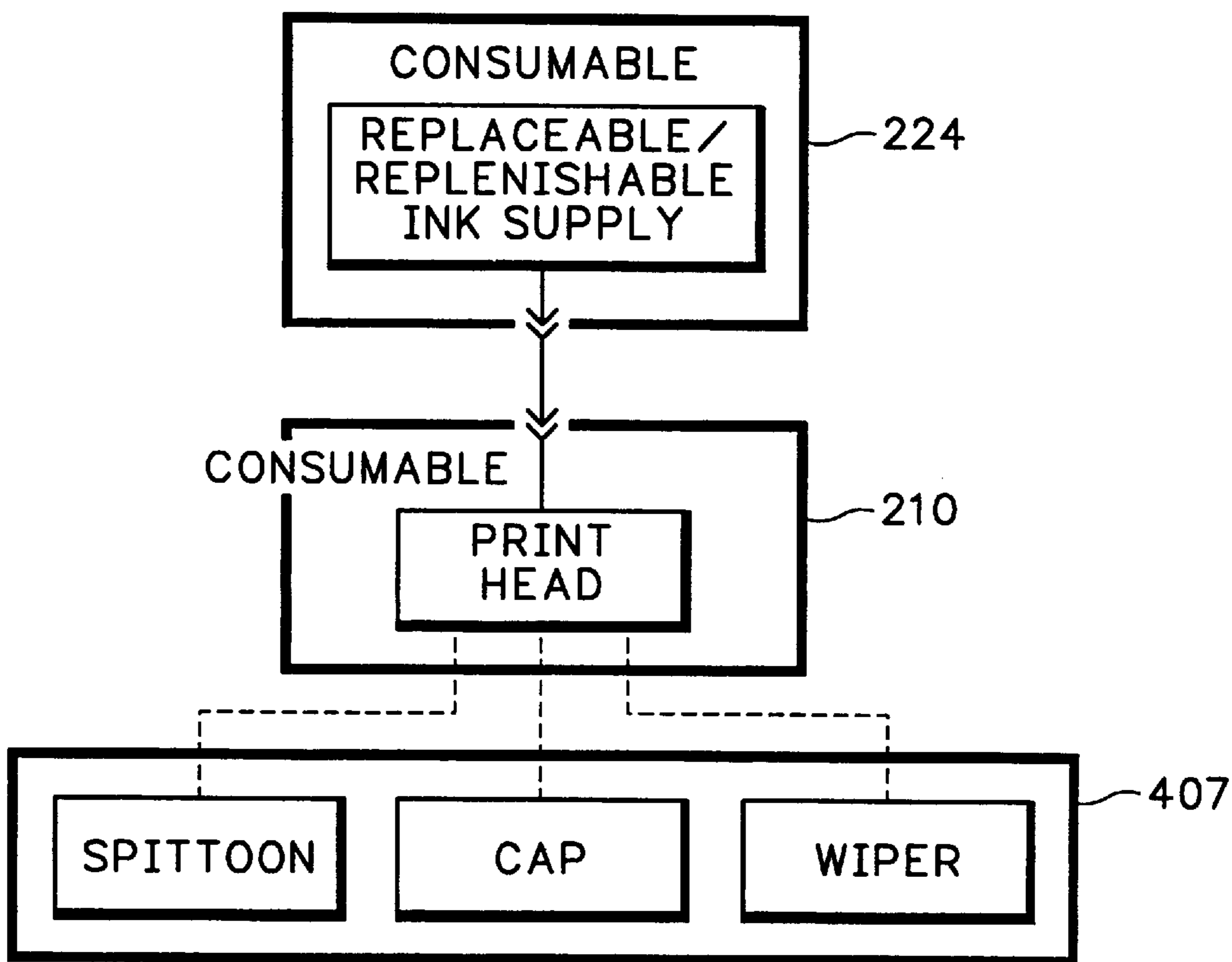
FIG.9 (PRIOR ART)
