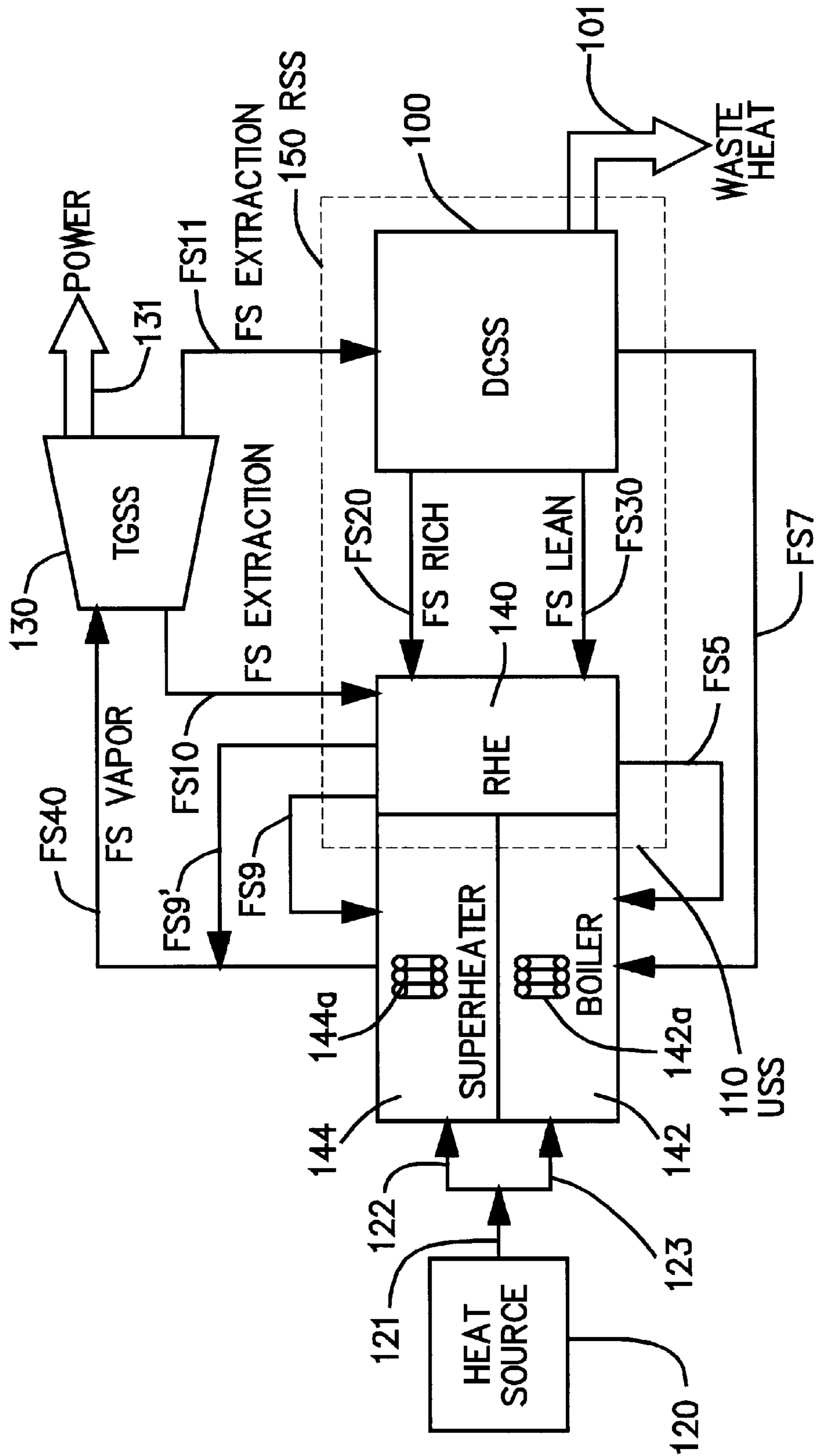
Figure 1 (PRIOR ART)
