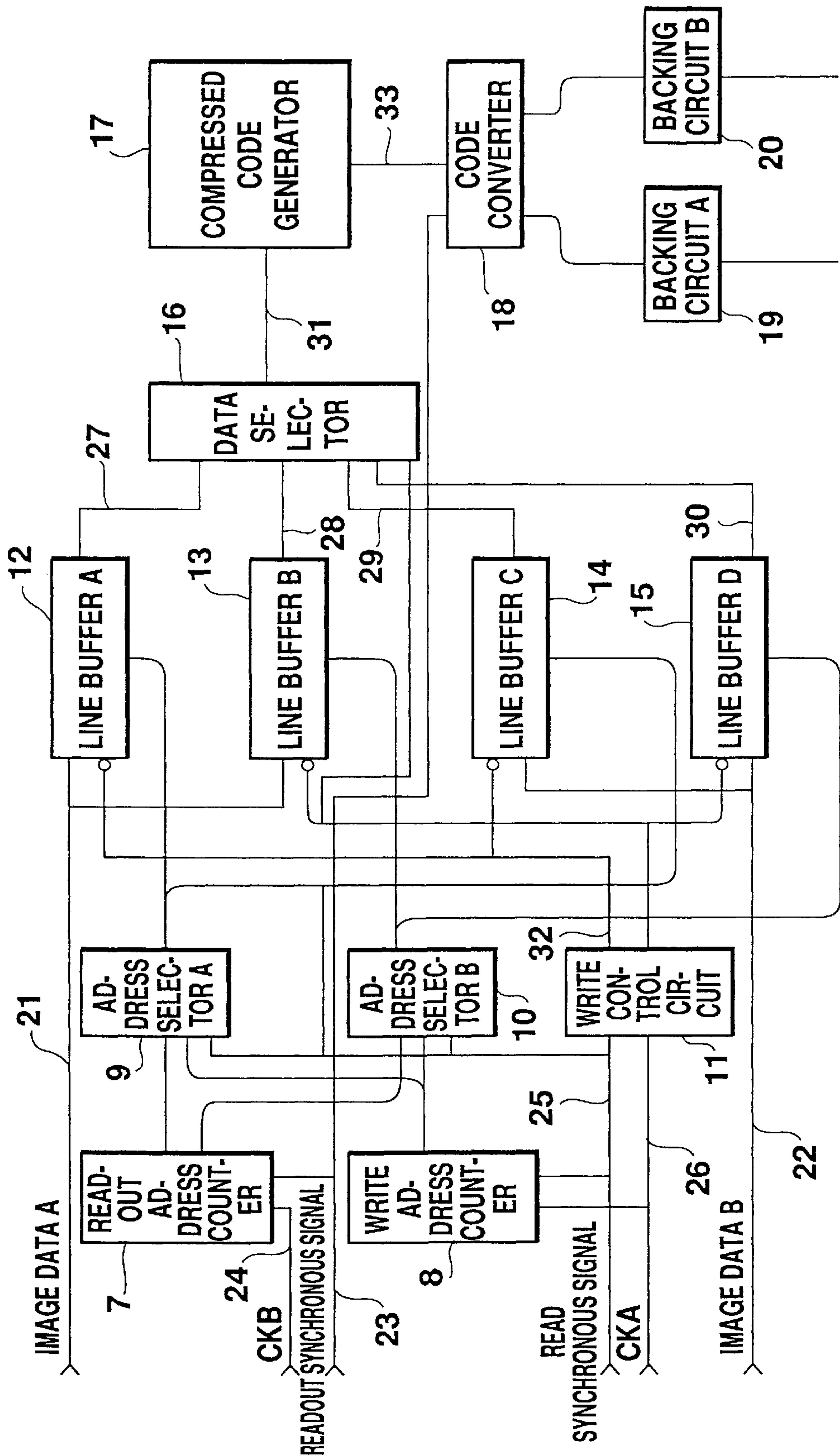
Fig. 20 PRIOR ART
