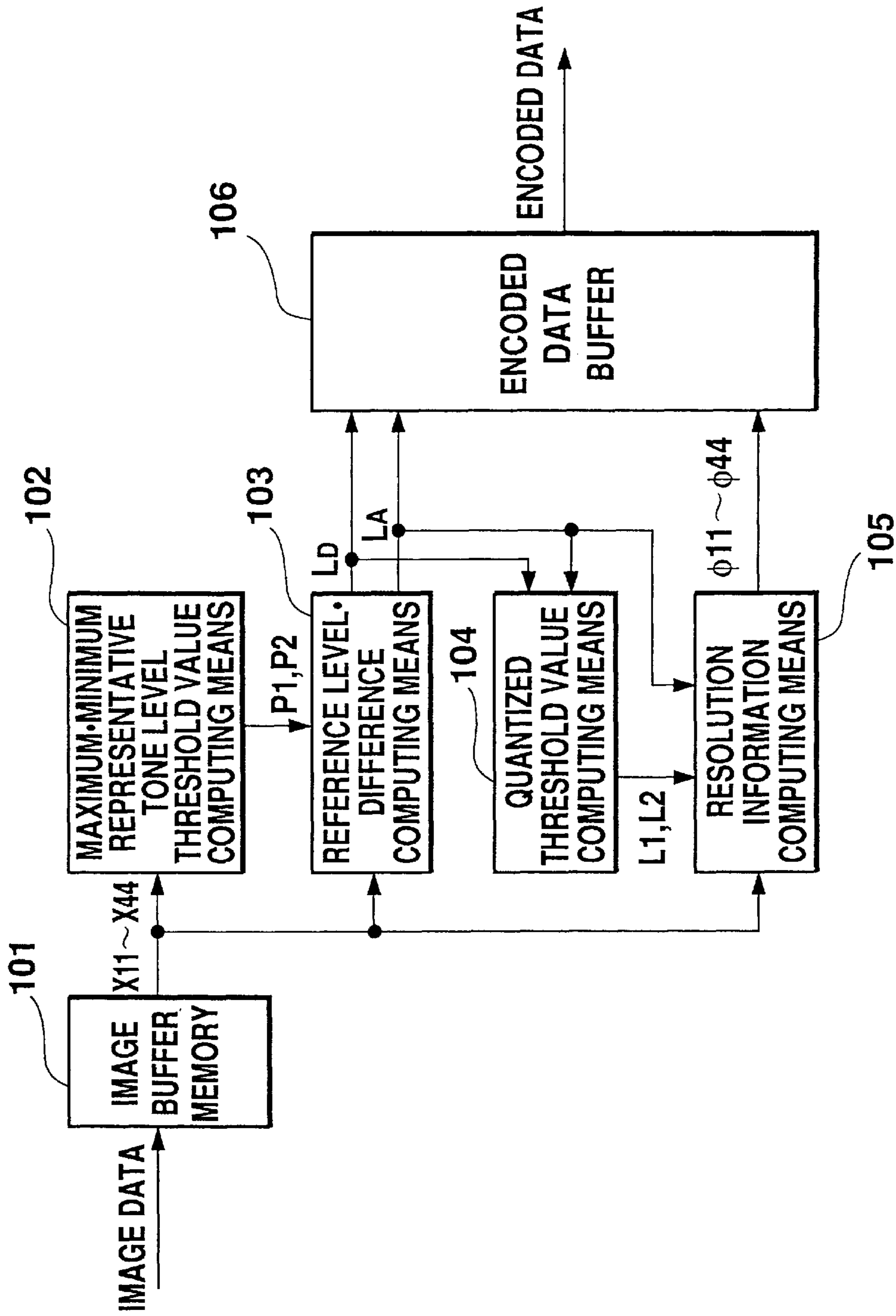
Fig. 22 PRIOR ART
