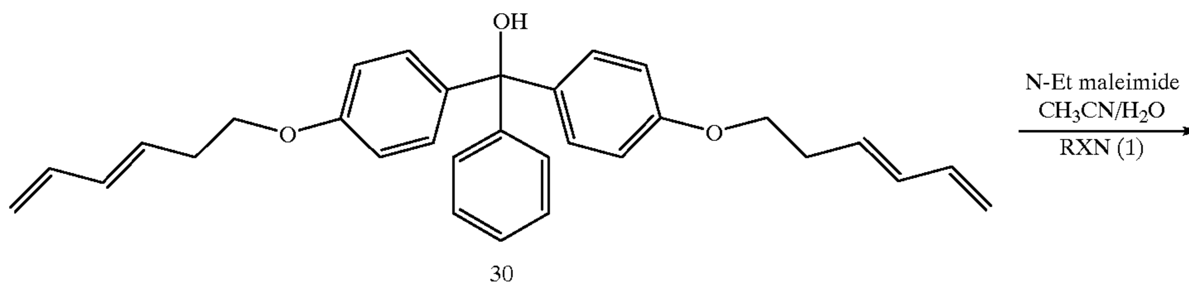
SCHEME 9
