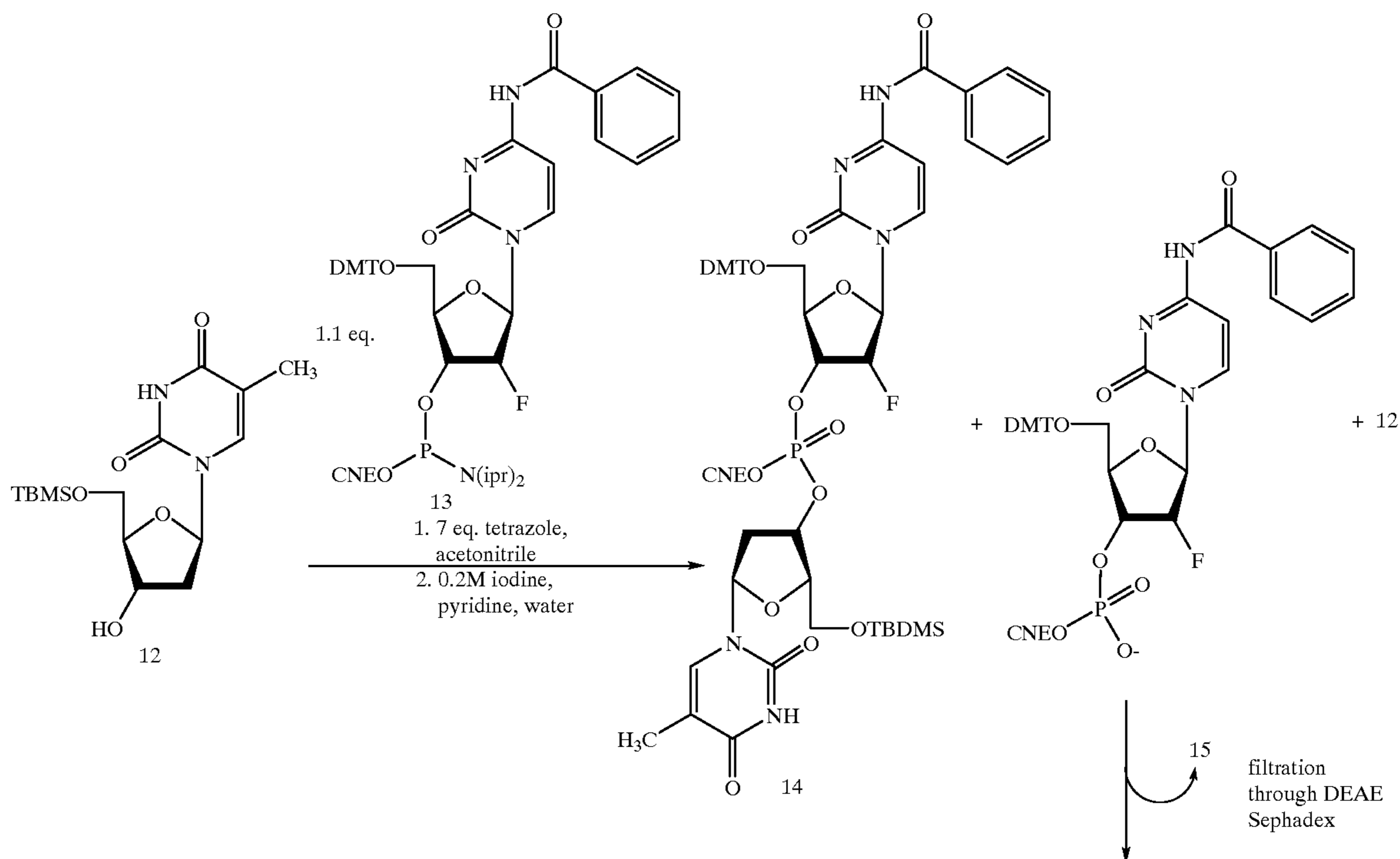
SCHEME 4
