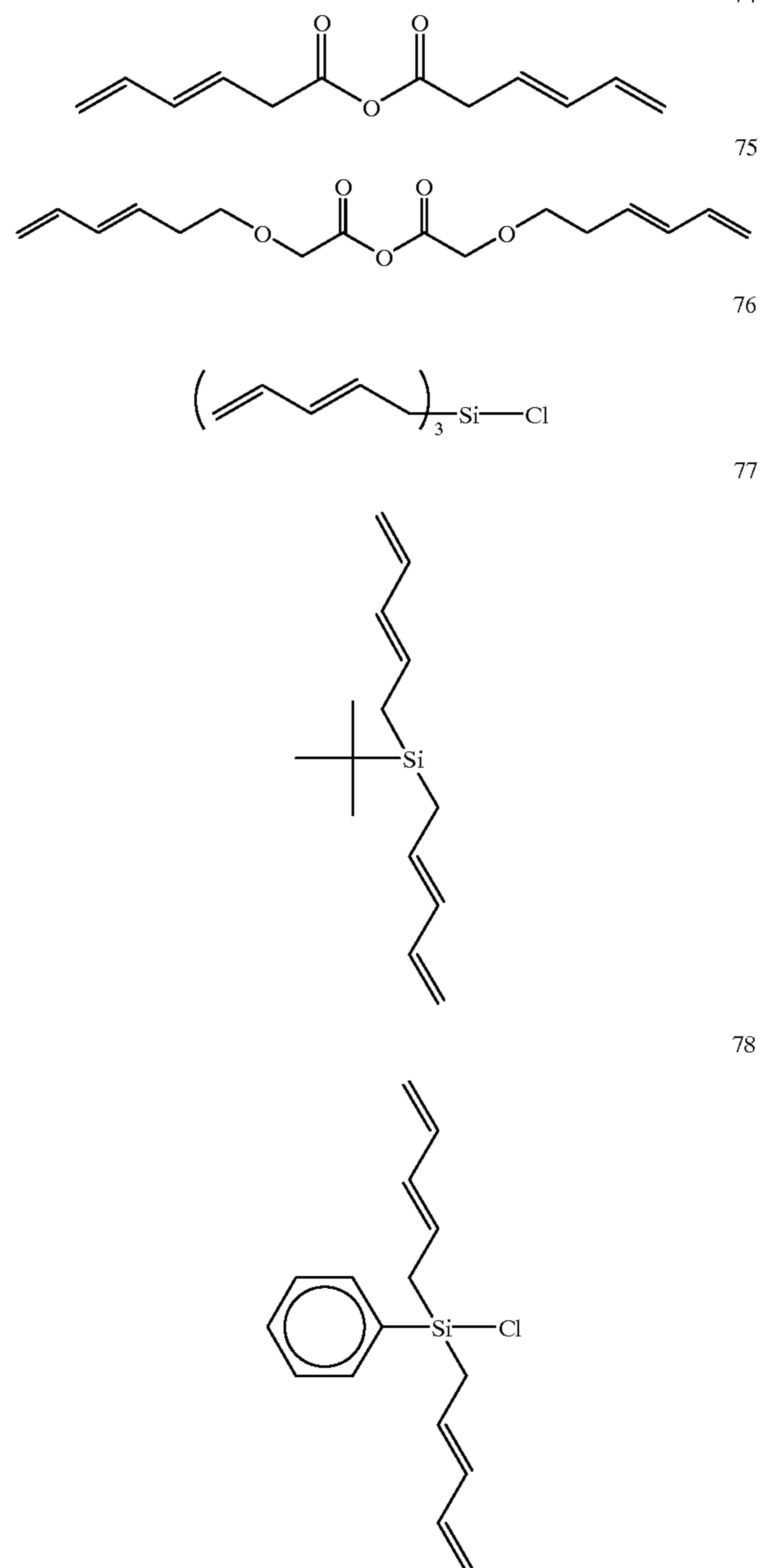
SCHEME 18
