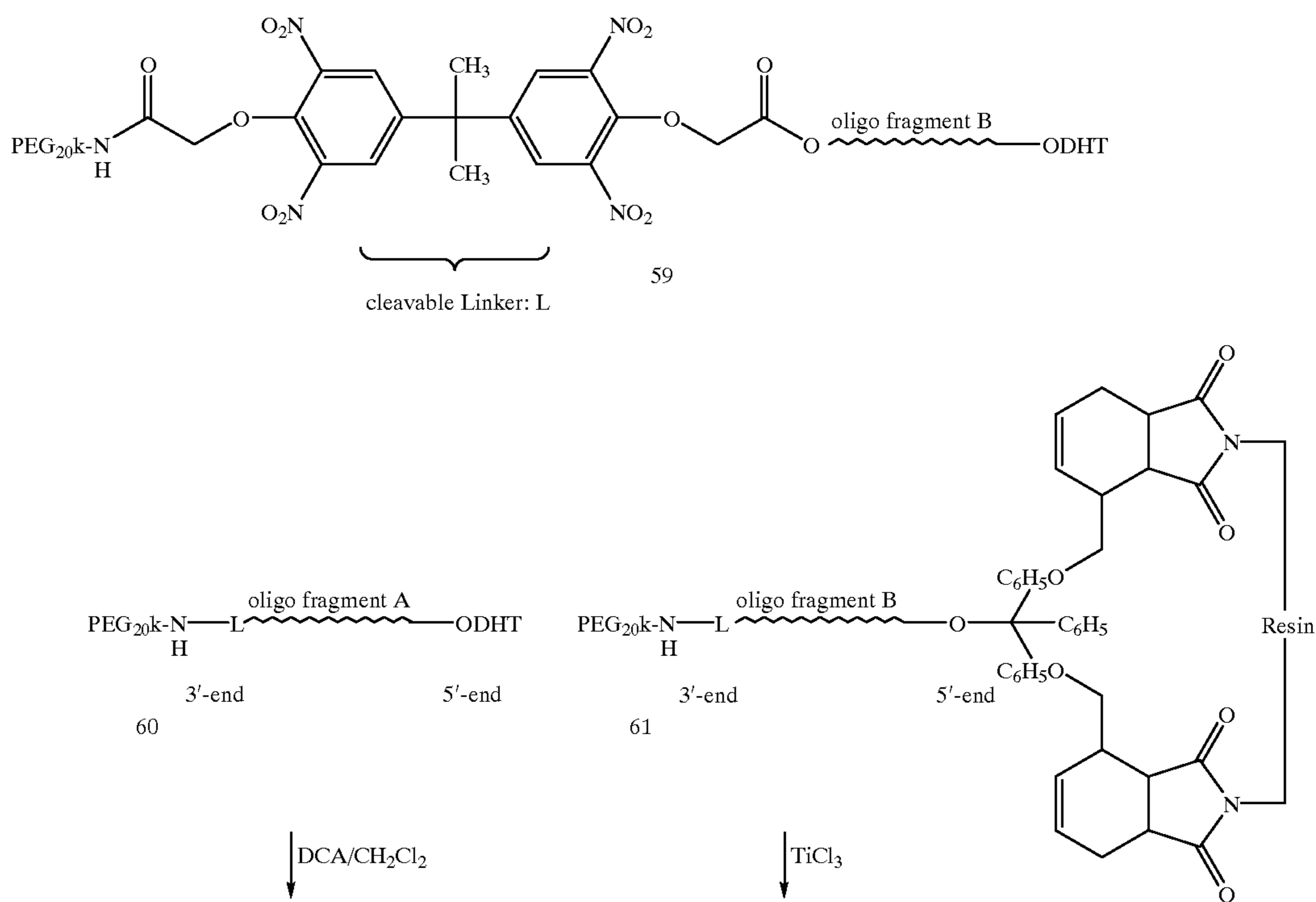
SCHEME 16
