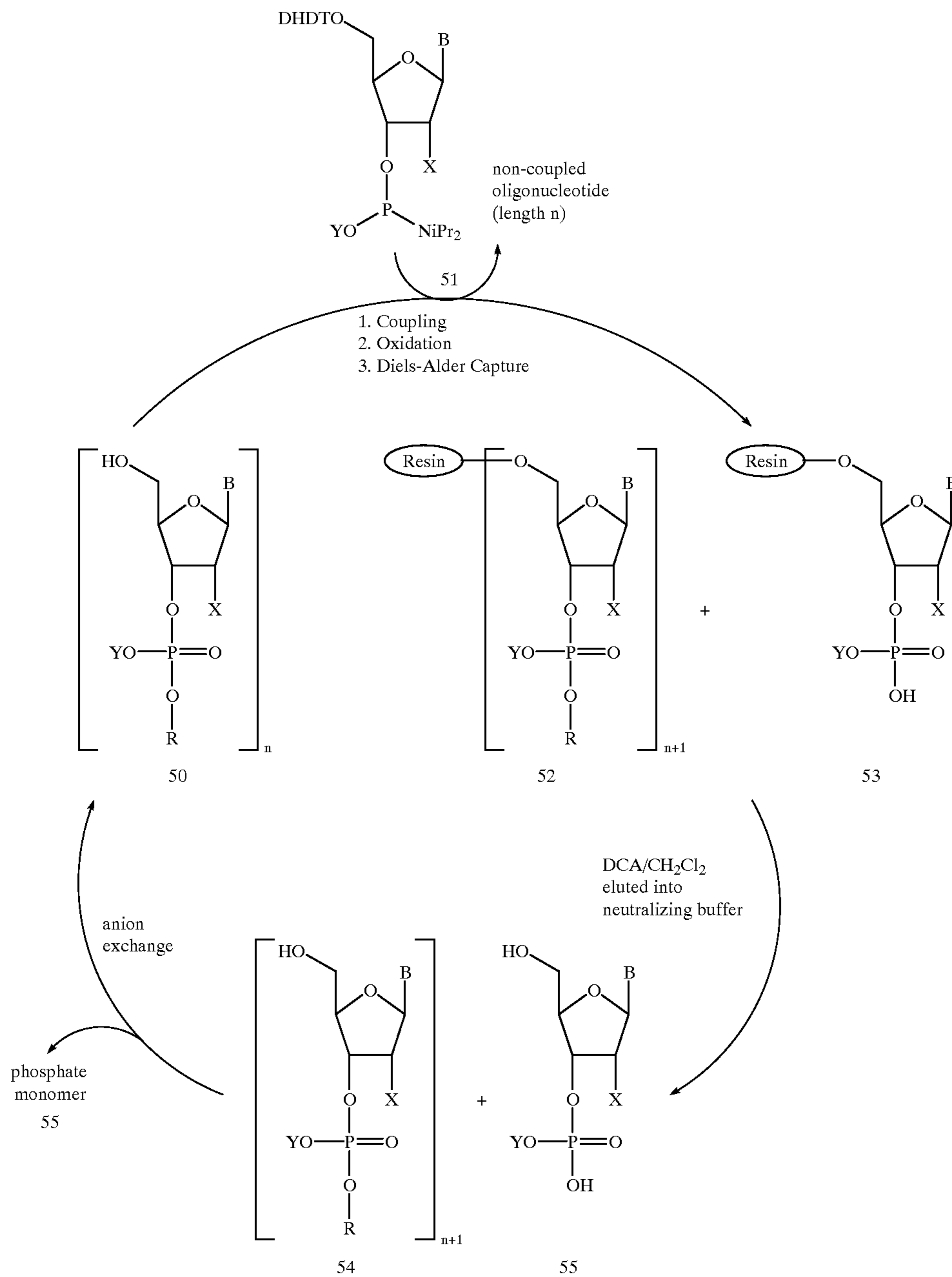
SCHEME 12
