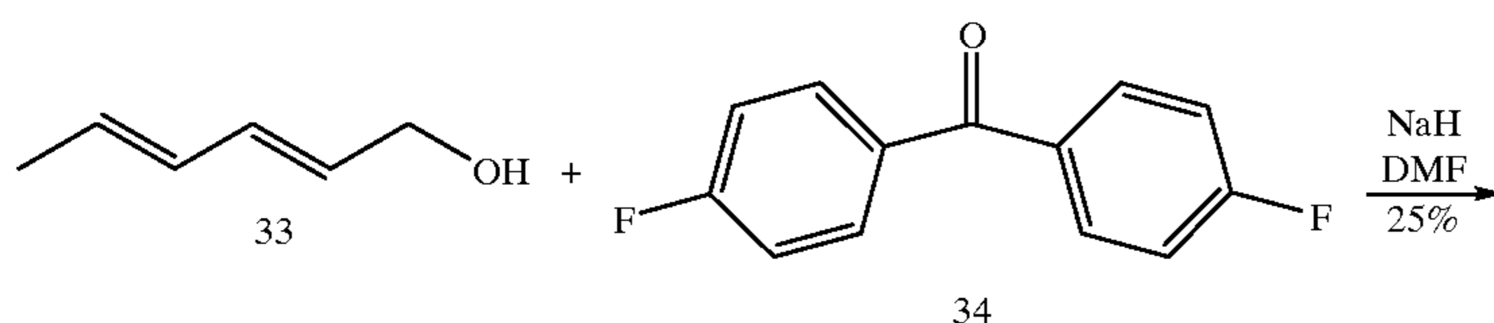
SCHEME 8
