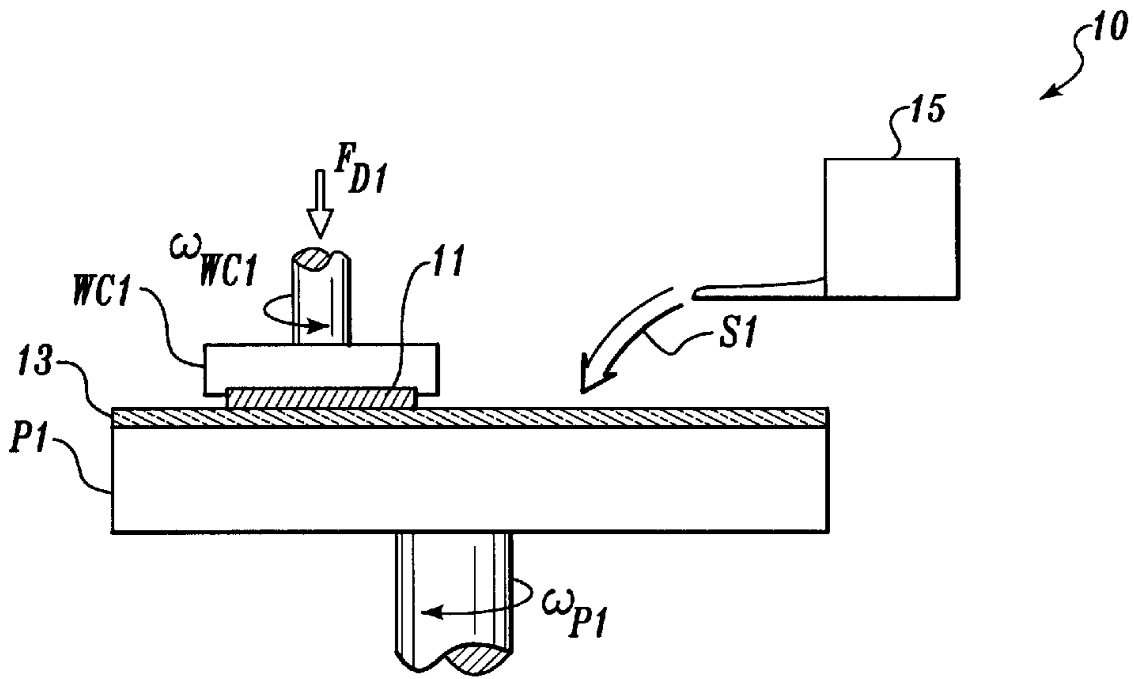
Fig. 1 (PRIOR ART)
