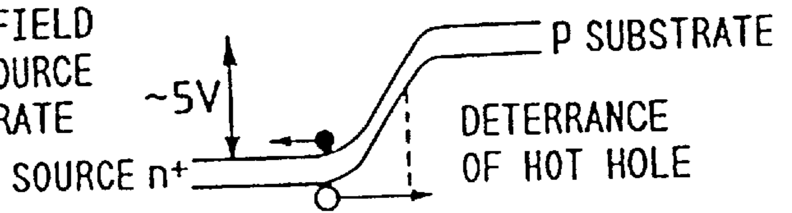
(b) PRESENT INVENTION
