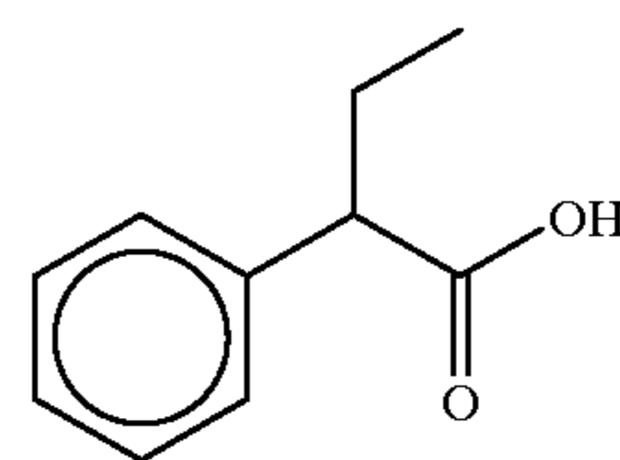
phenylbutyrate
