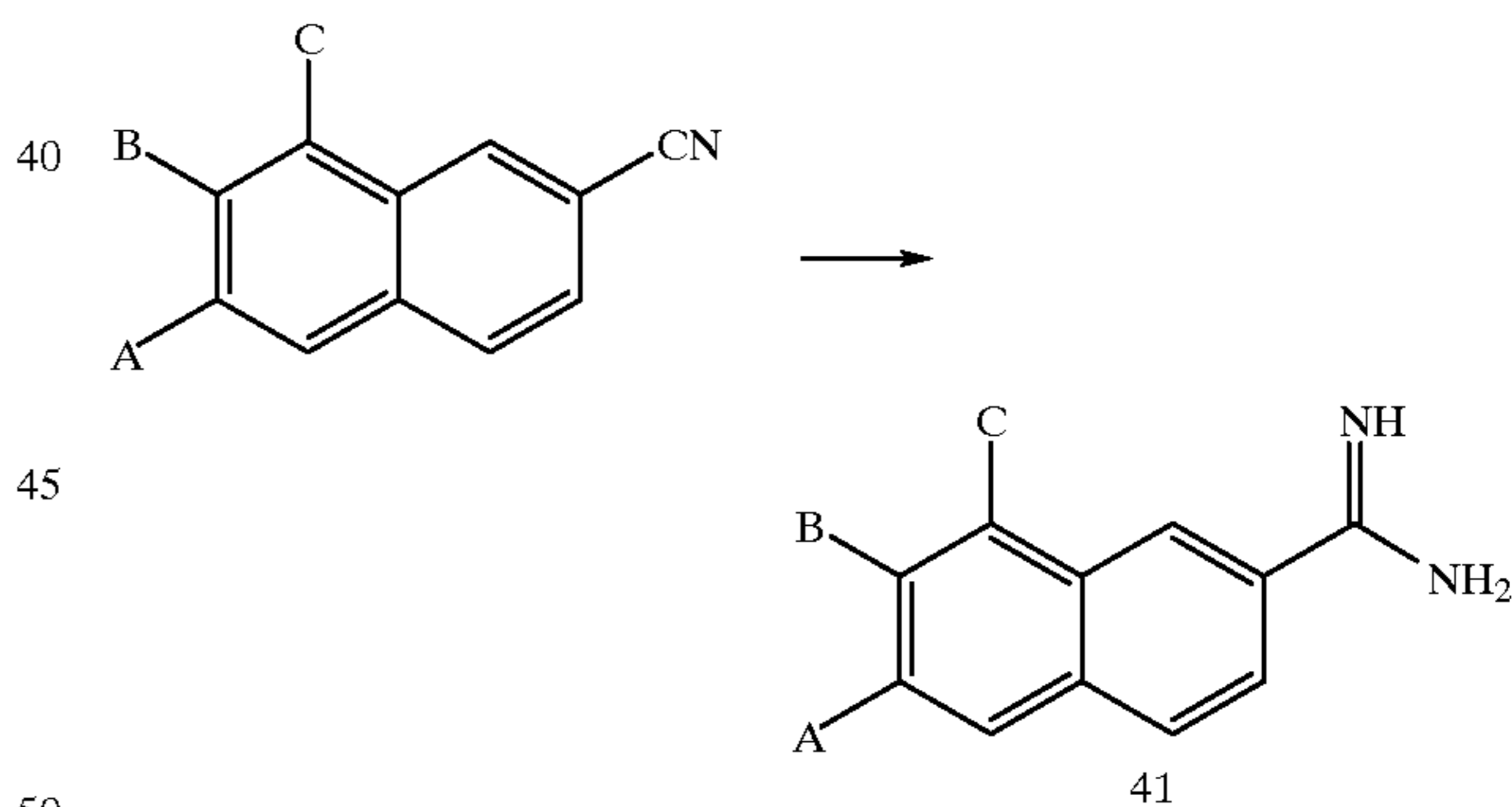
Scheme 7
