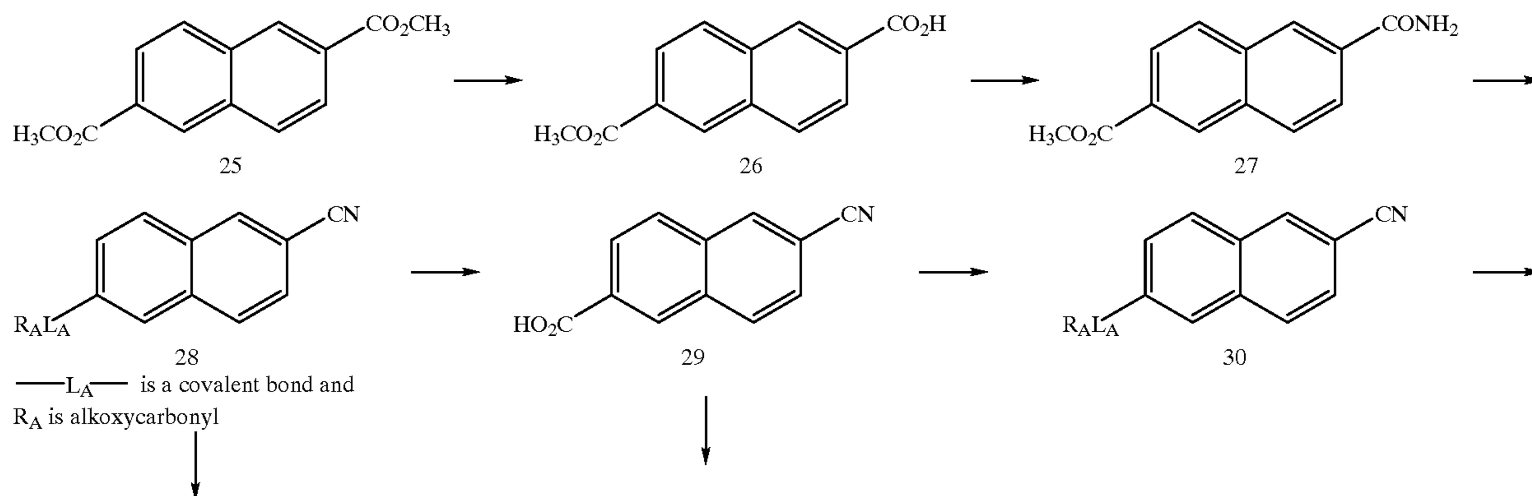
Scheme 5
