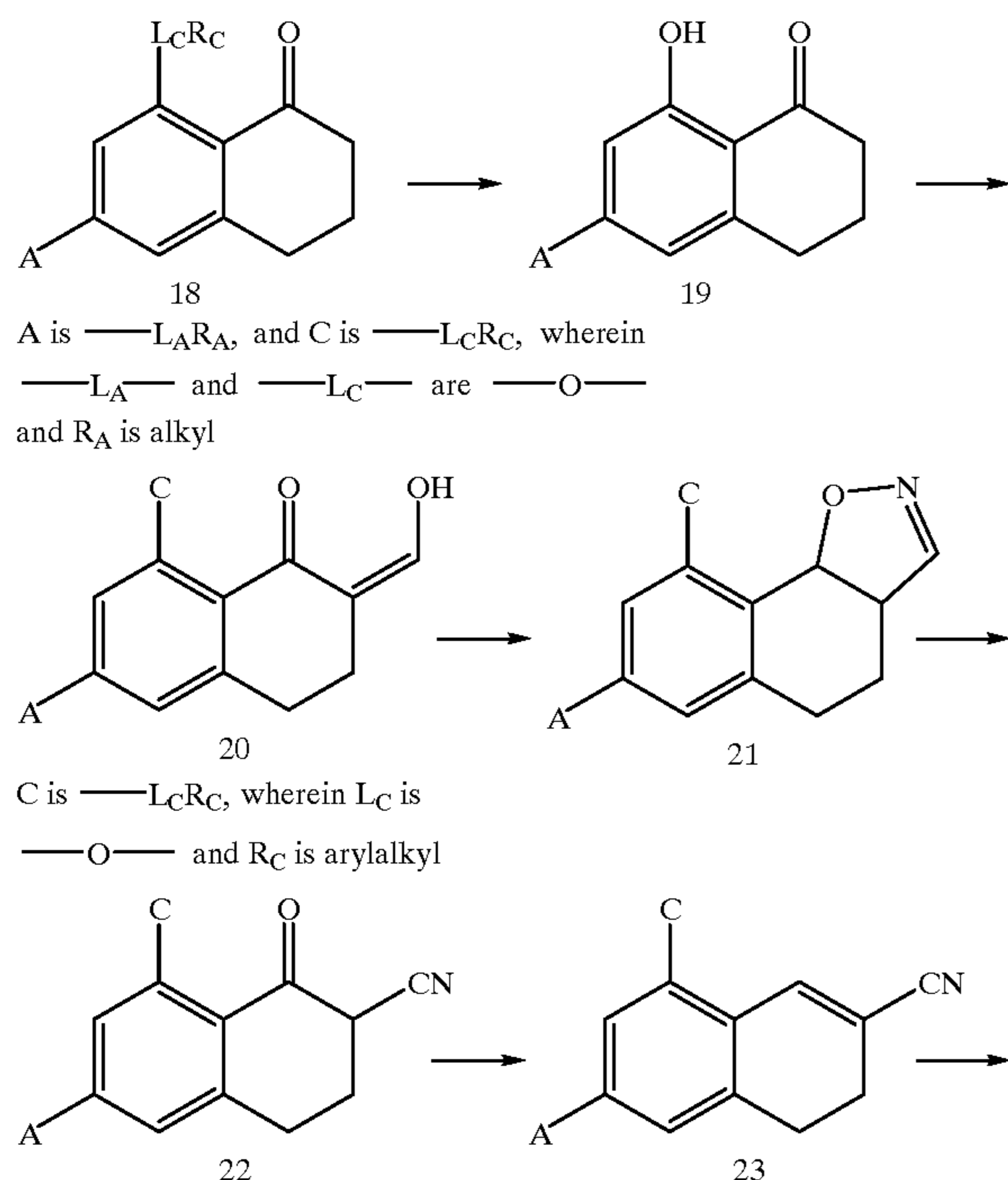
Scheme 4
