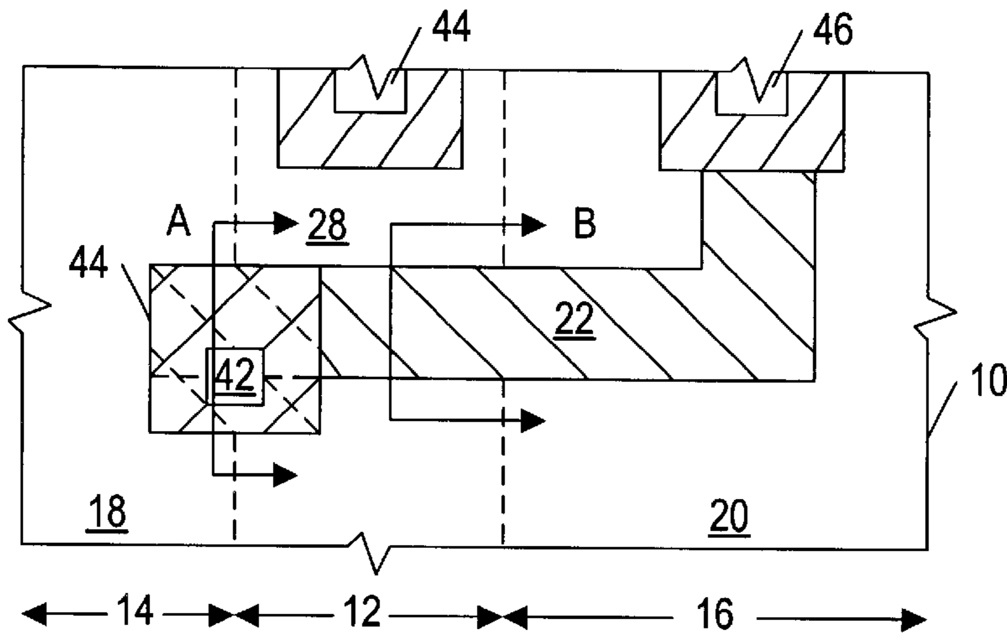
FIG. 1 (PRIOR ART)
