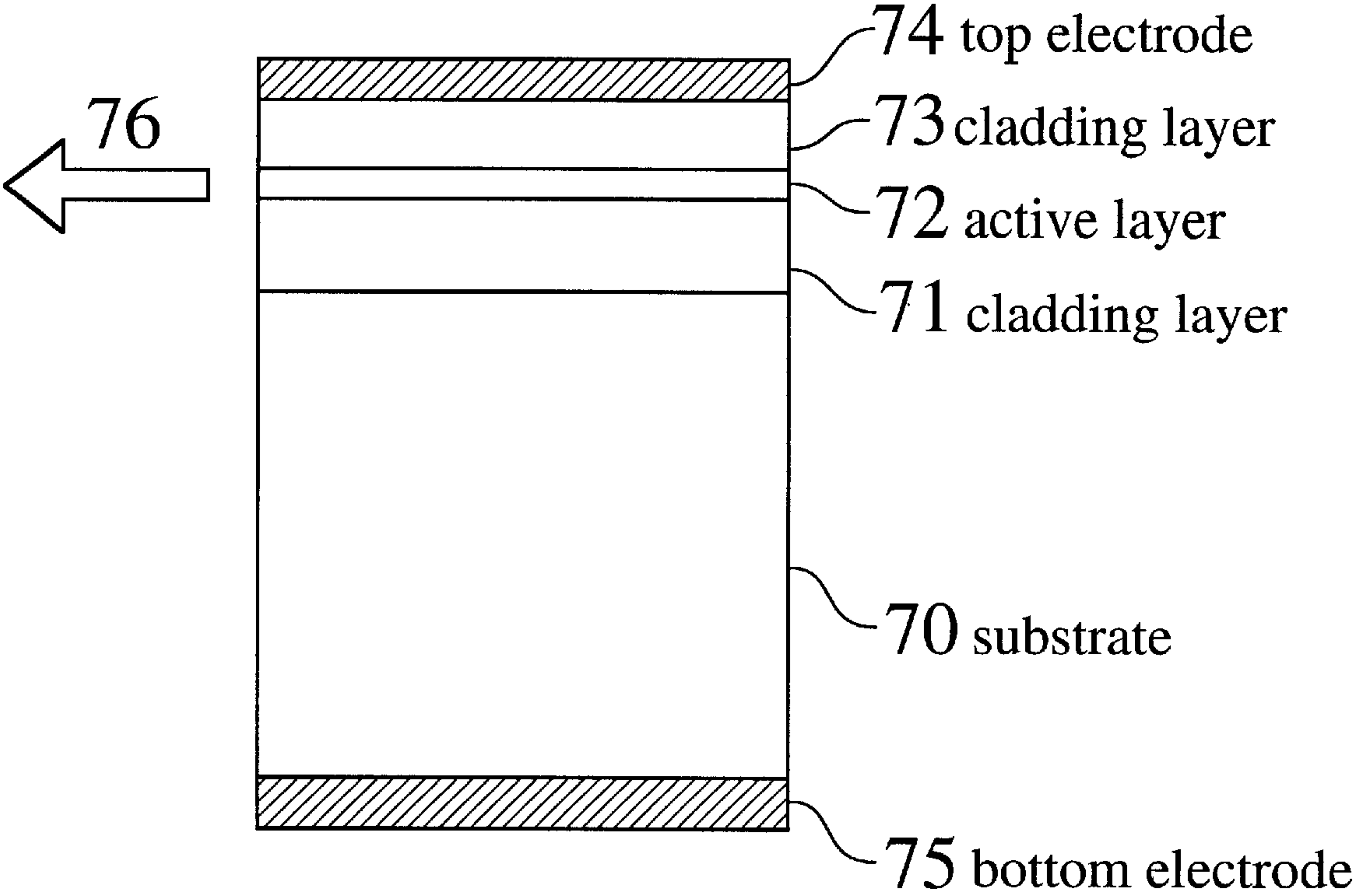
Fig. 1 (PRIOR ART)
