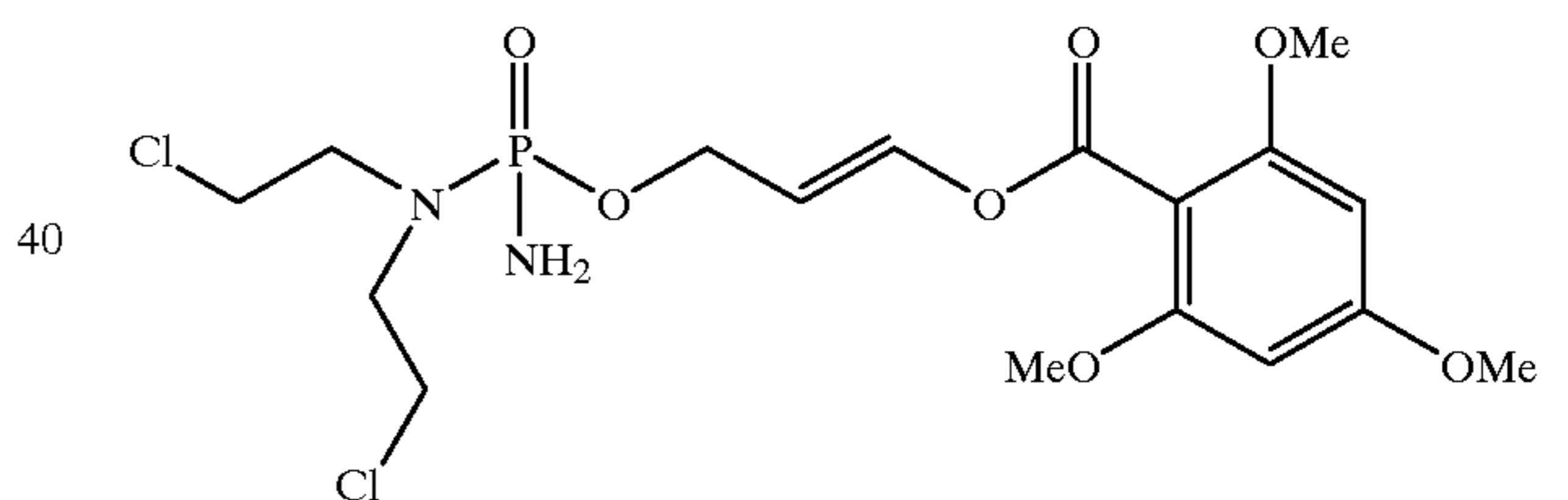
2,4,6-Trimethoxybenzoate ester of enol form of aldophosphamide
