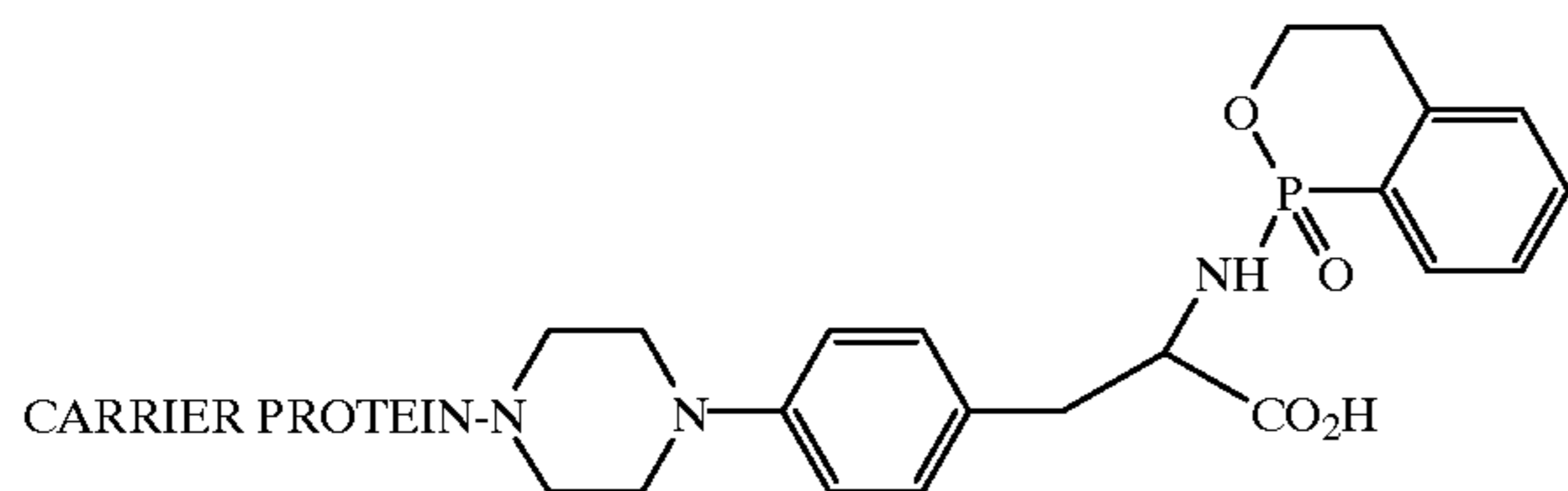
Phosphonate hapten for melphalan-2-hydroxyethyl benzoic acid amide
