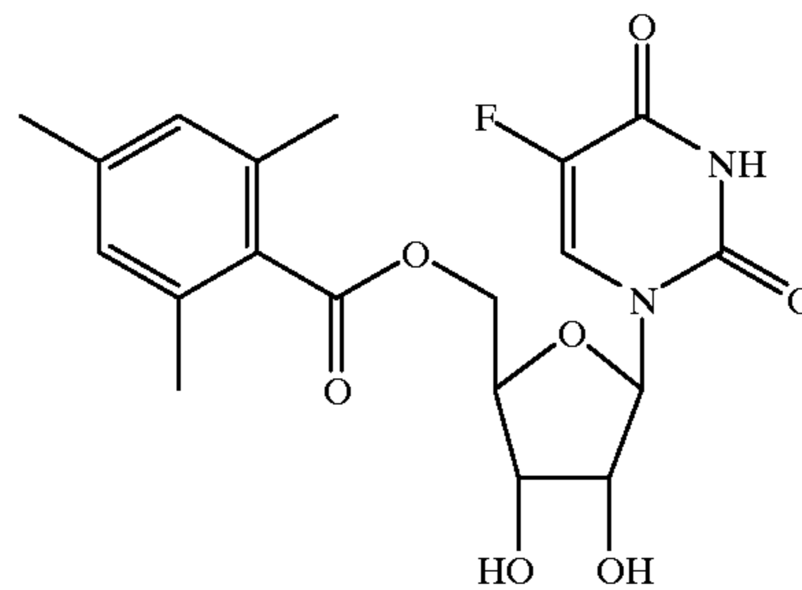
5-Fluorouridine-5'-O-2,4,6 trimethylbenzoate
