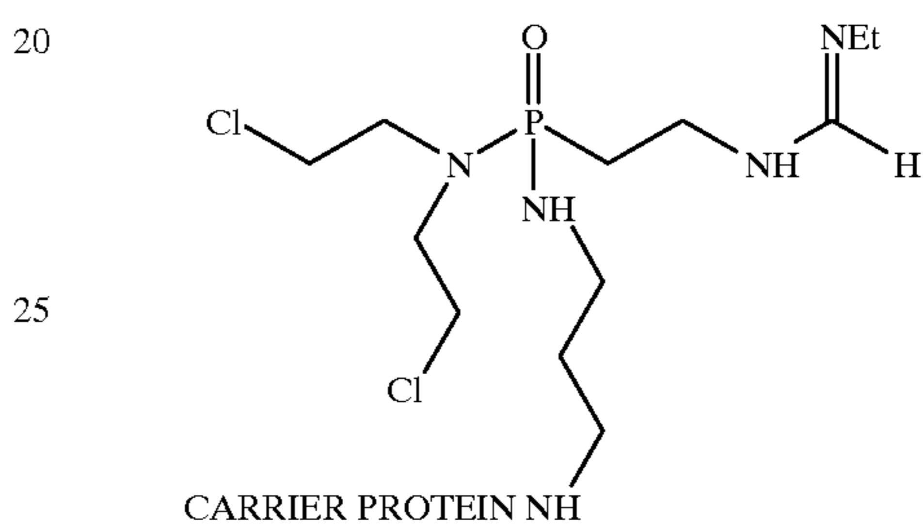
Hapten for aldophosphamide-diethylacetal
