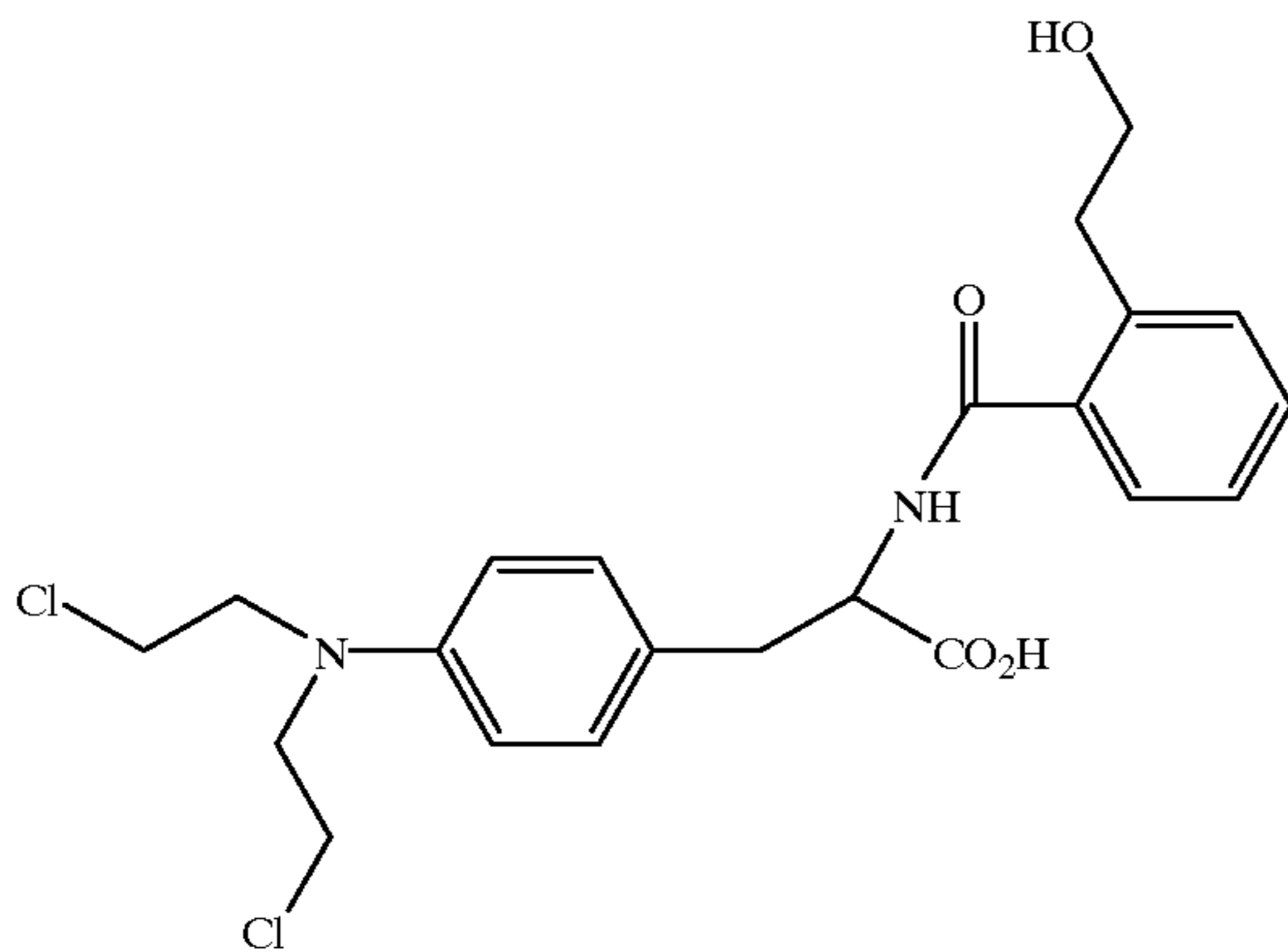
Phosphonate hapten for melphalan-2-hydroxyethyl benzoic acid amide
