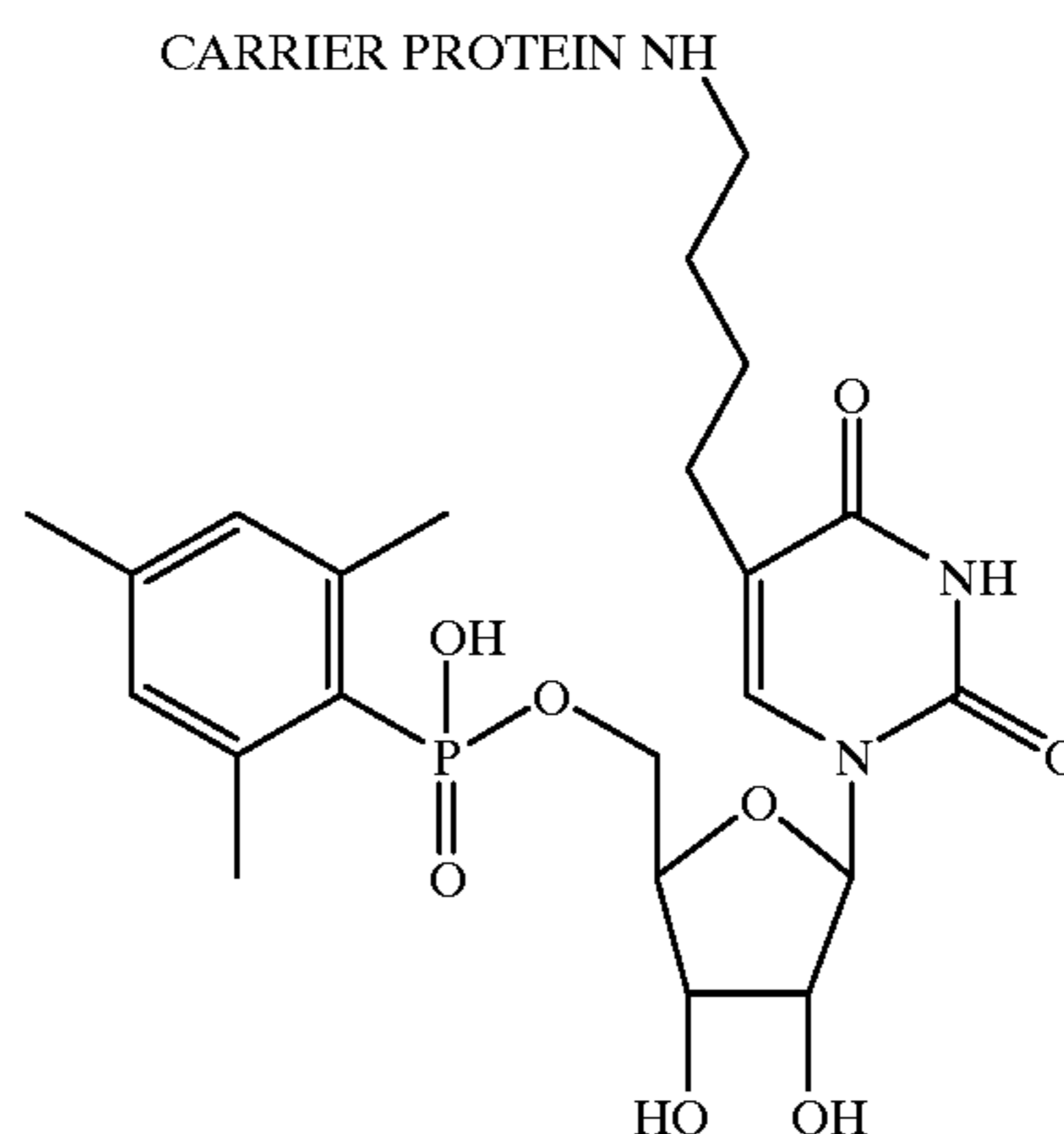
Phosphonate hapten for 5-fluorouridine-5'-O-2,4,6 trimethylbenzoate
