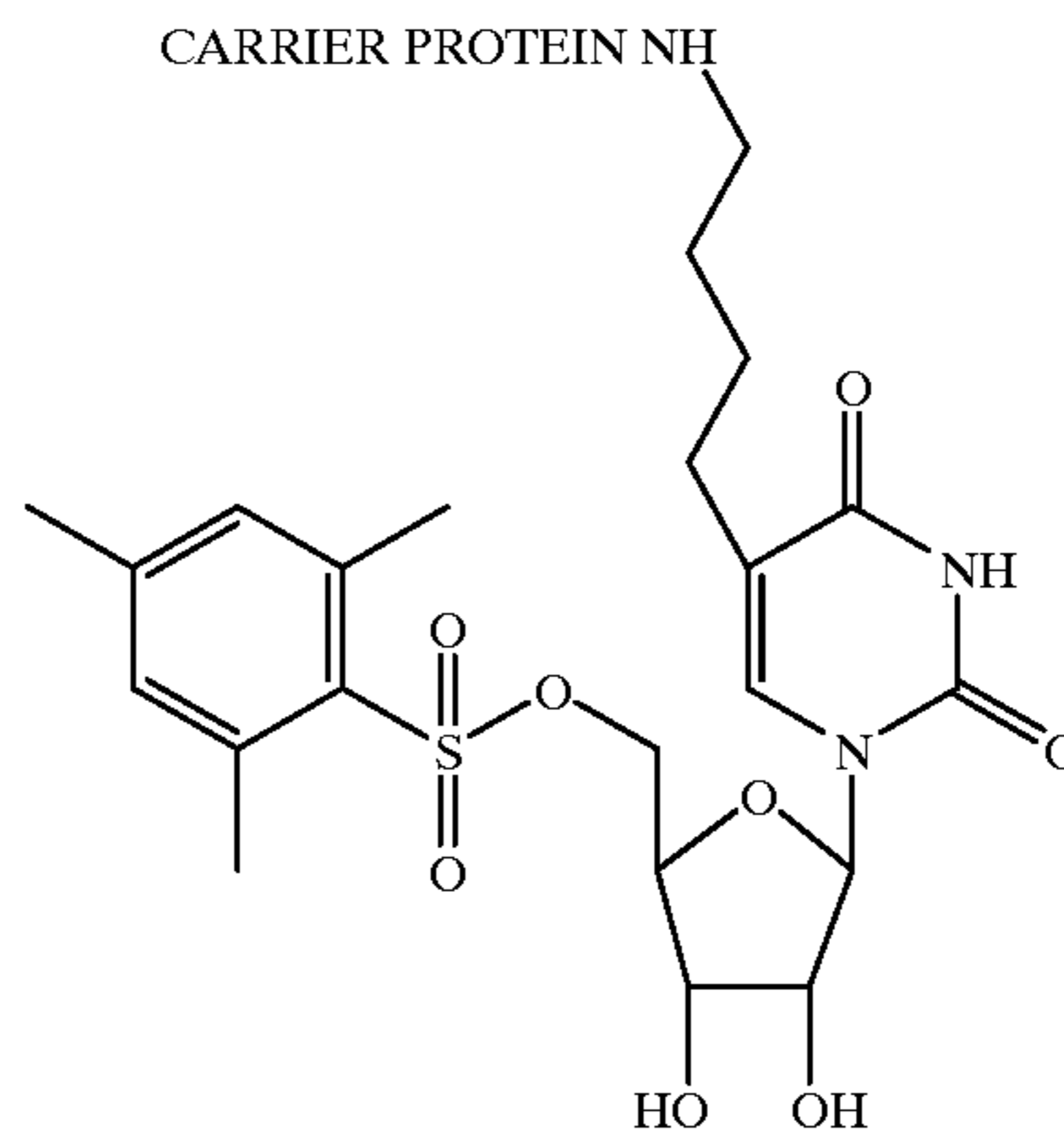
Sulphonate hapten for 5-fluorouridine-5'-O-2,4,6 trimethylbenzoate
