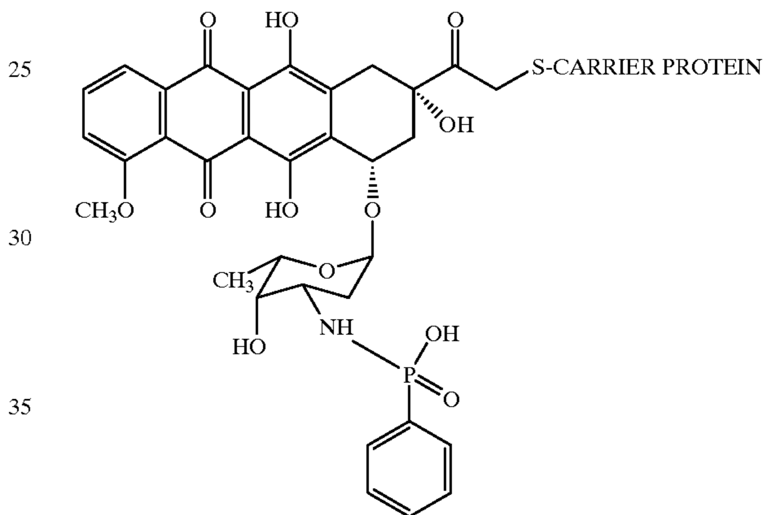
Phosphonate hapten for doxorubicin-benzoic acid amide
