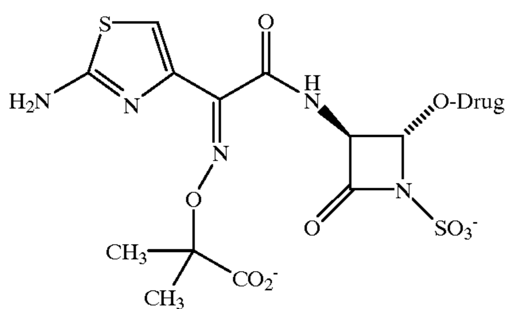
Aztreonam-based Prodrug
