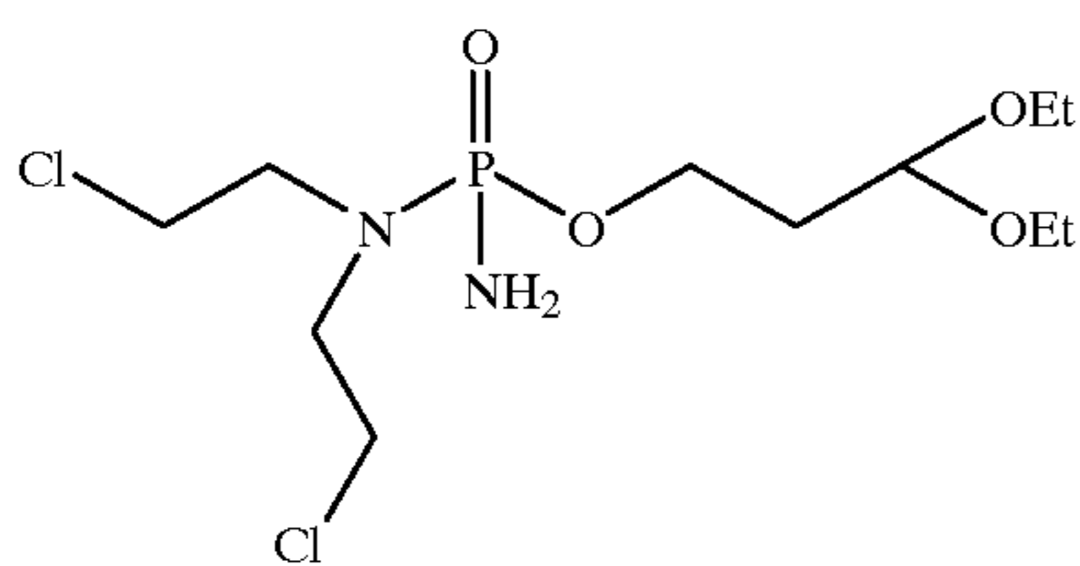
Aldophosphamide-diethylacetal
