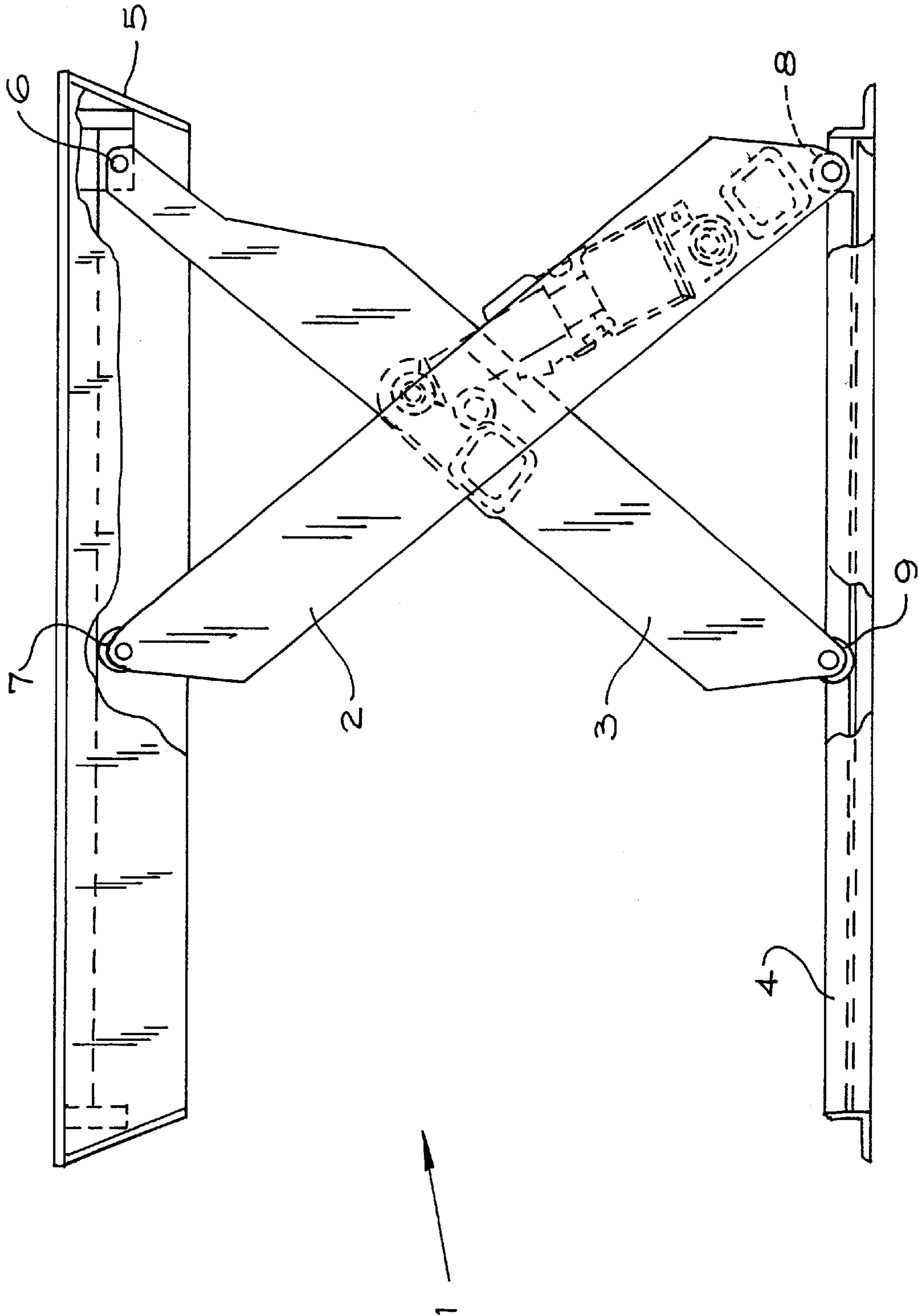
Fig. 3 (Prior Art)
