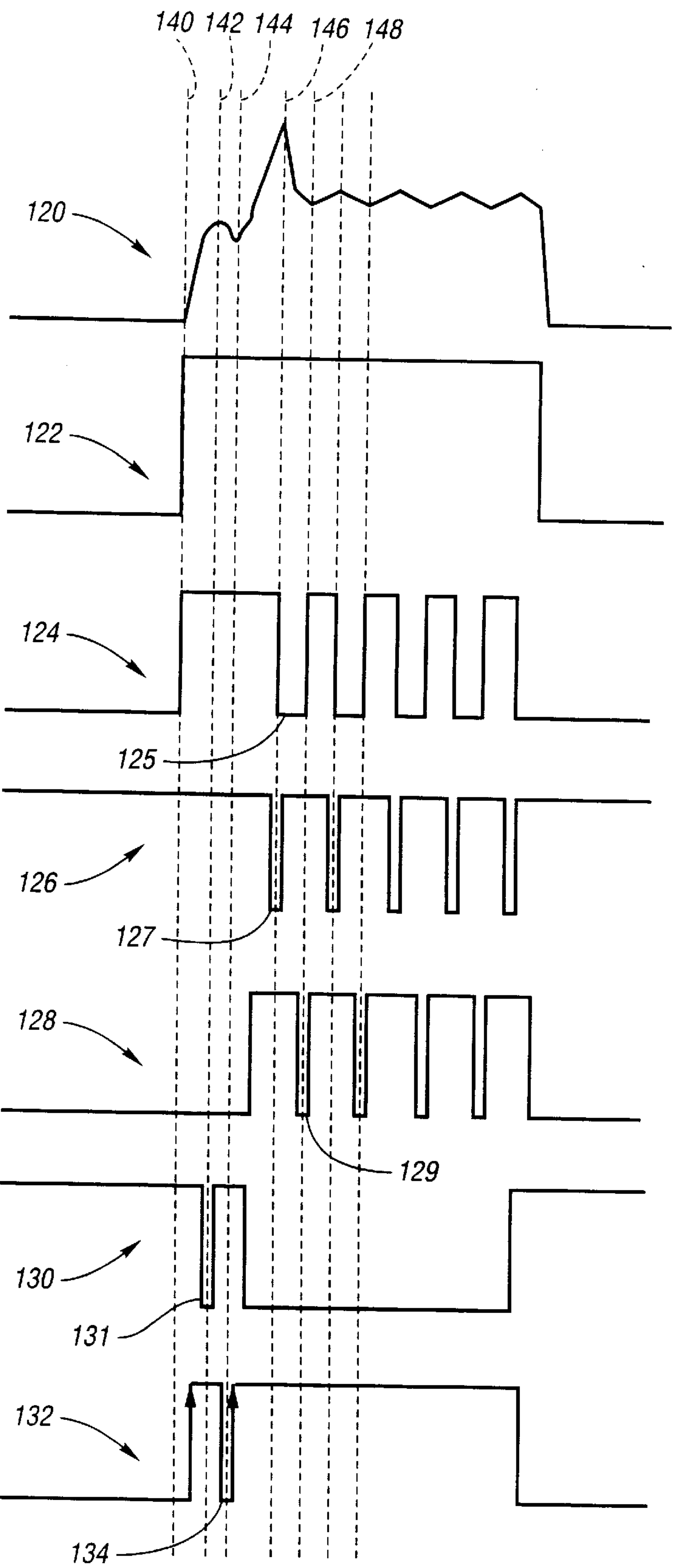
Fig. 4d COMPARATOR A
