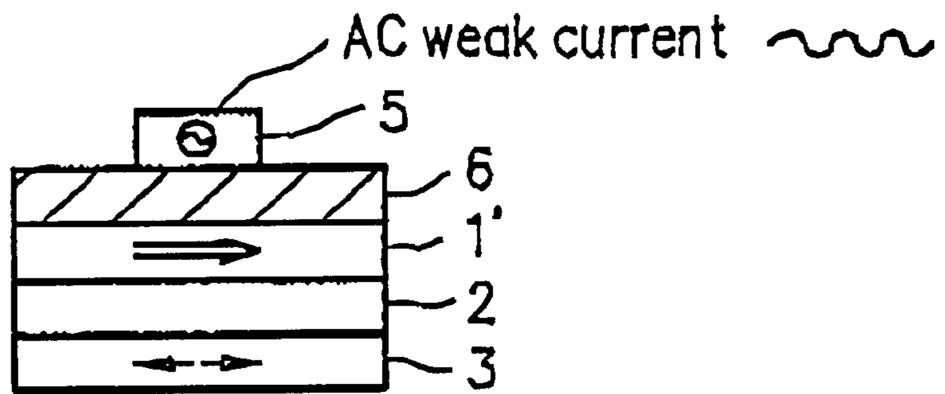
FIG. 8B Amplifying operation
