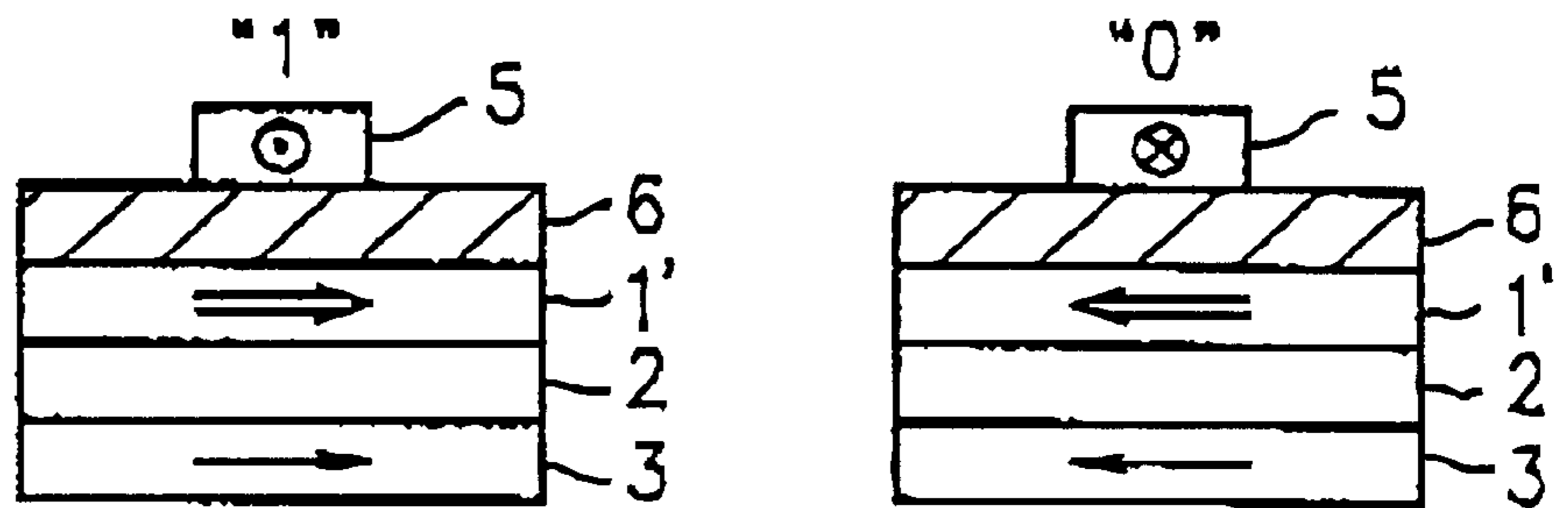
FIG. 6A Information recording by current
