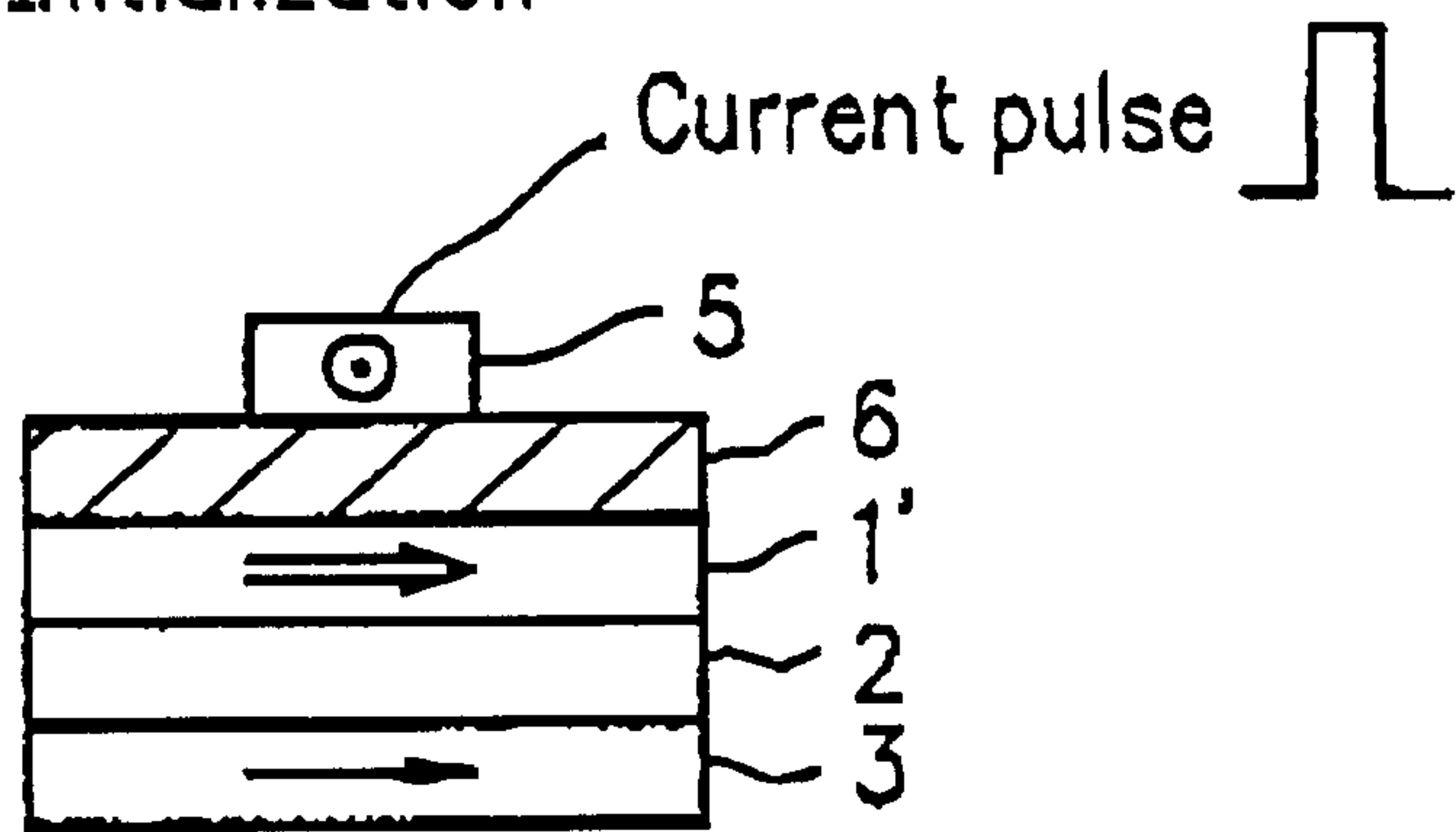
FIG. 8A Initialization
