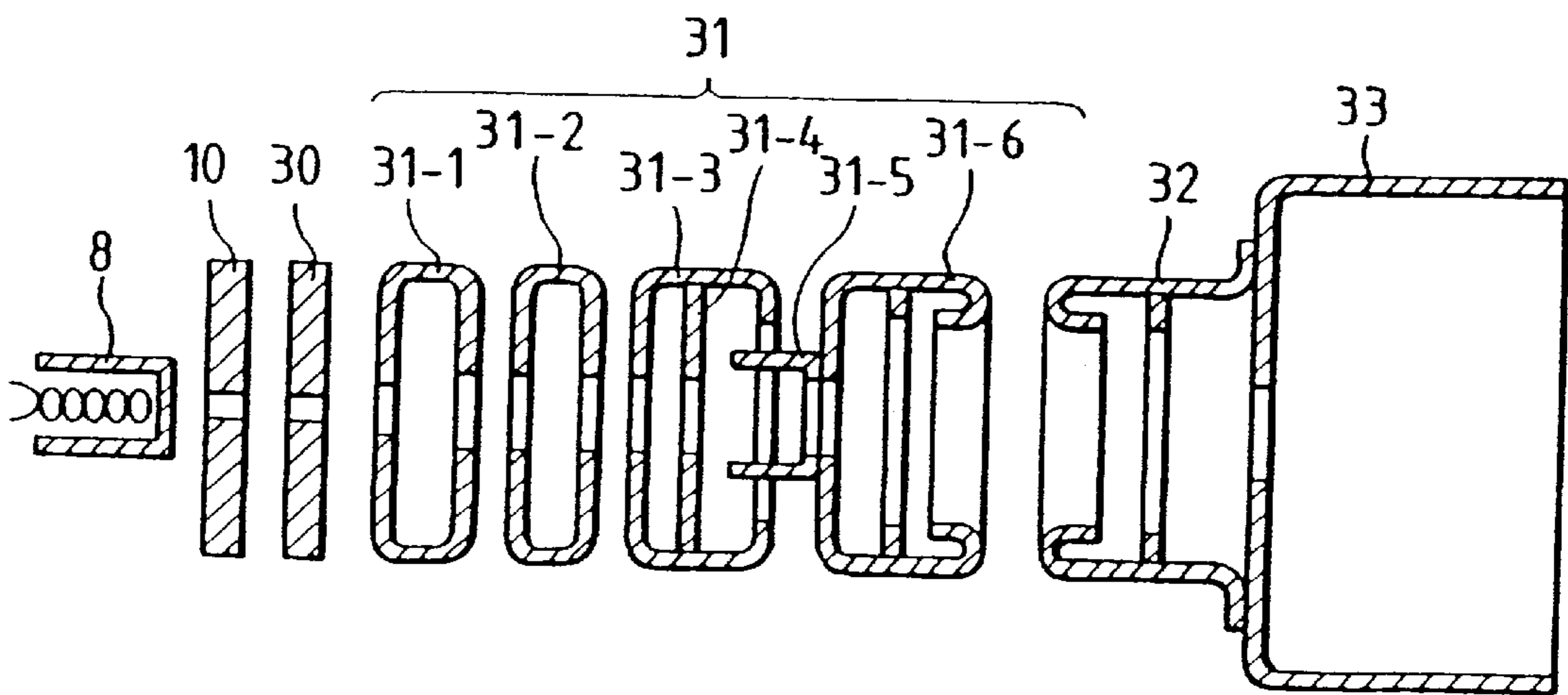
FIG. 6 (PRIOR ART)
