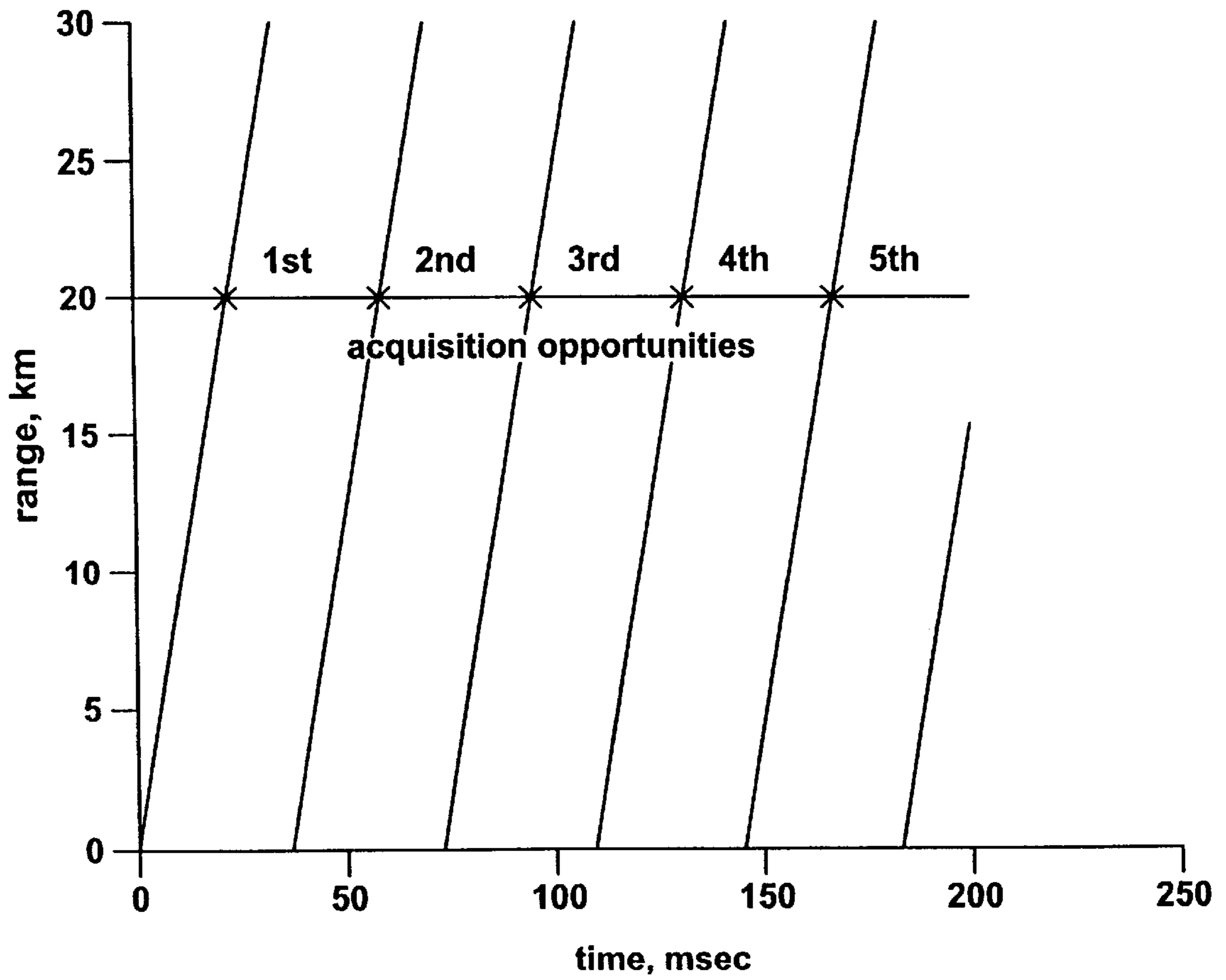
Mean Cell Sweep Time, FSU @ 20 KM
