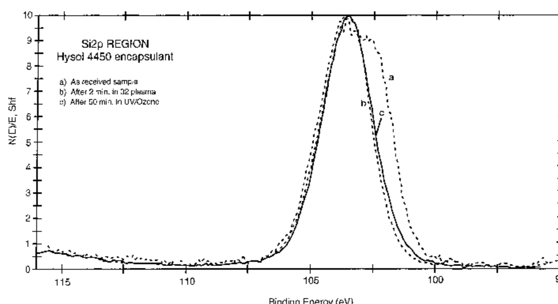
ESCA Multiplex 6 Oct 95 Area: 1 Species: Si1 Region: 4 Angle: -45 degrees Acquisition Time: 12.00 min File: jk5065_2 Hysol encapsulant_44-51_48-48 Scale Factor: 0.120 keV Offset: 0.214 keV Pass Energy: 23.500 eV Aperture: 4 A1 400W
