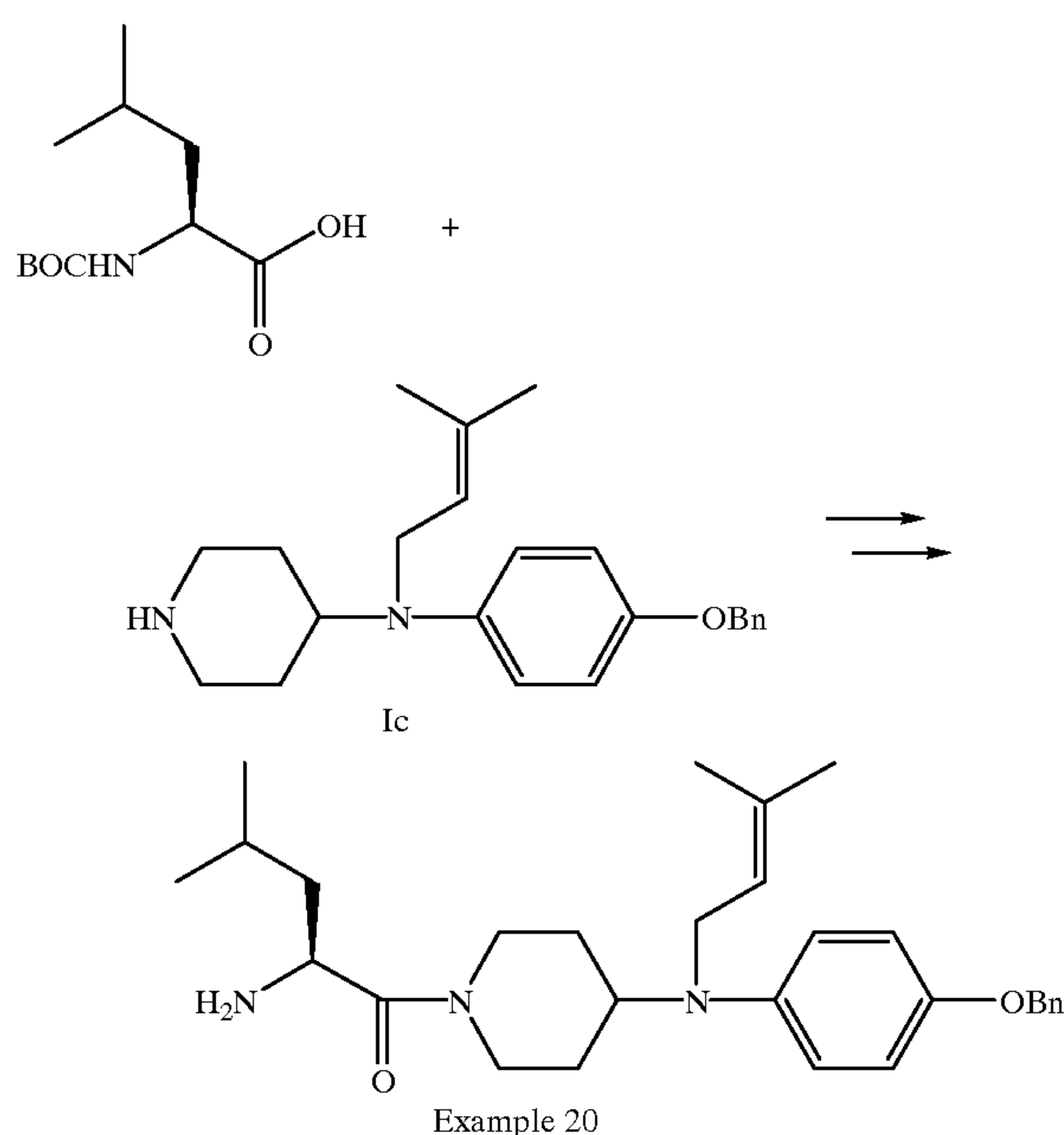
Scheme XIII
