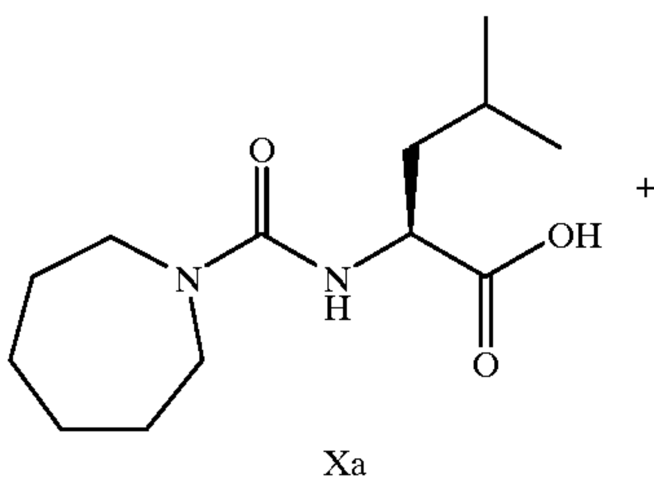
Scheme VII
