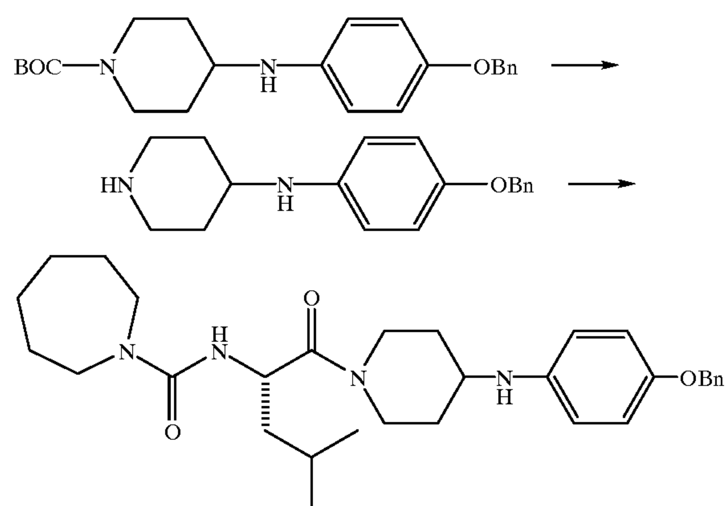
Example 28
