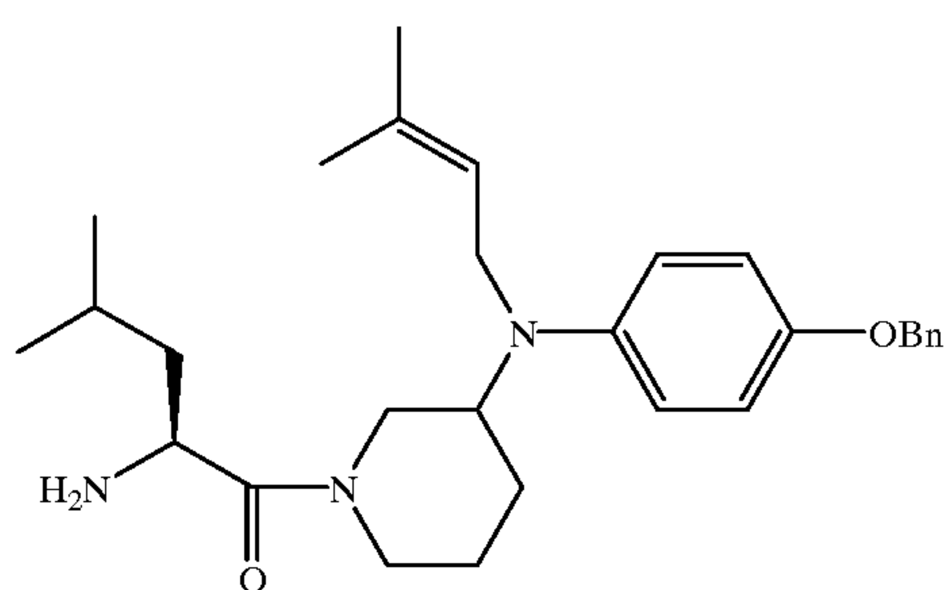
Example 45
