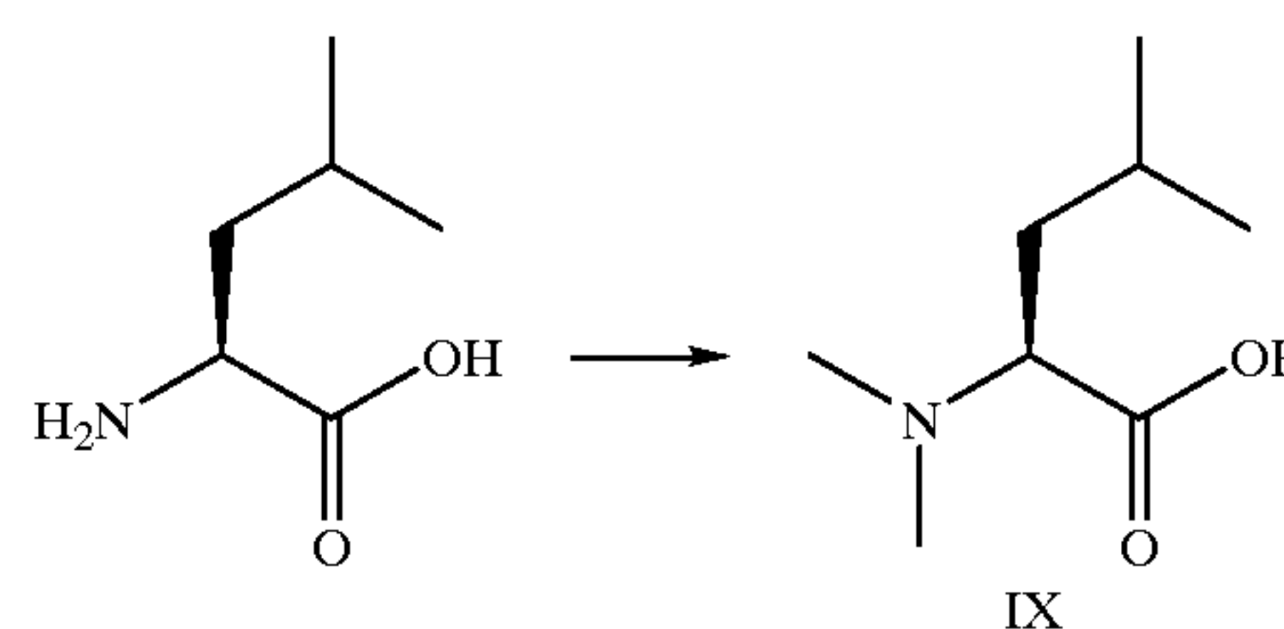
Scheme IX
