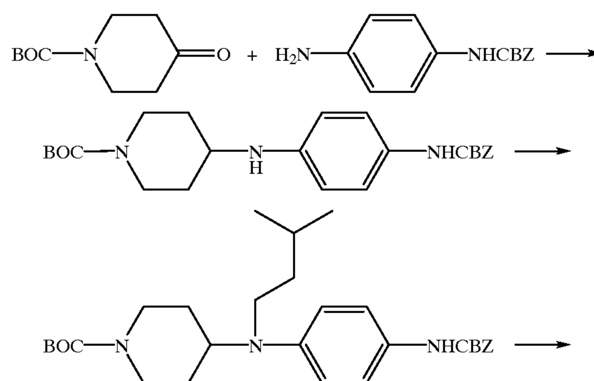
Scheme XVI
