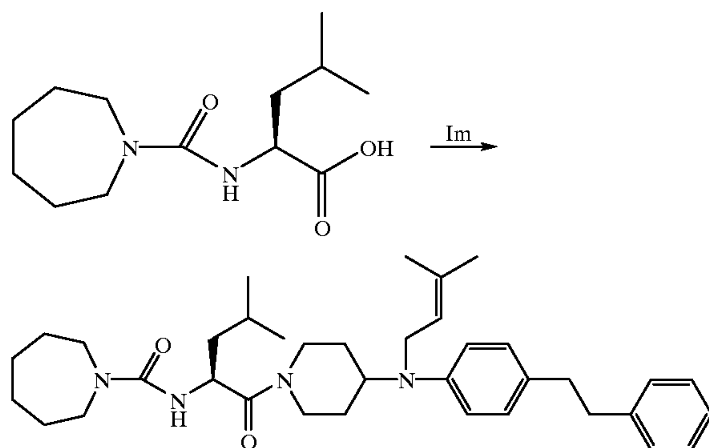
Example 51
