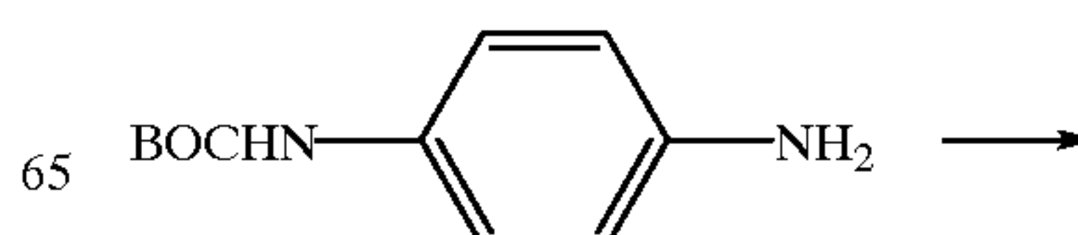
Scheme XV
