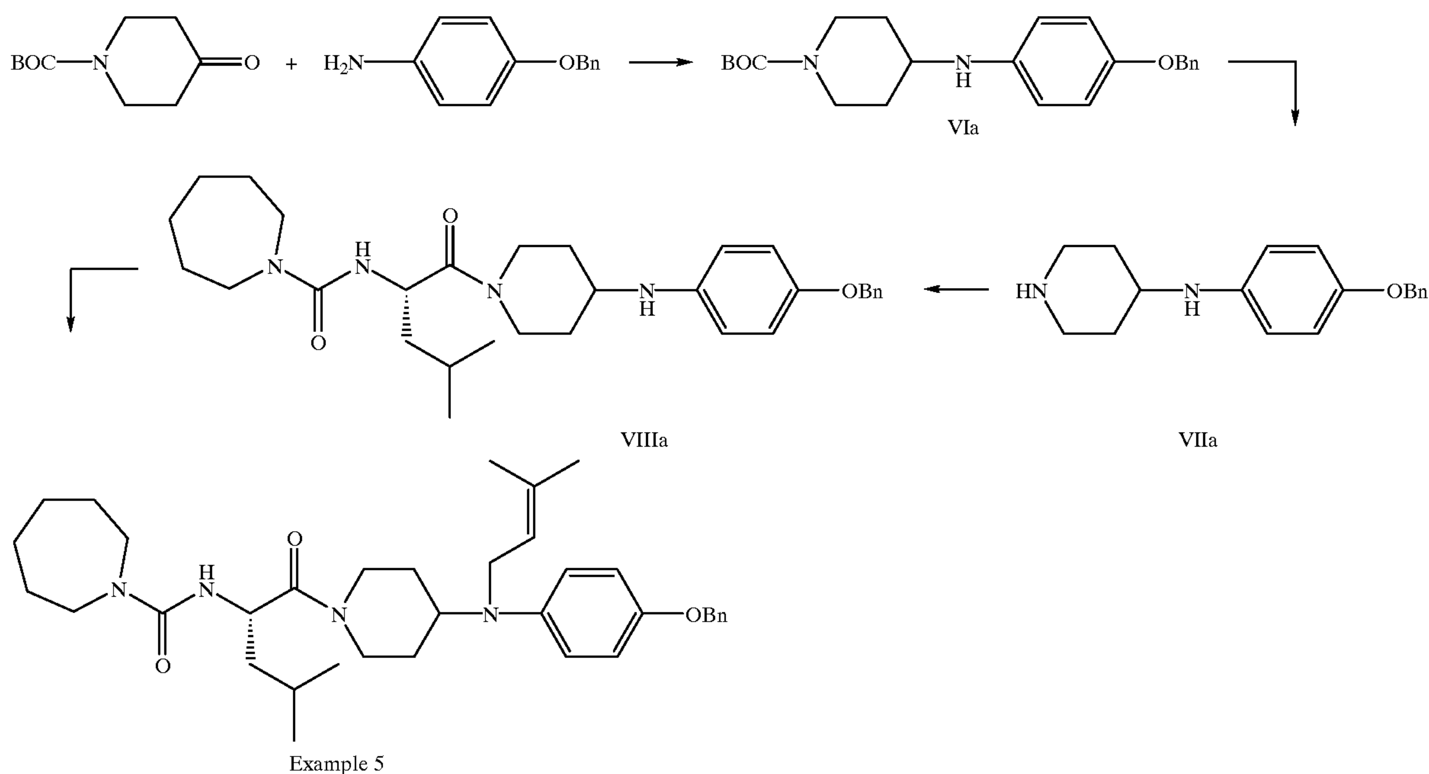
Scheme VIII
