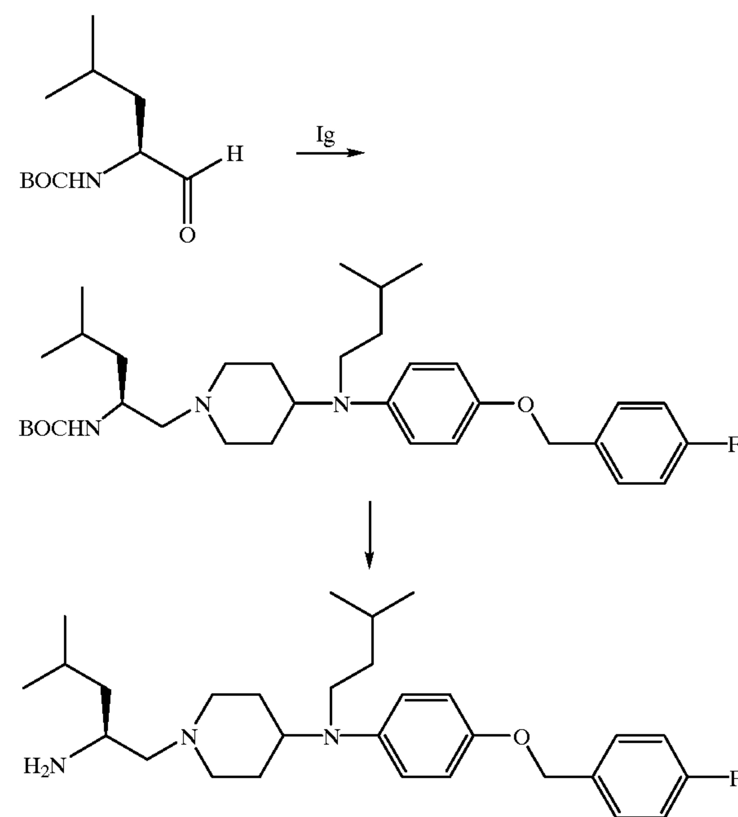
Example 49
