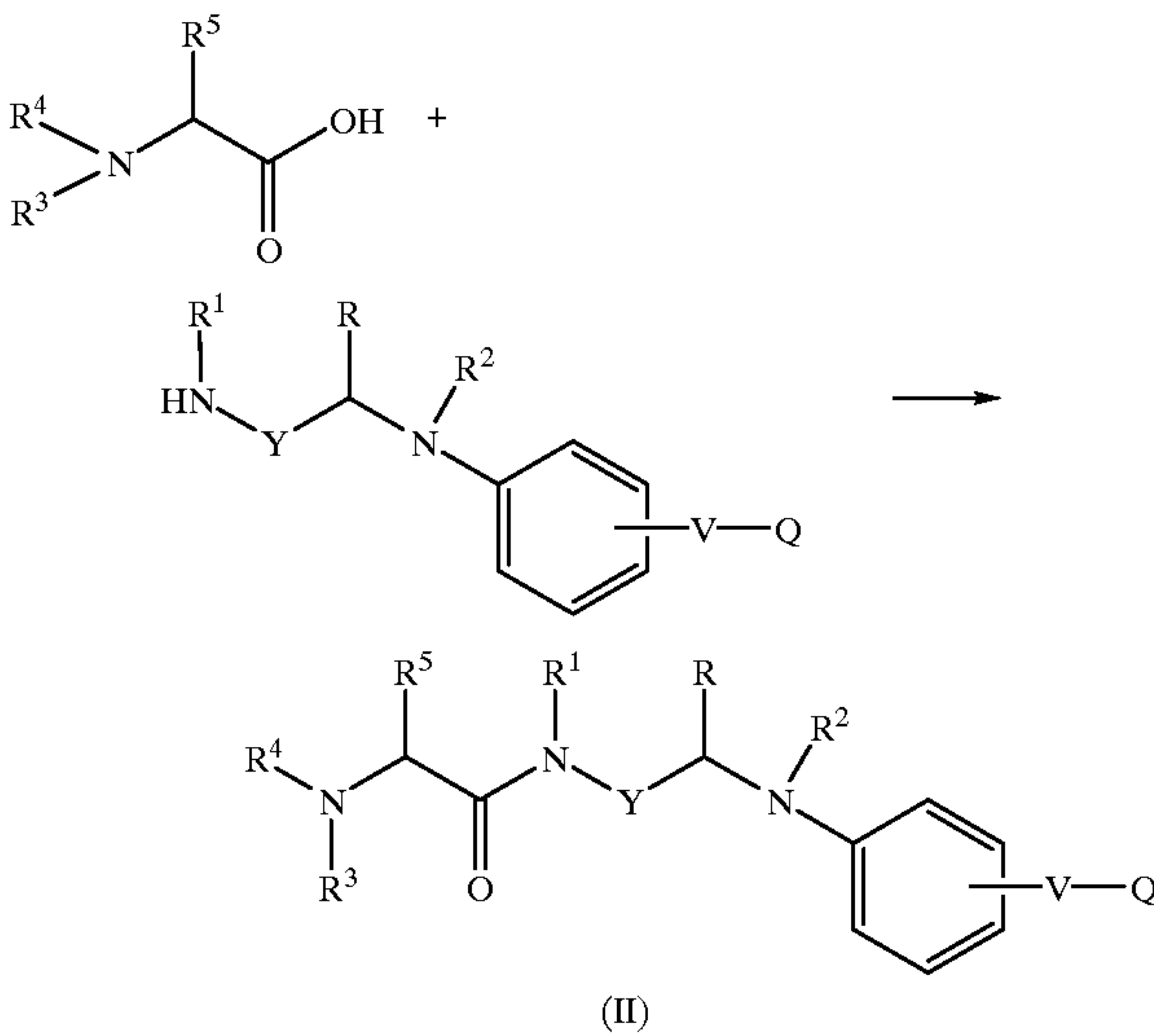
Scheme IV
