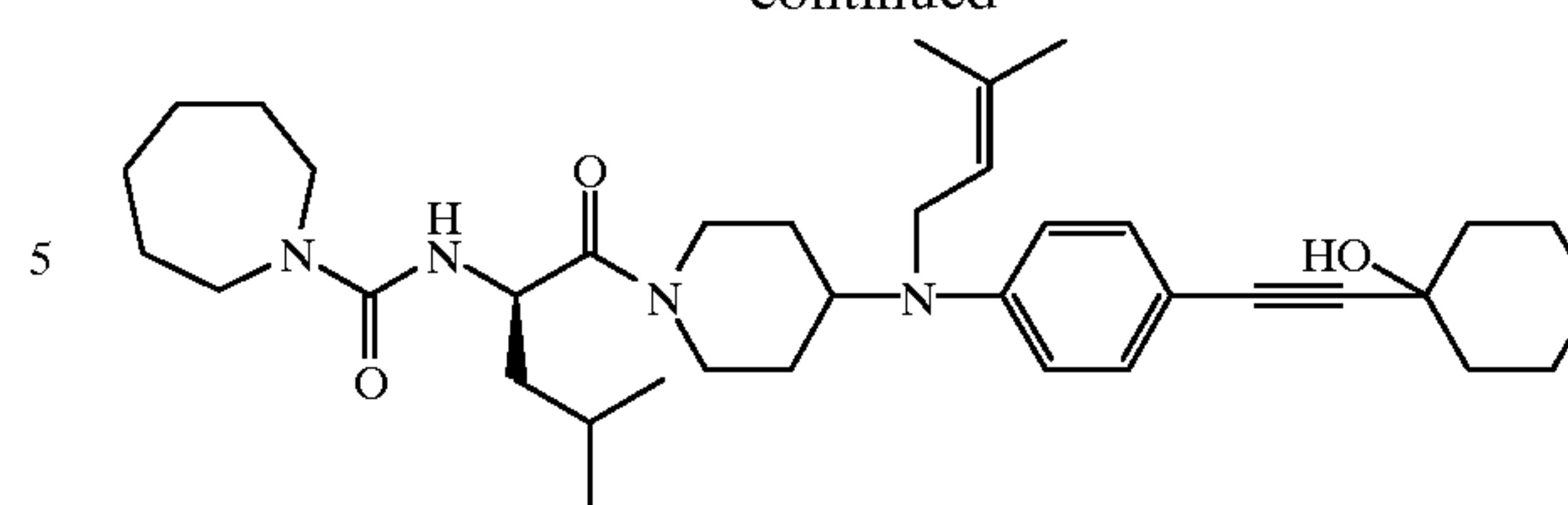
Example 43
