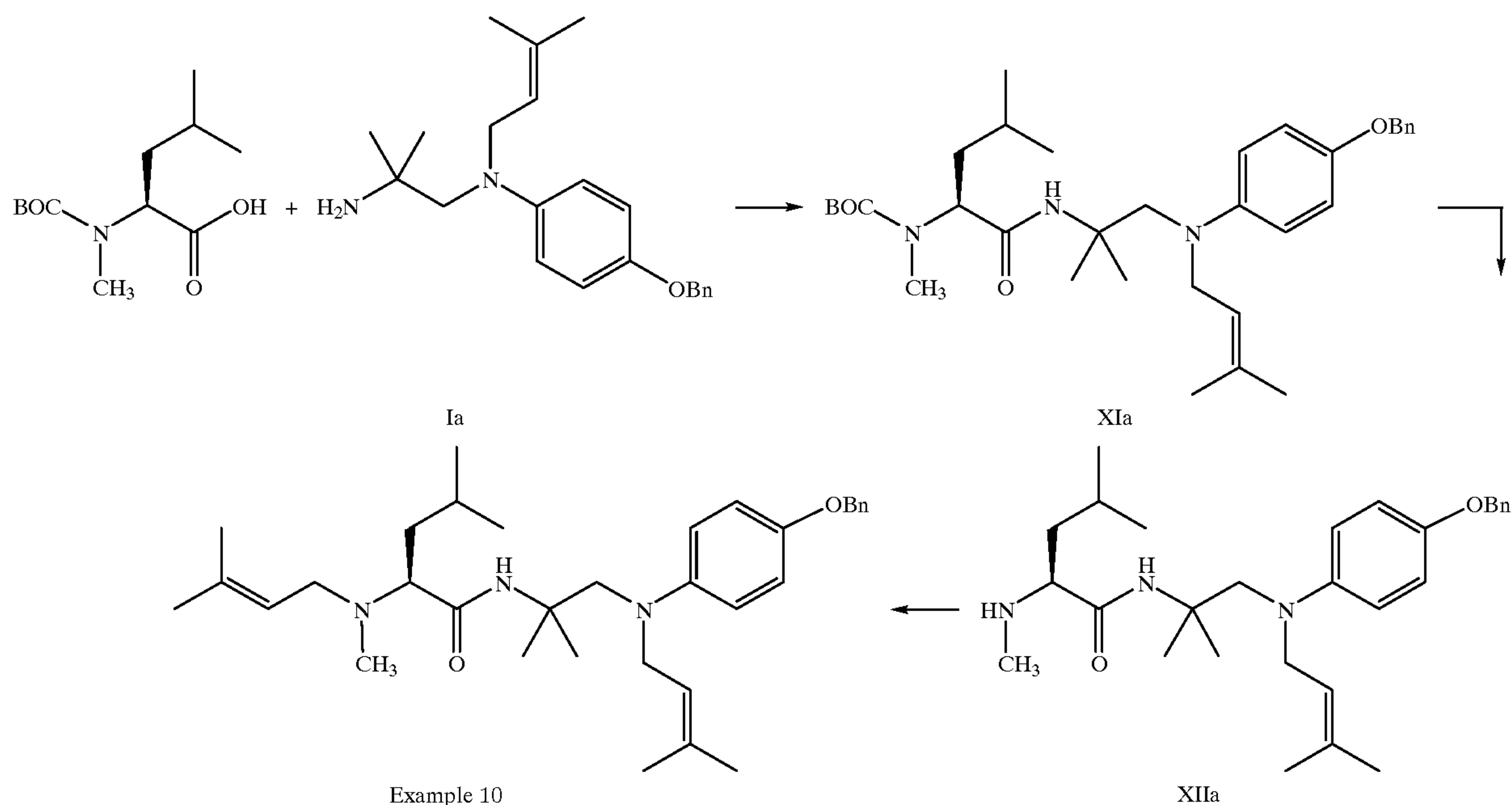
Scheme XI
