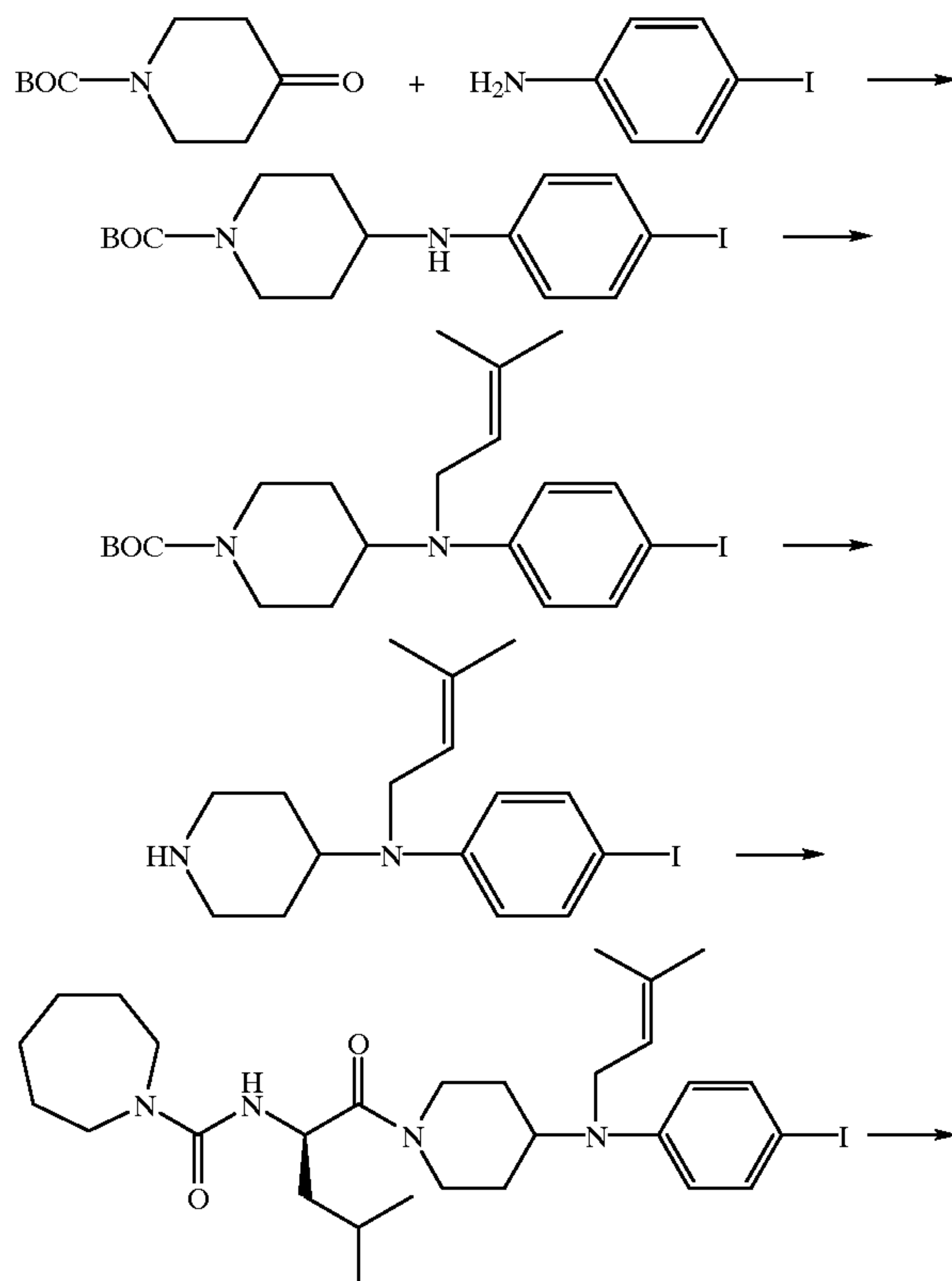
Scheme XVII
