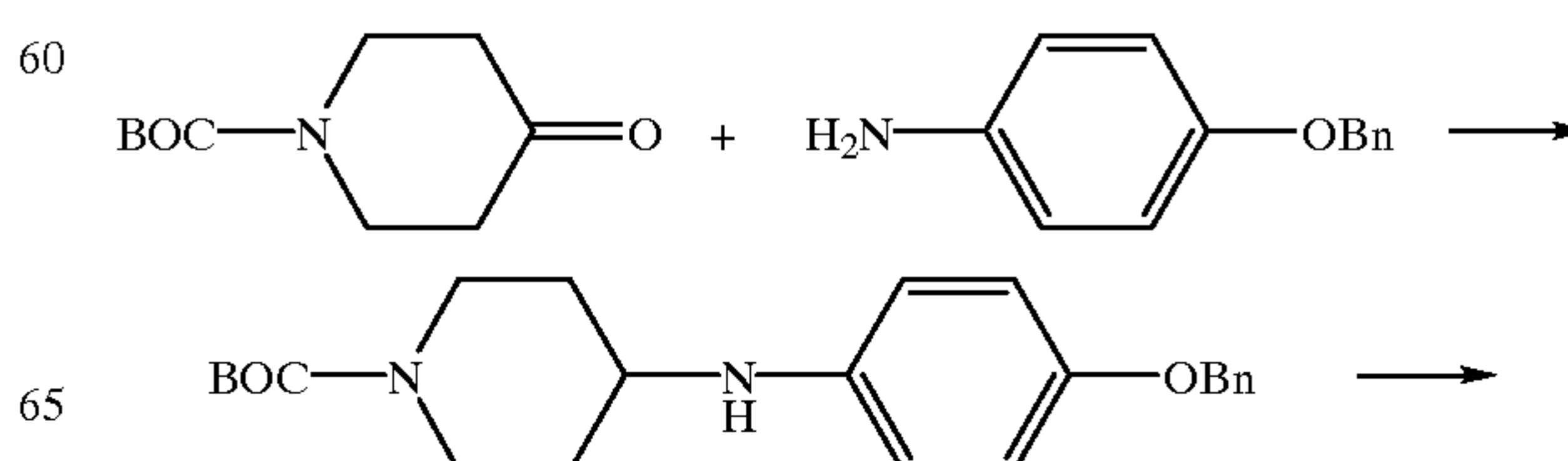
Scheme XII
