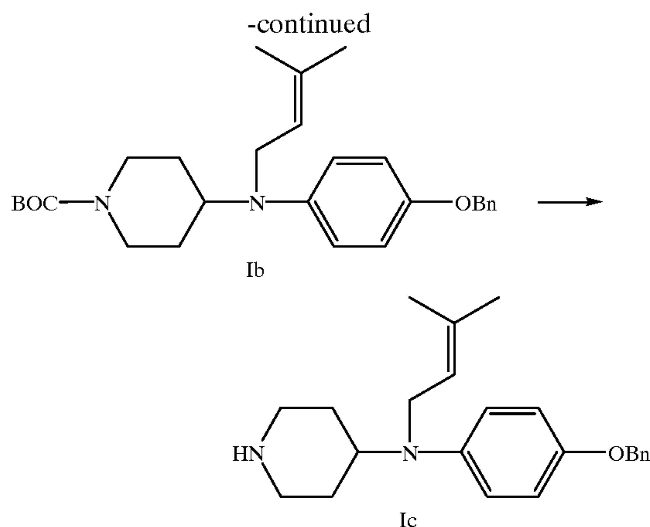
Scheme XIII
