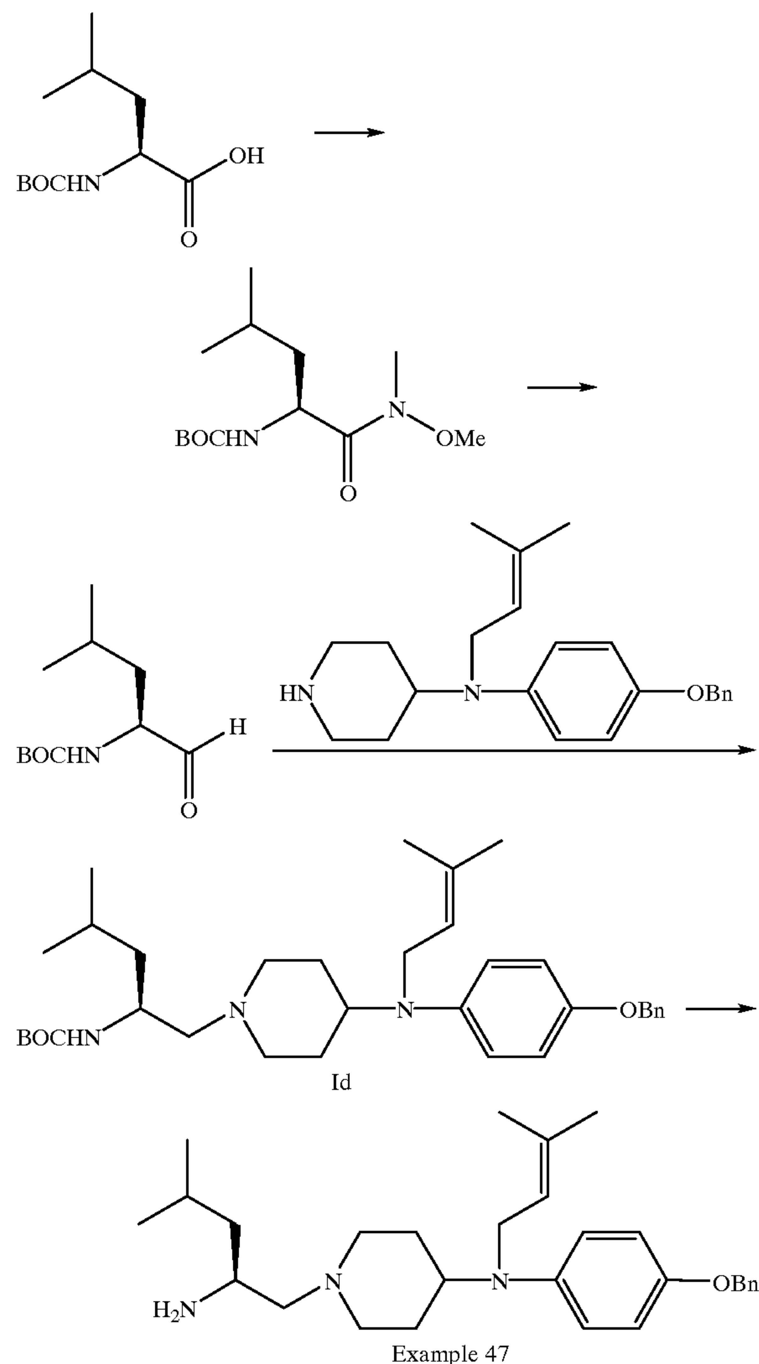
Scheme XIX
