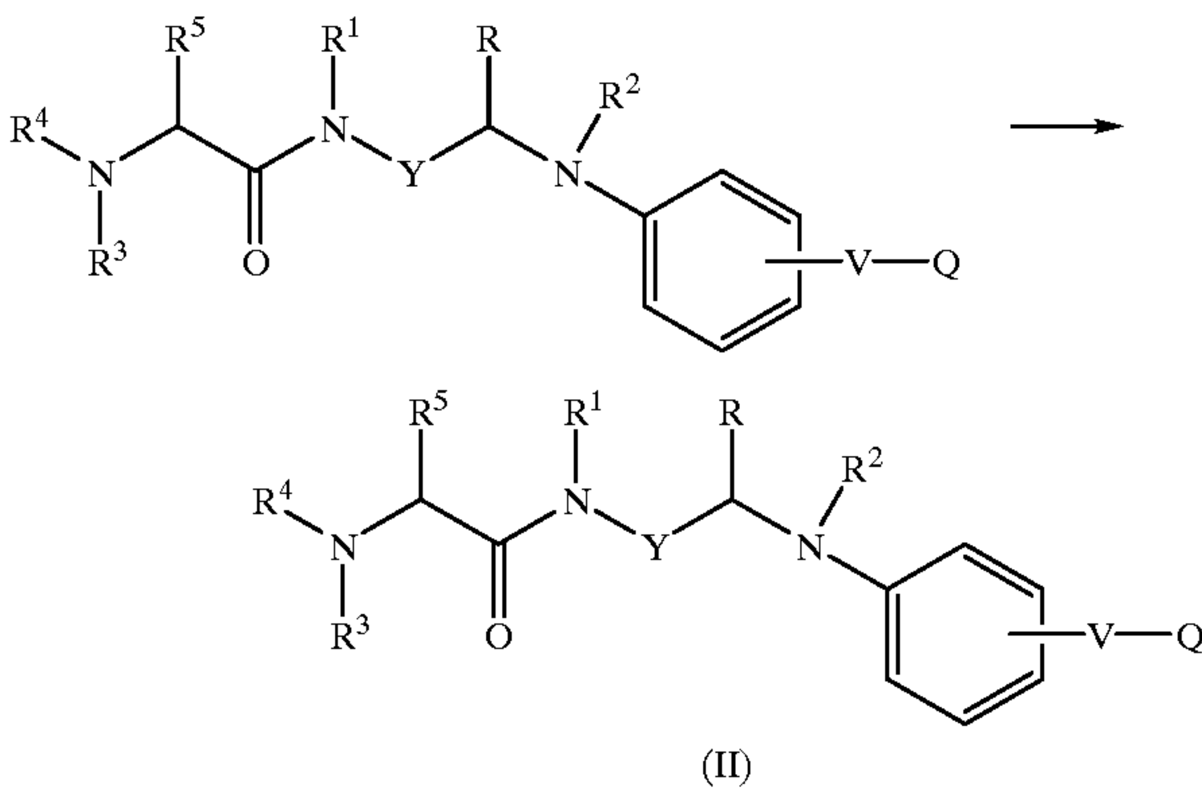
Scheme V
