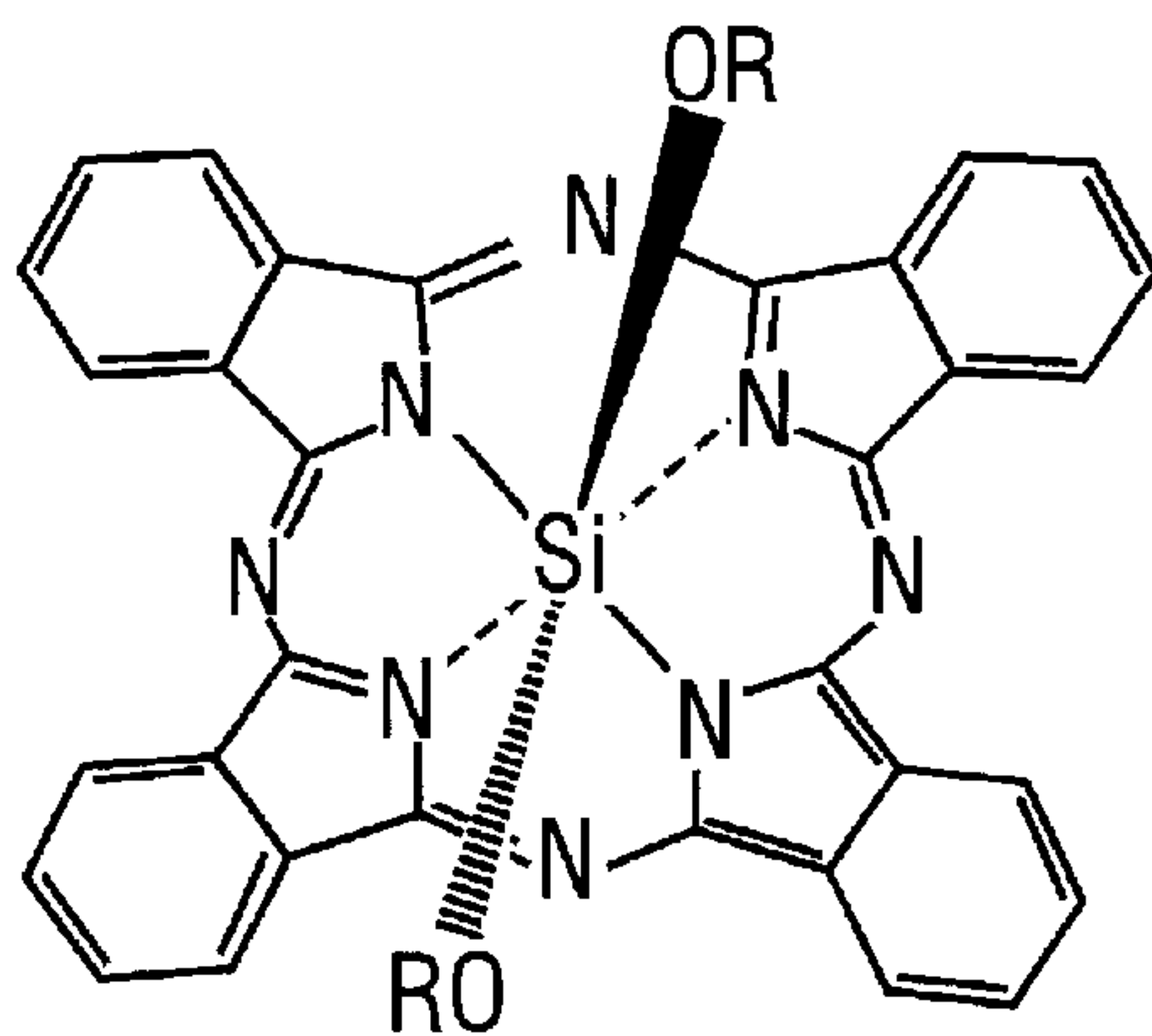
Silicon Phthalocyanine
