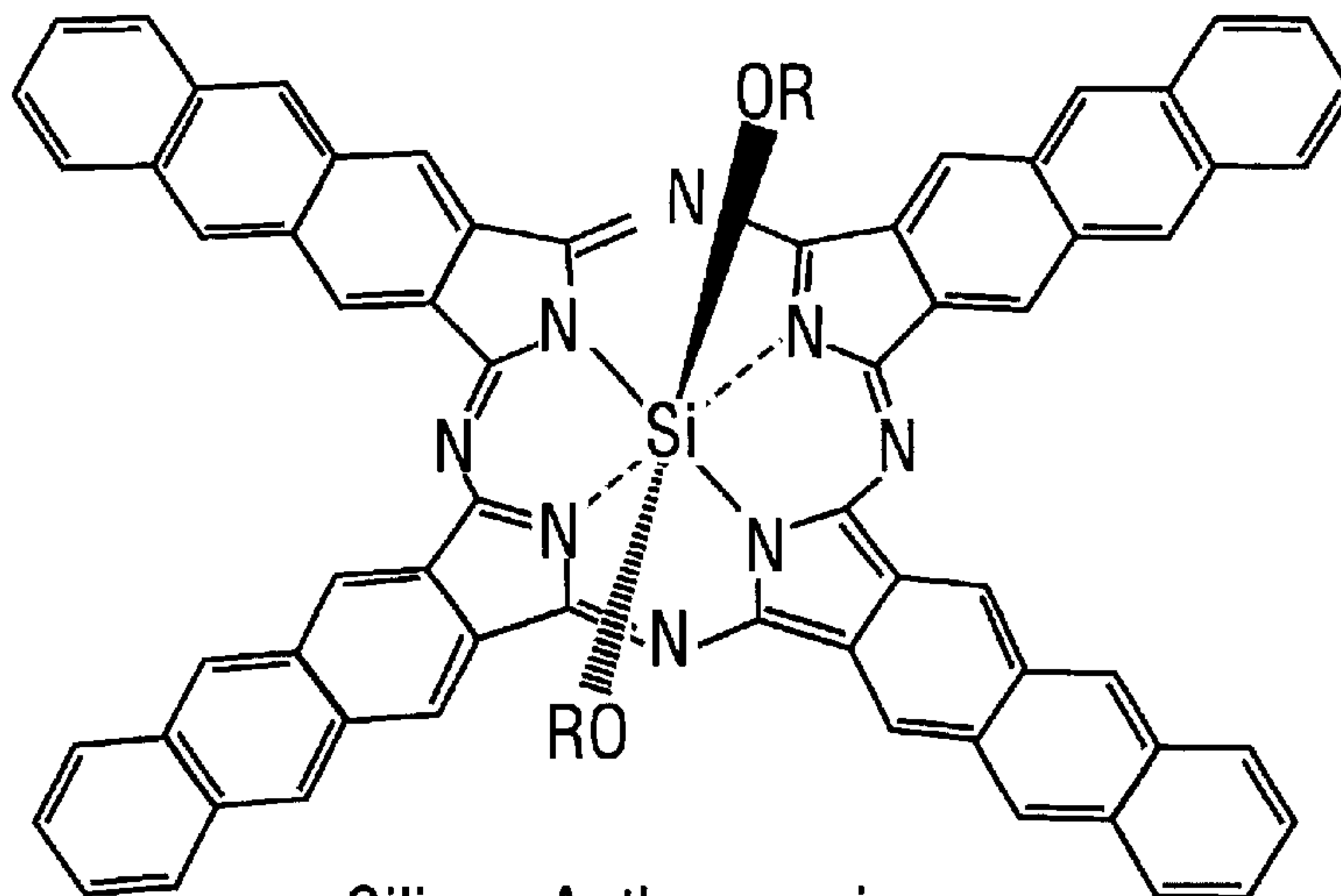
Silicon Anthracyanine
