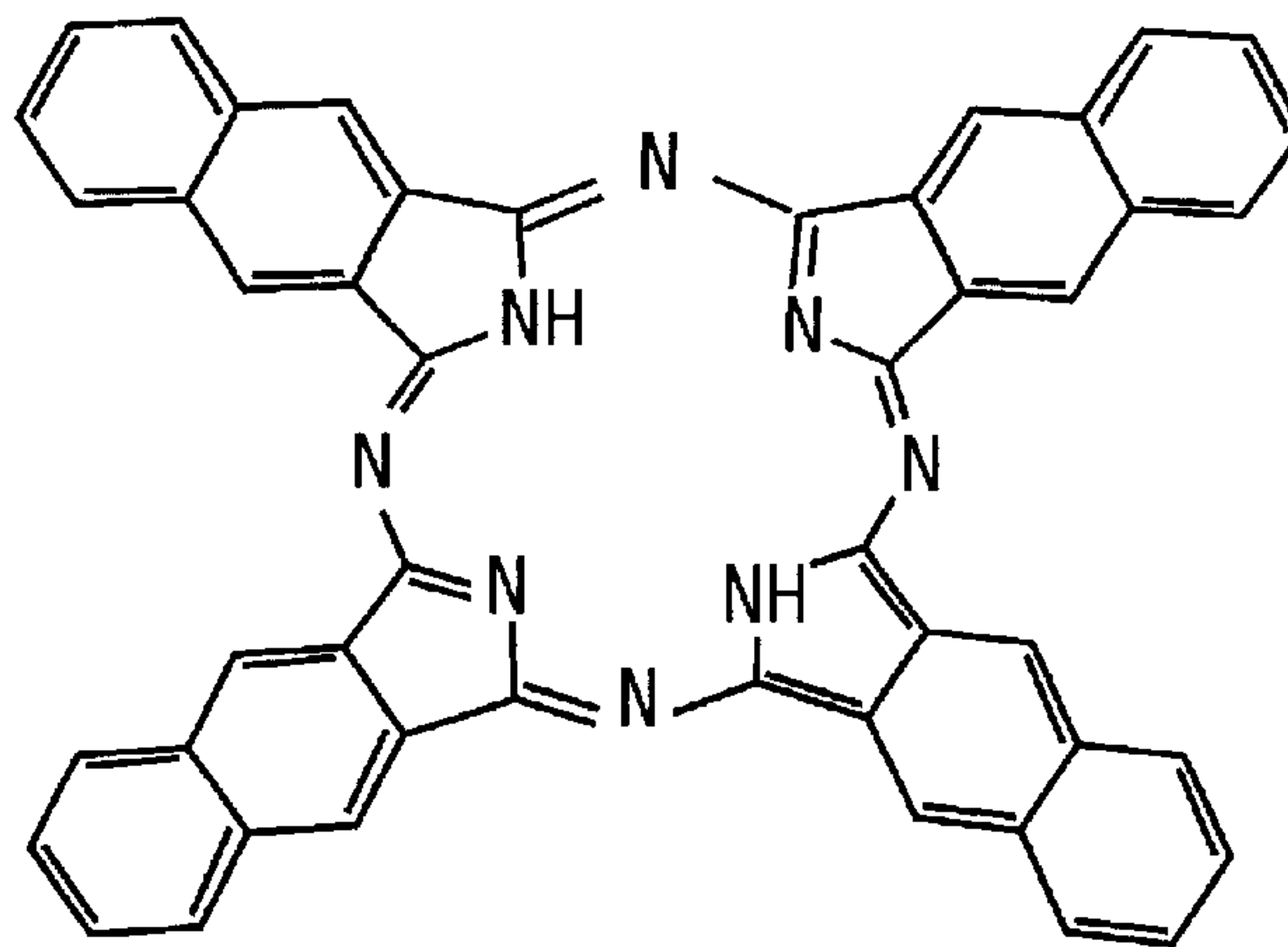
Naphthalocyanine
