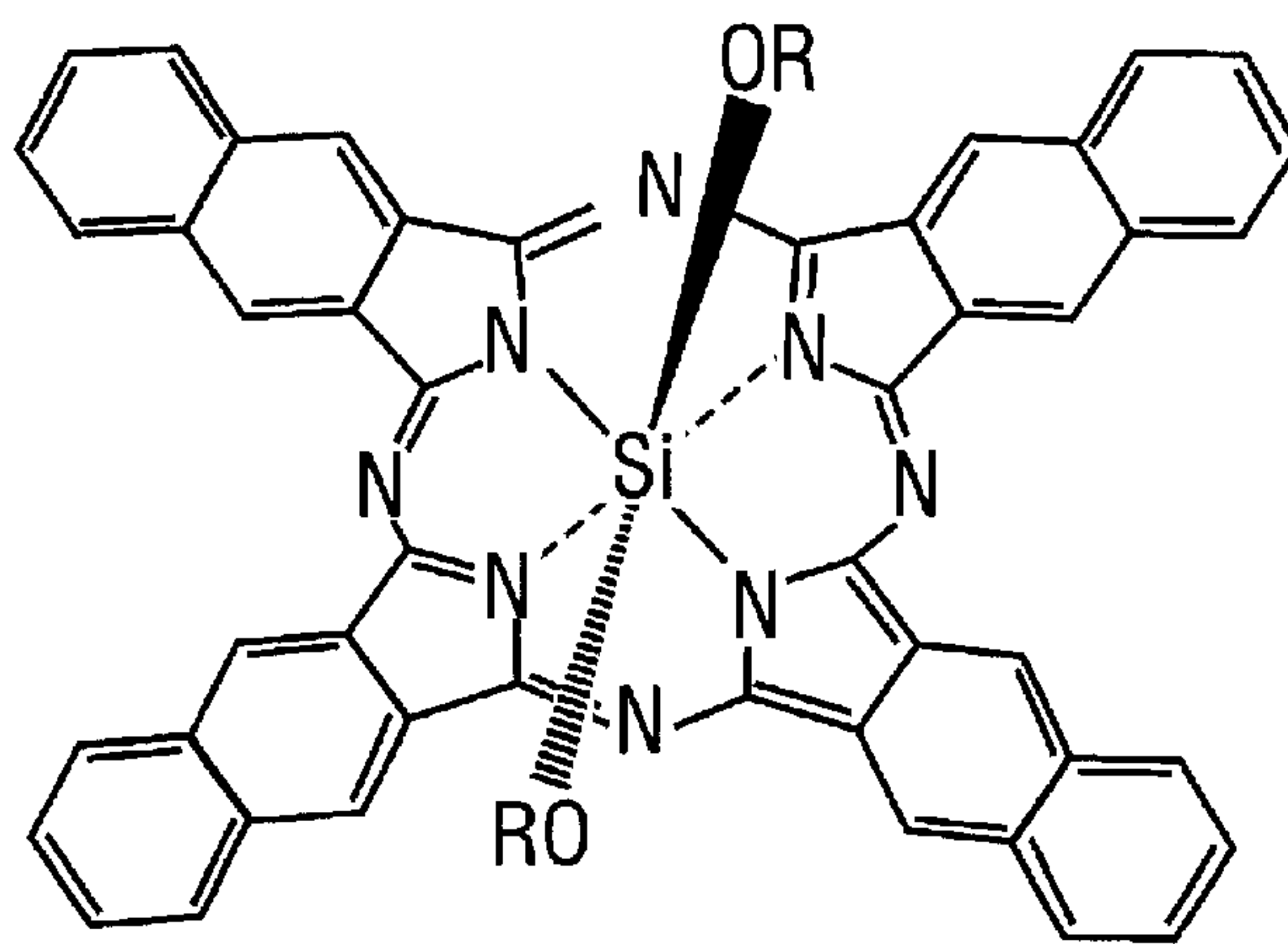
Silicon Phthalocyanine
