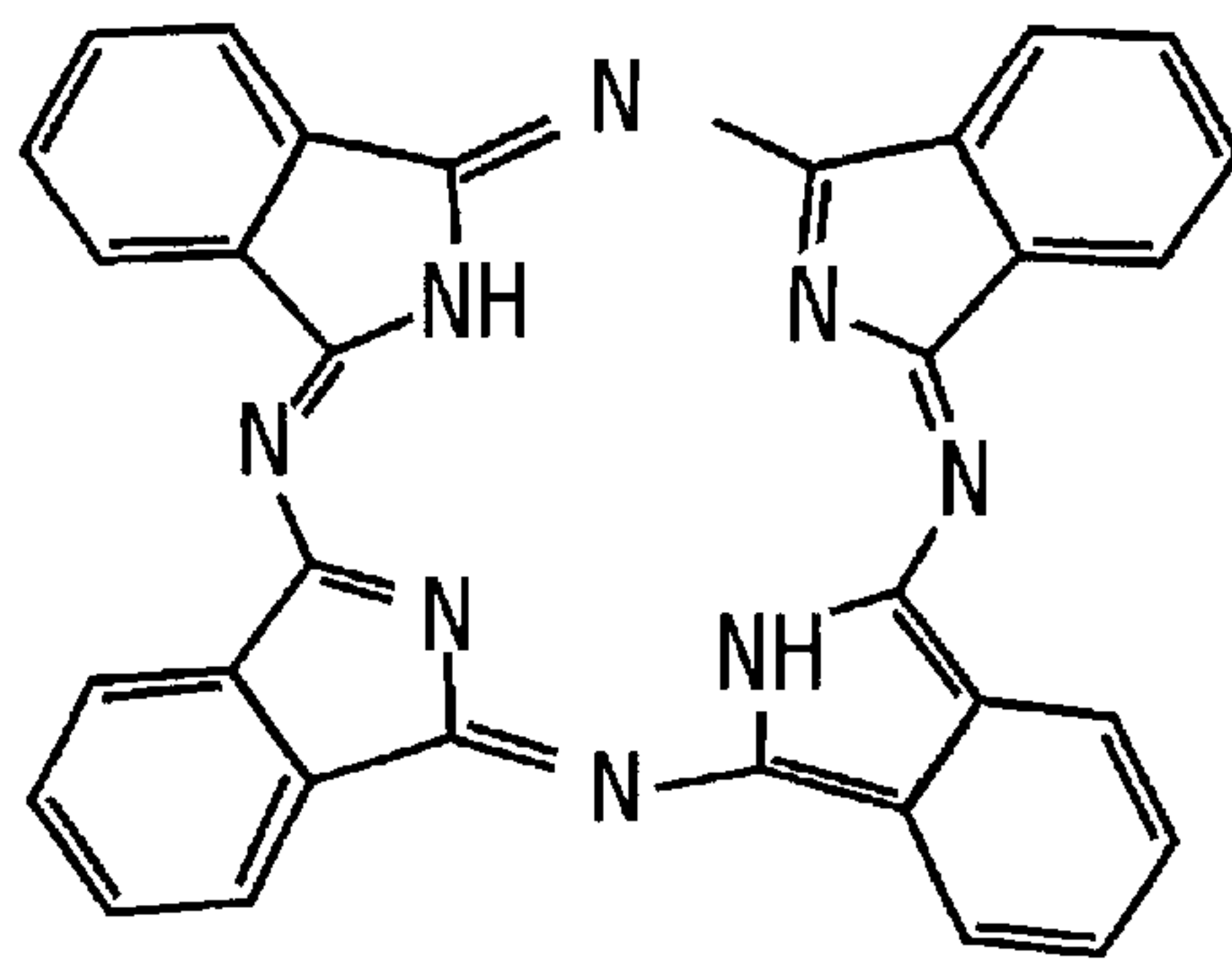
Phthalocyanine
