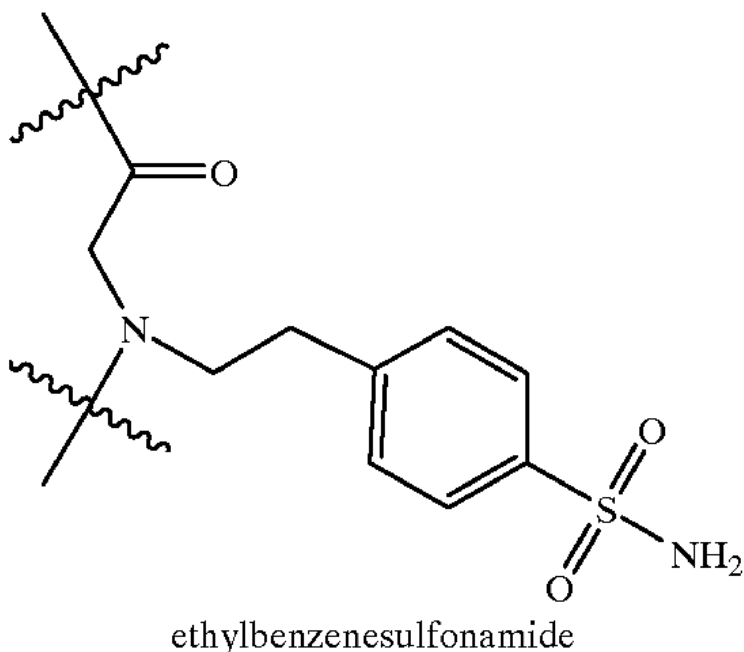
ethylbenzenesulfonamide
