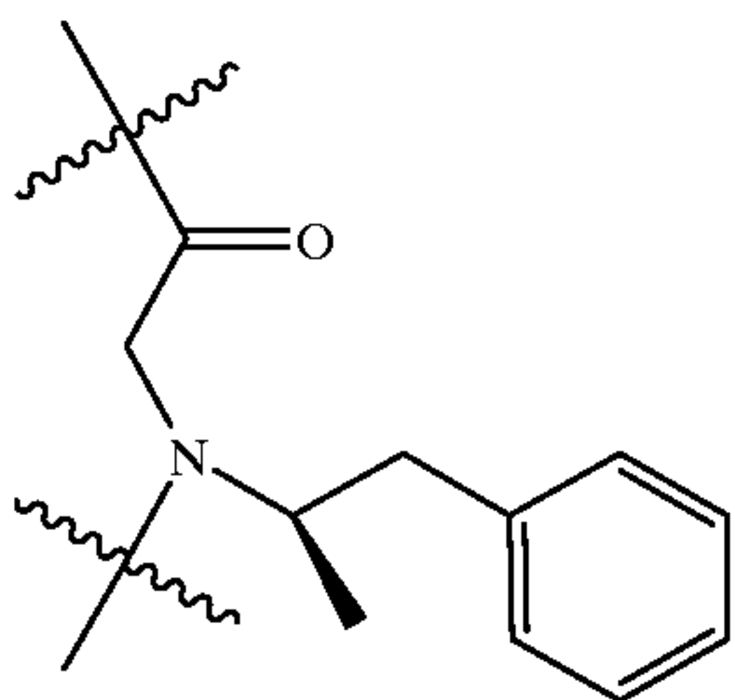
amphetamine
