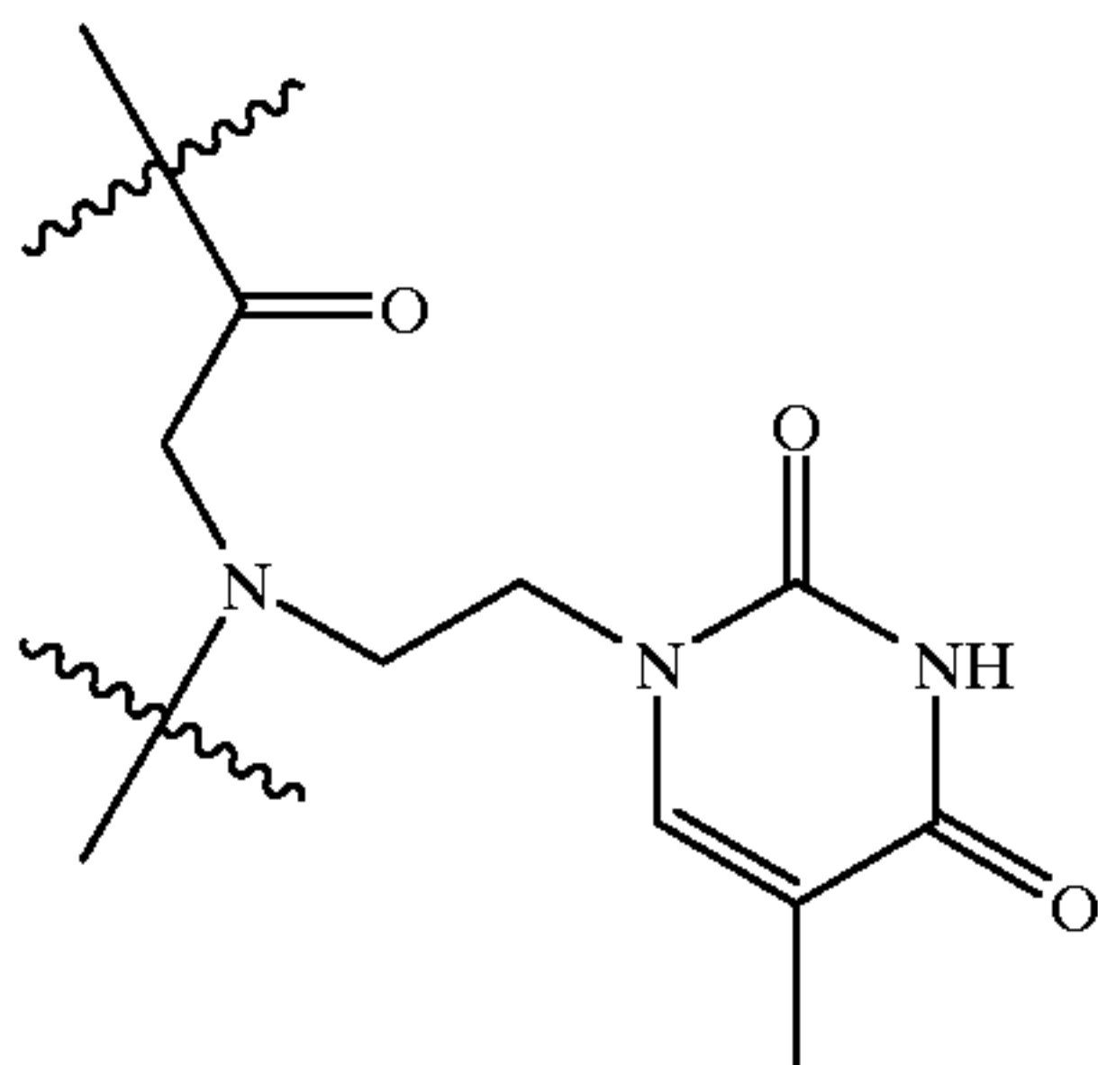
1-ethylthymine
