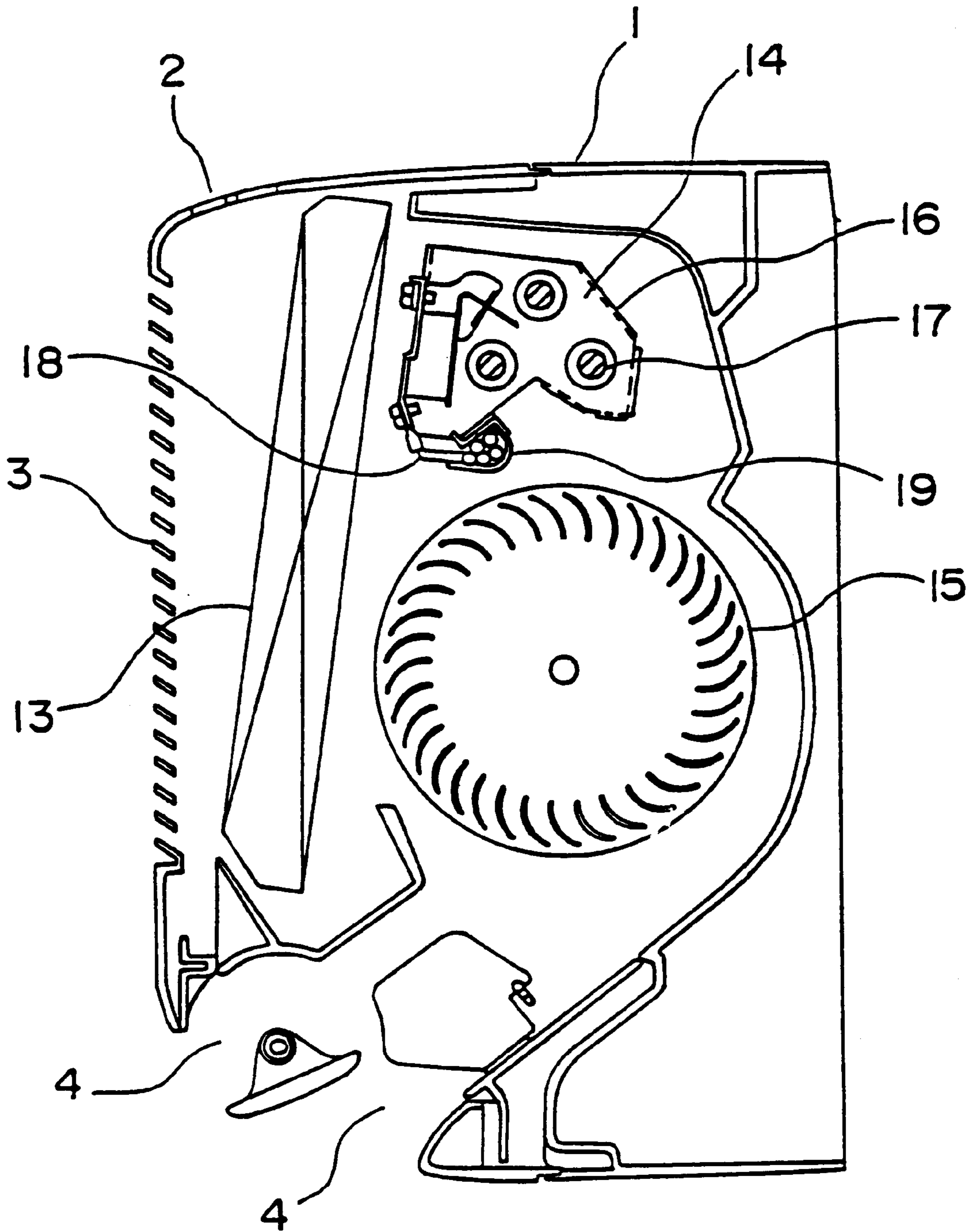
FIG. 11 PRIOR ART
