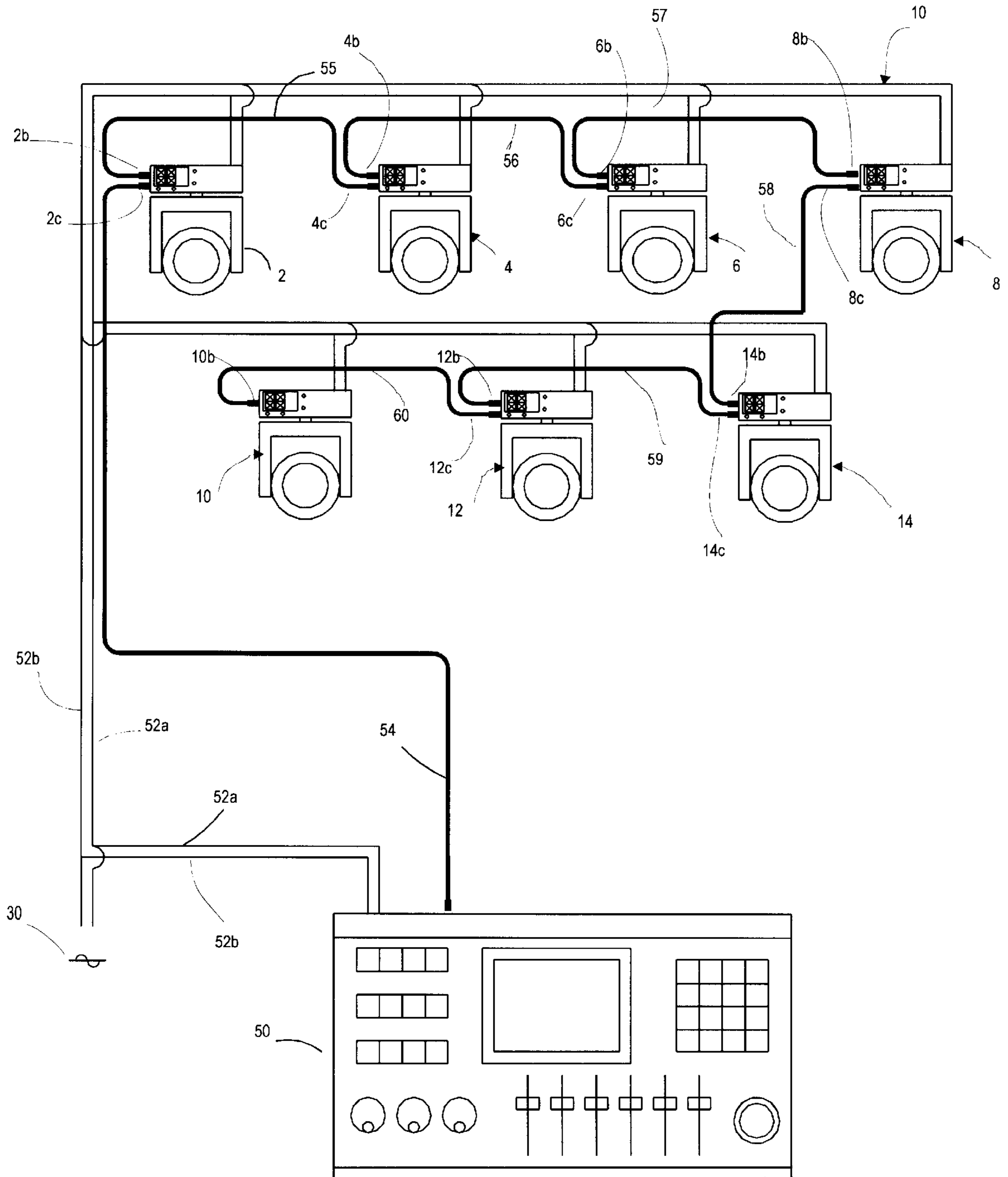
Fig. 1 (Prior Art)
