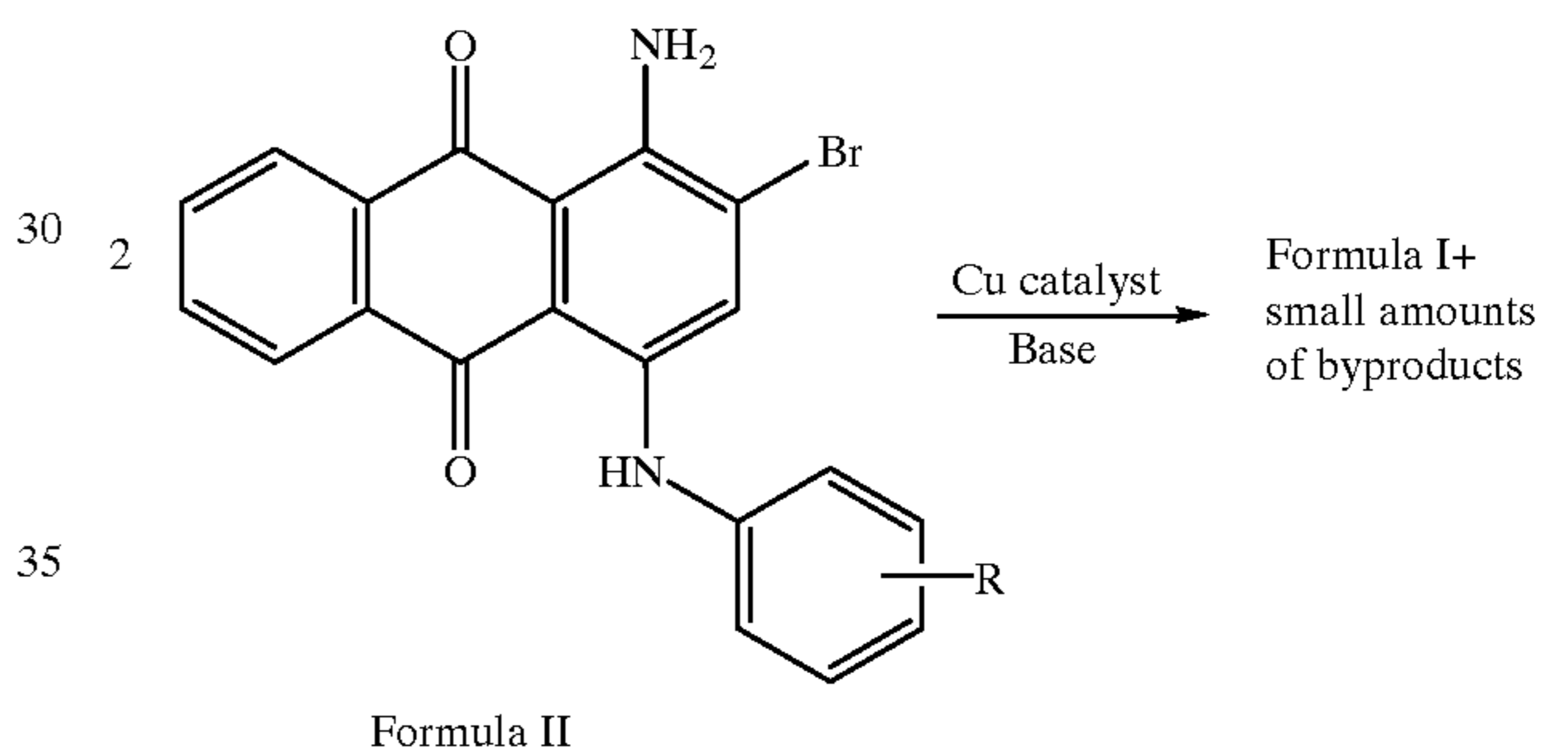
Scheme I
