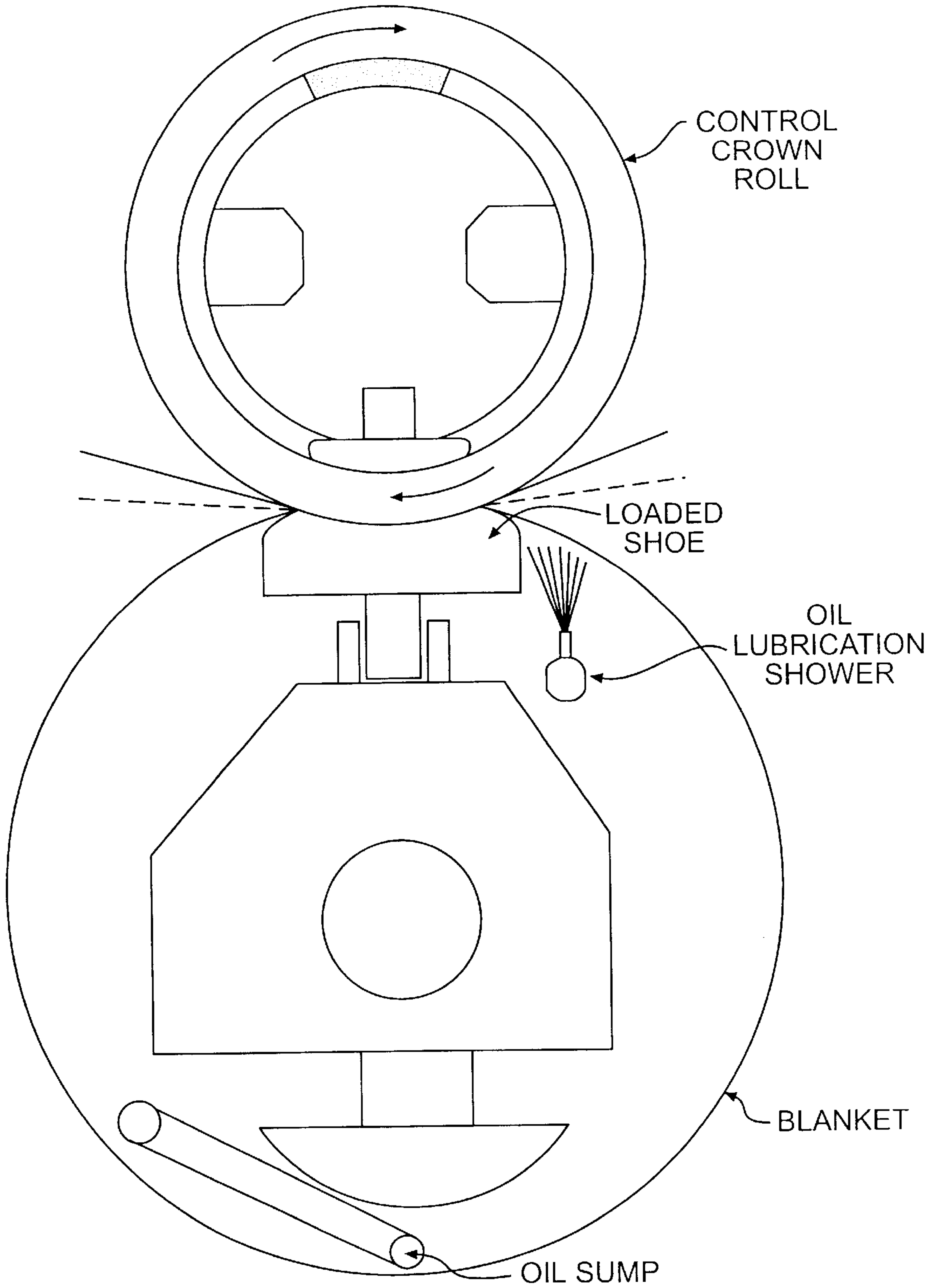
SIDE VIEW OF WIDE SHOE PRESS
