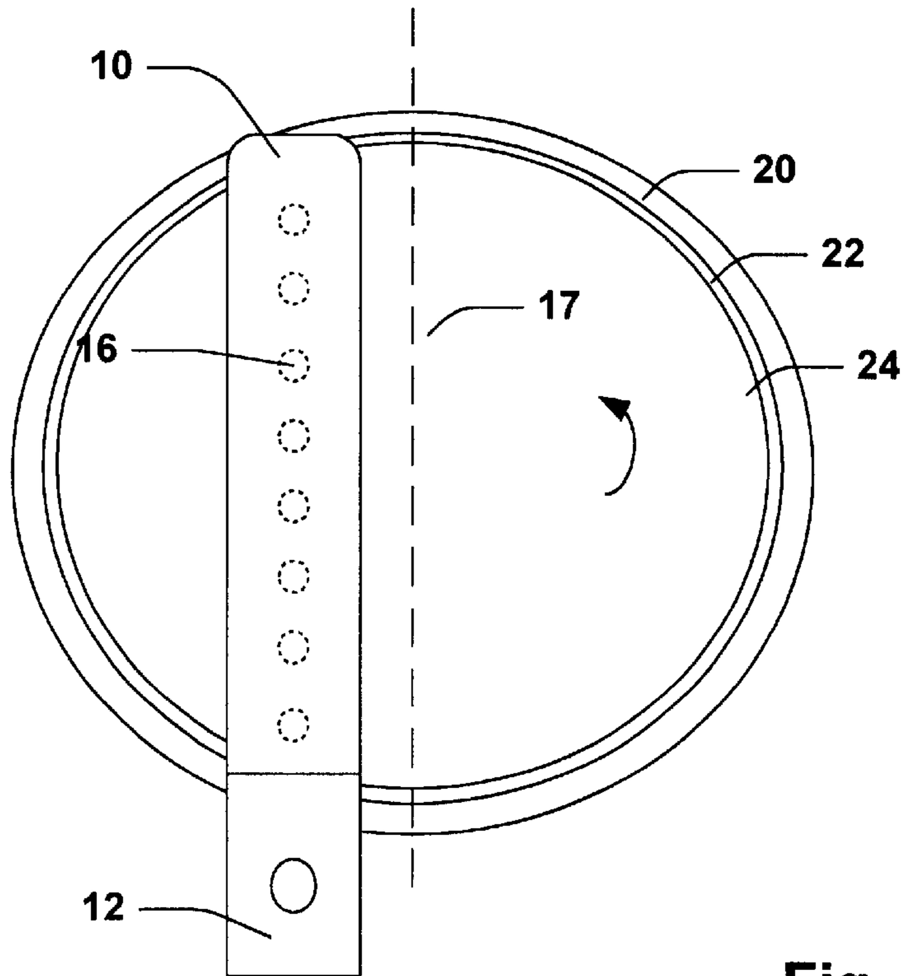
Fig. 1c Prior Art
