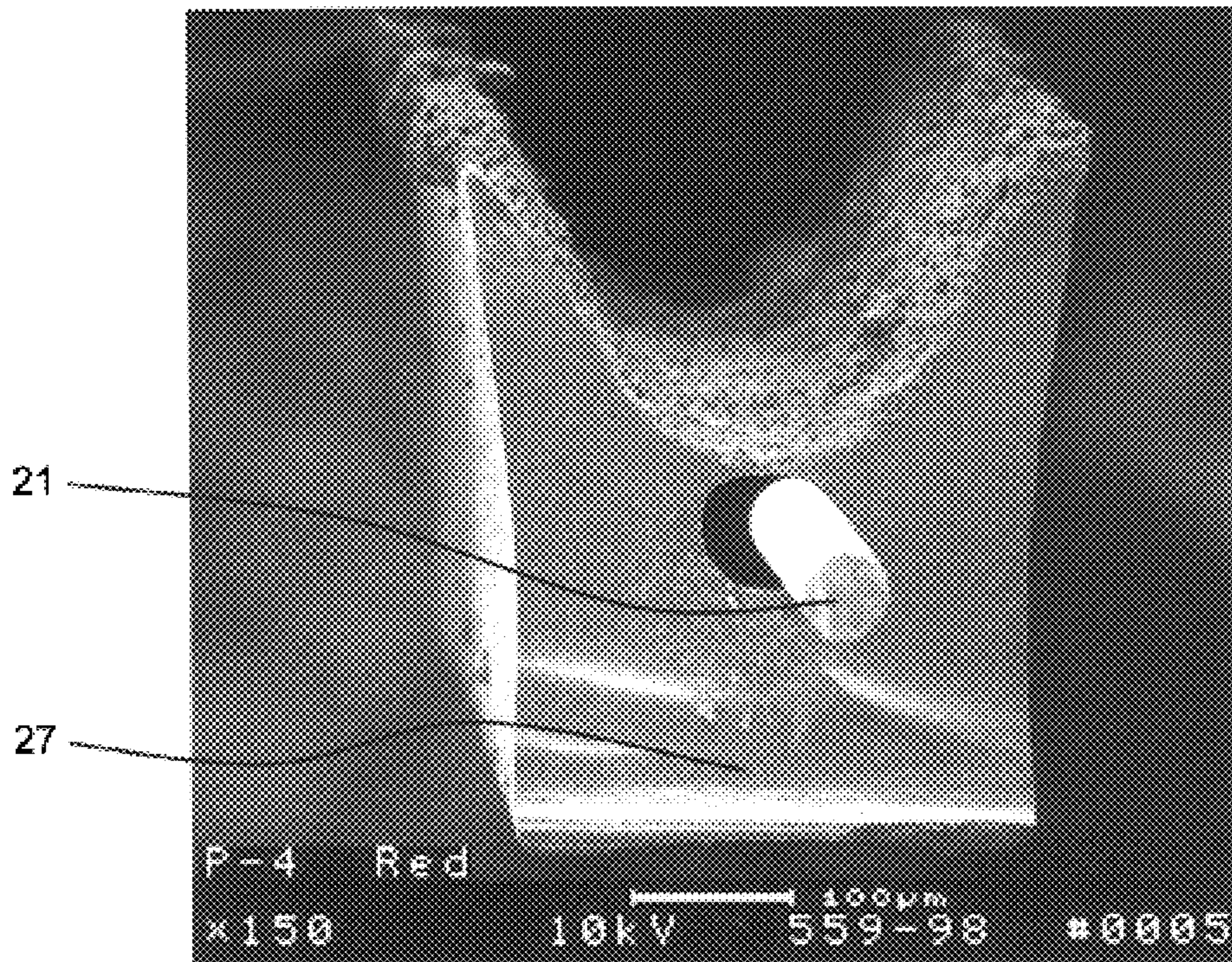
Figure 7A
