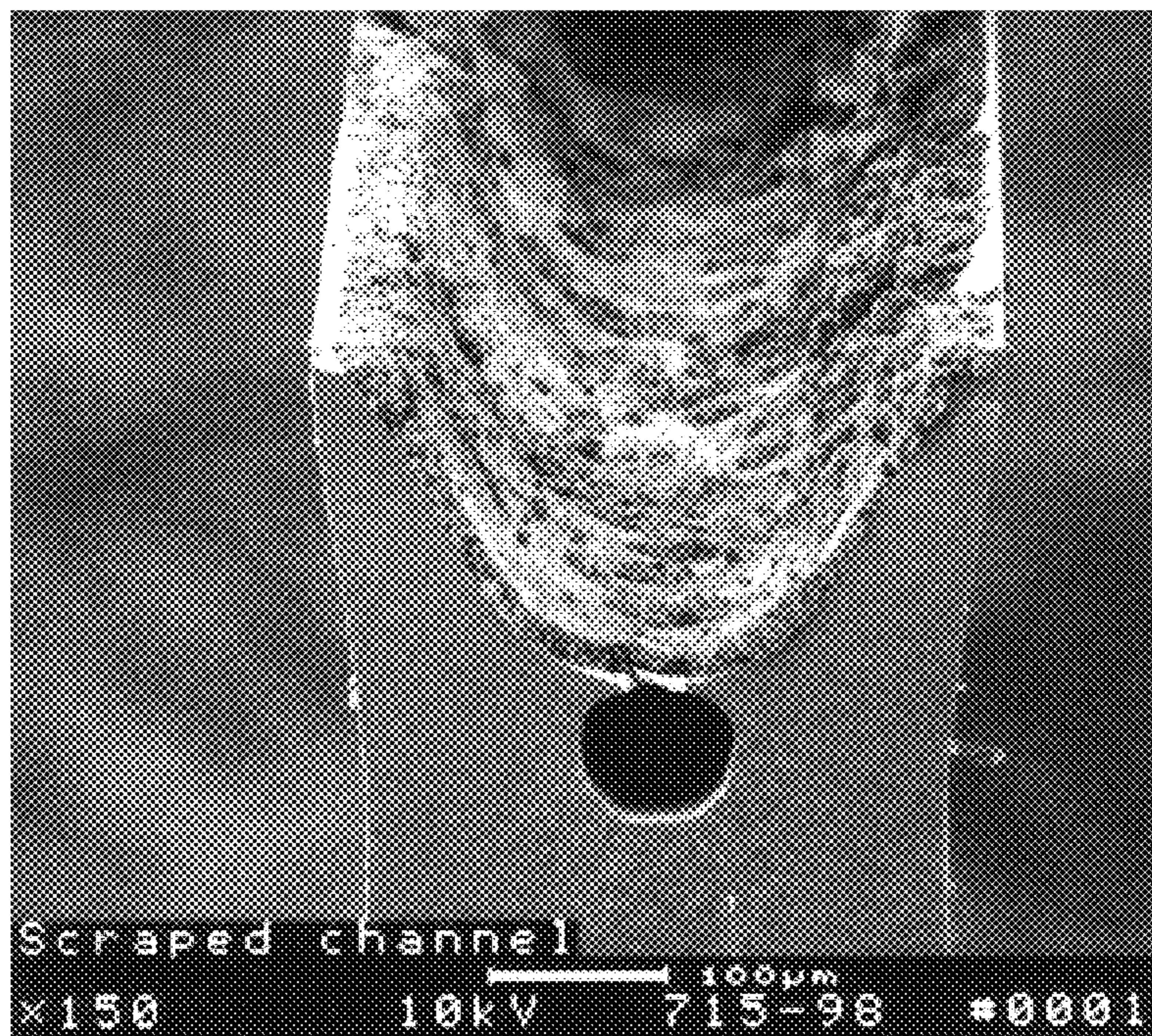
Figure 28B
