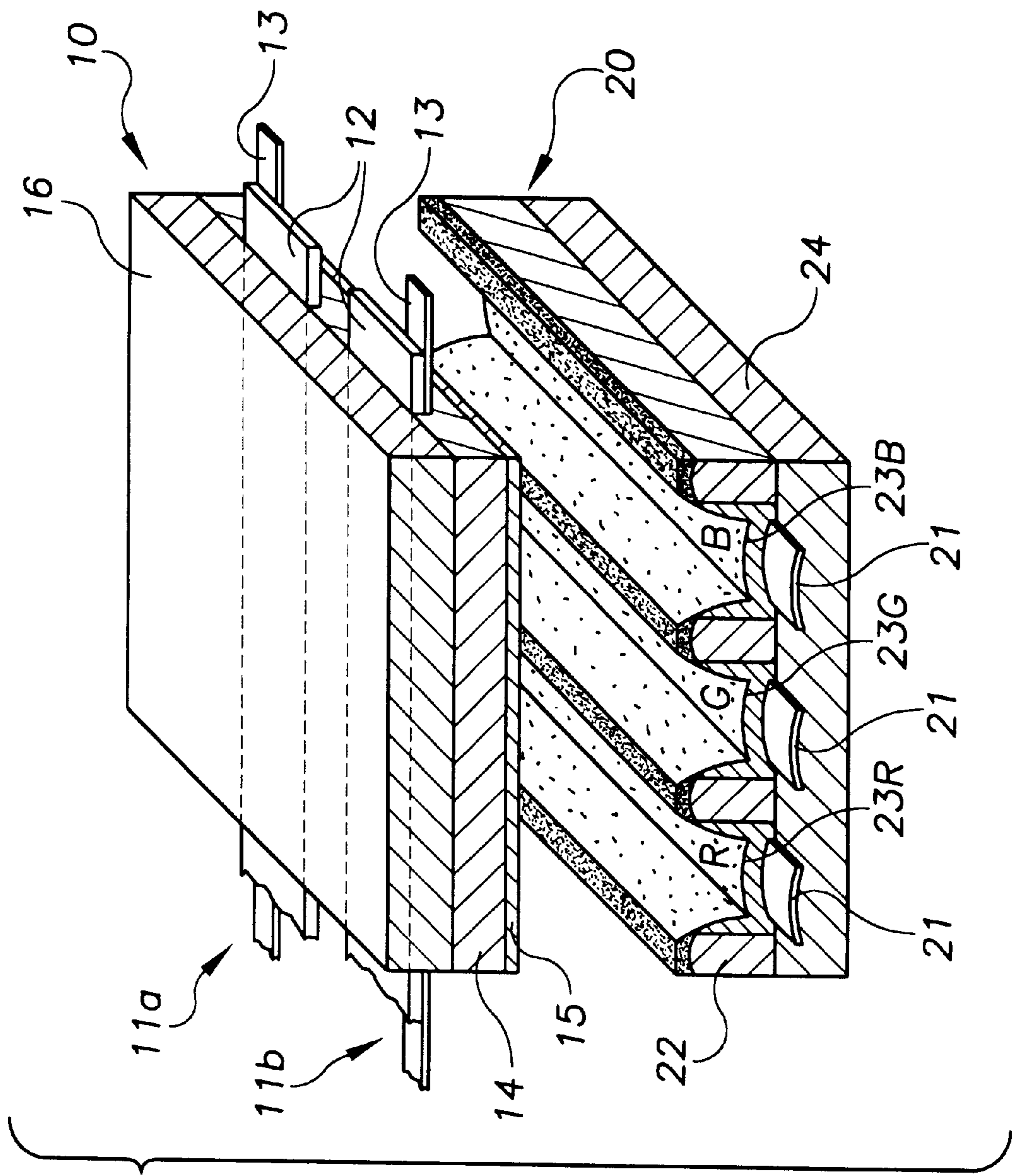
FIG. 1 PRIOR ART
