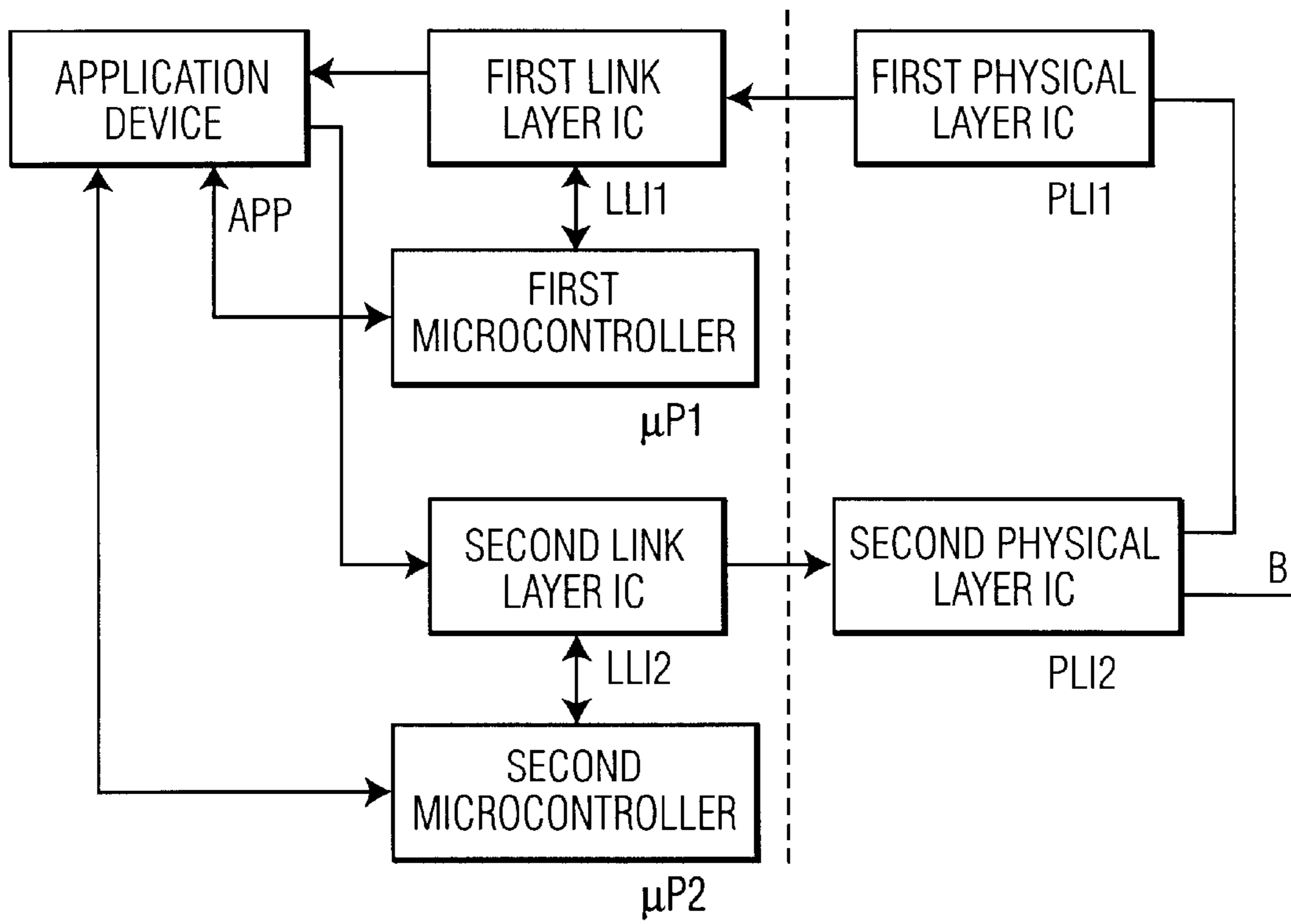
FIG. 1 PRIOR ART
