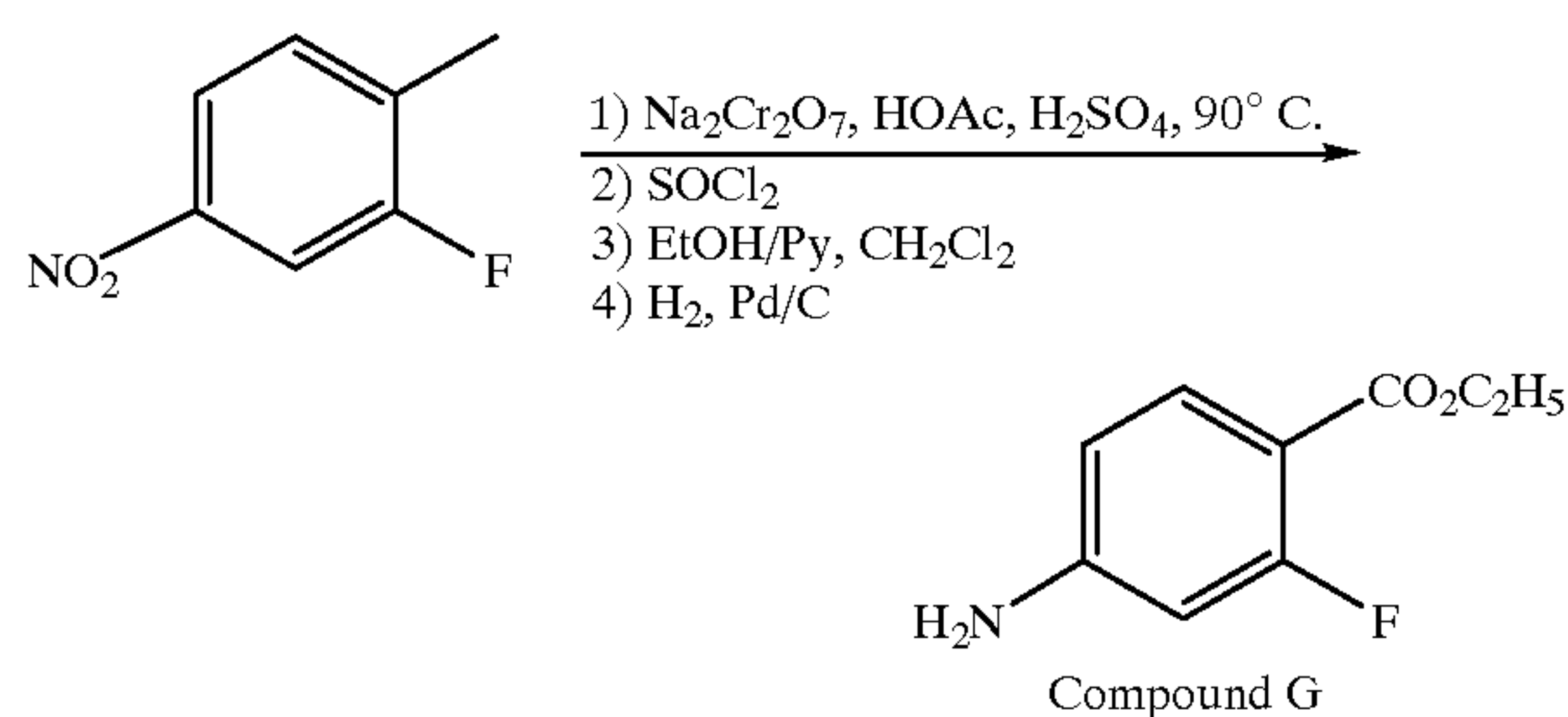
Reaction Scheme 2
