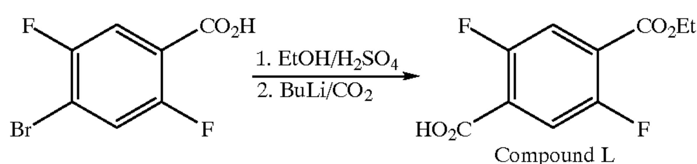
Reaction Scheme 4
