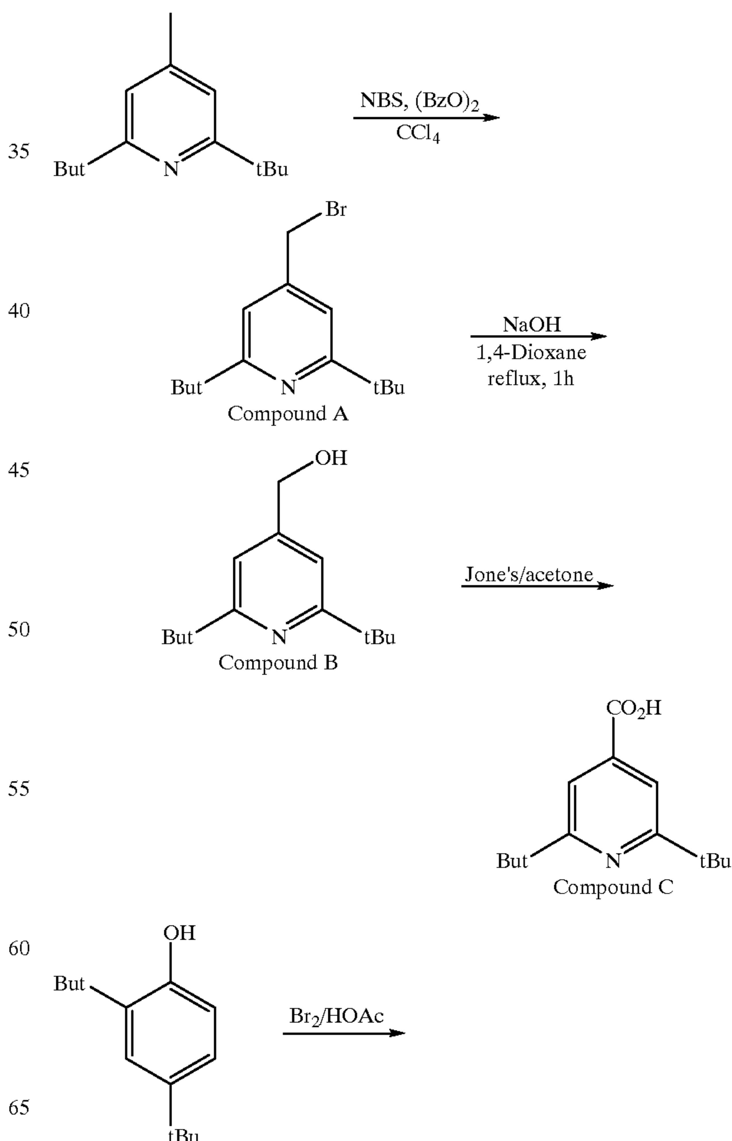
Reaction Scheme 1
