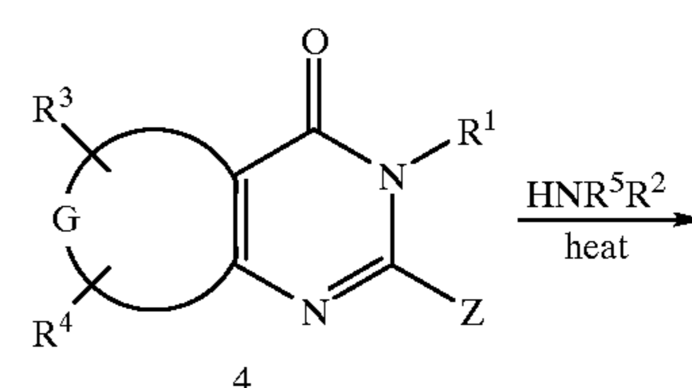
Scheme 5
