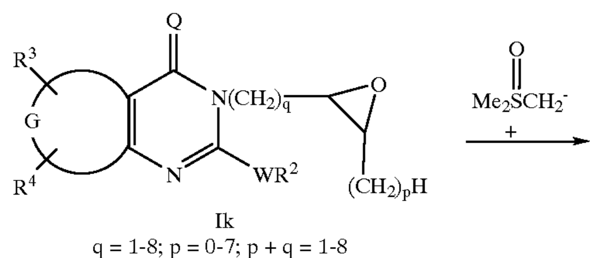
Scheme 12
