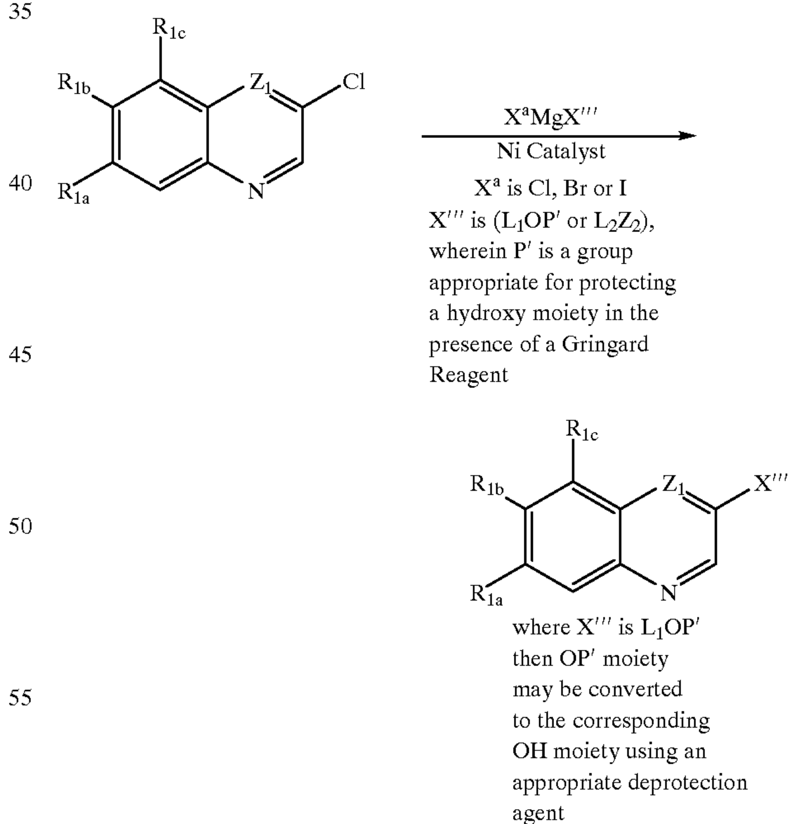
Scheme IX
