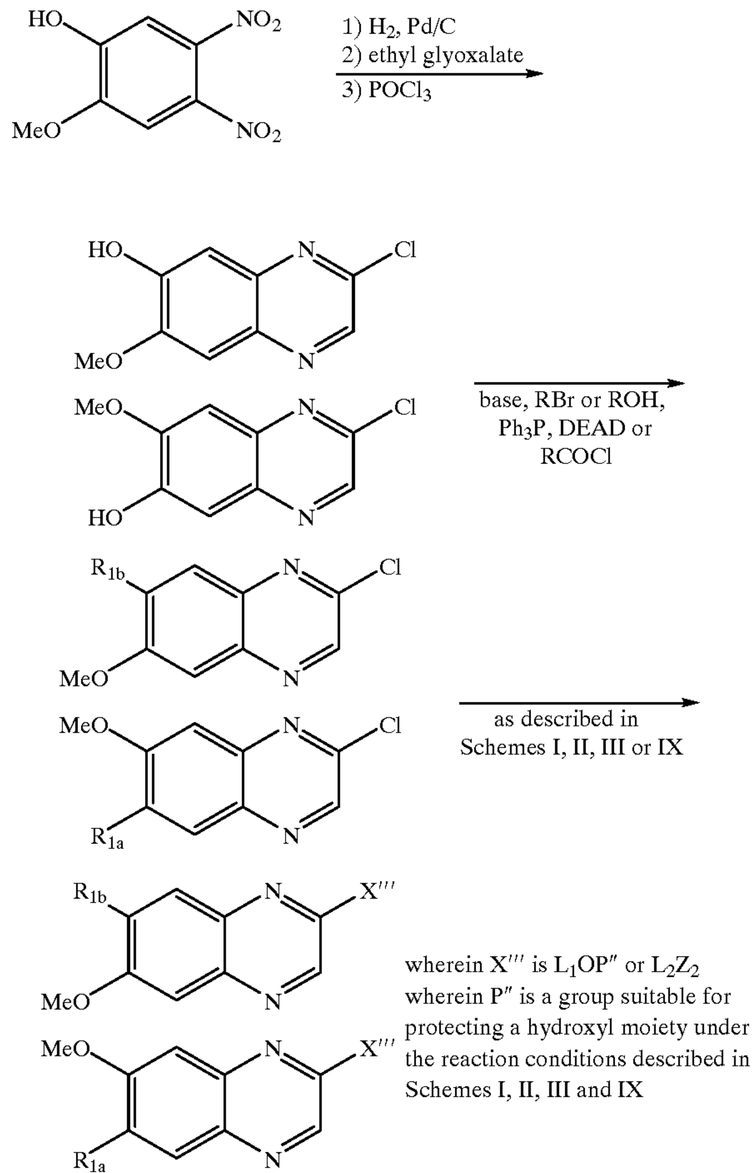
Scheme VII
