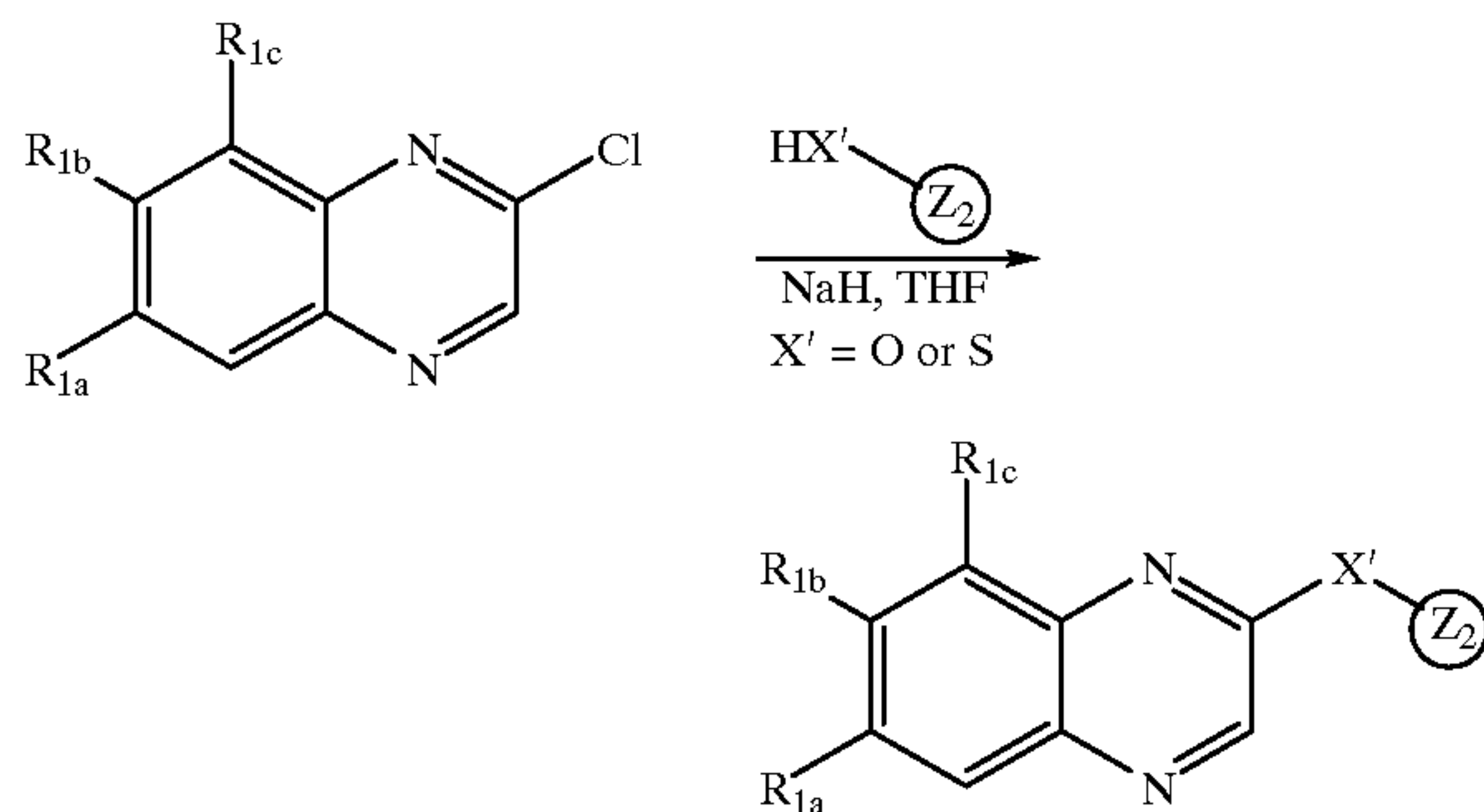
Scheme II
