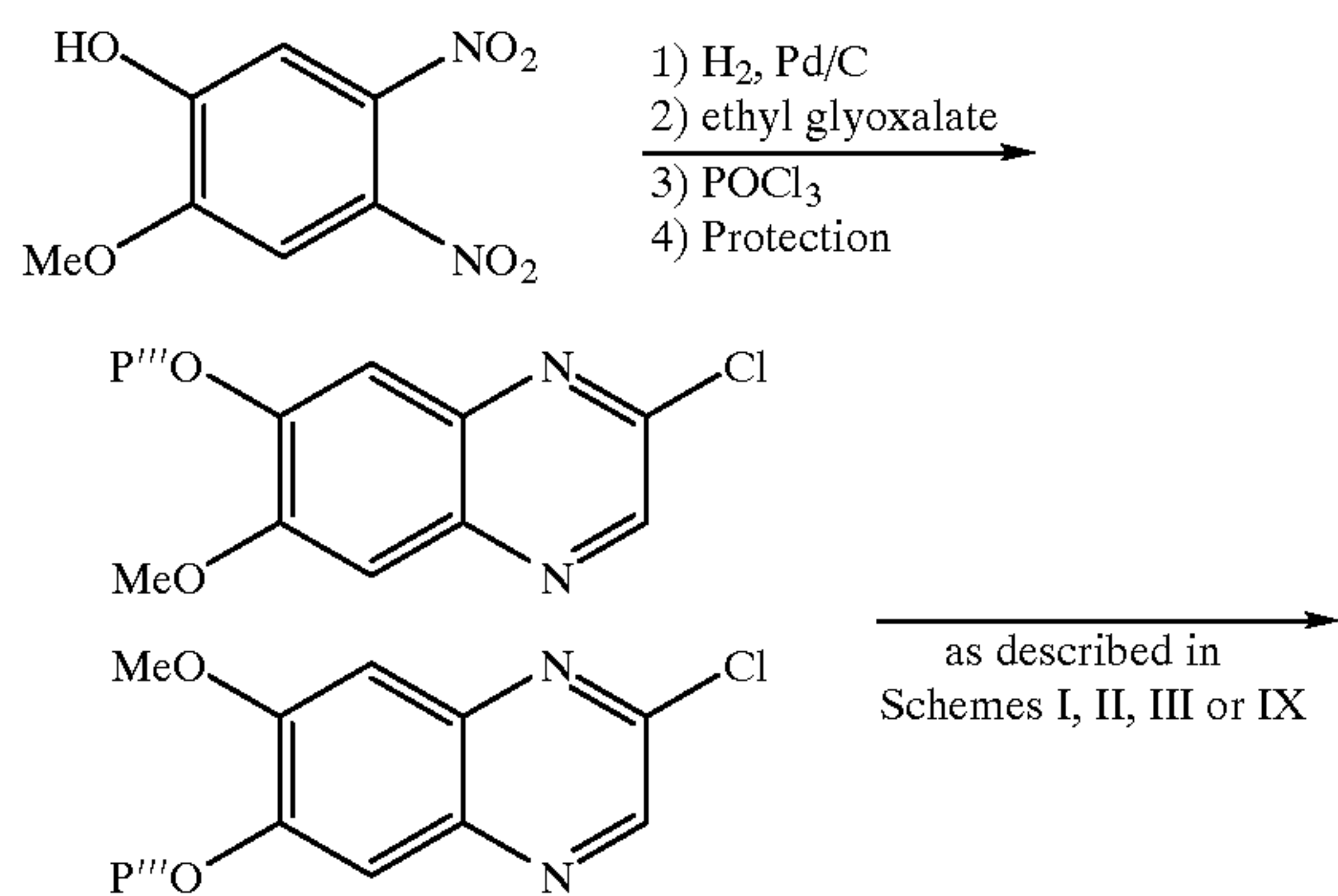
Scheme VIII
