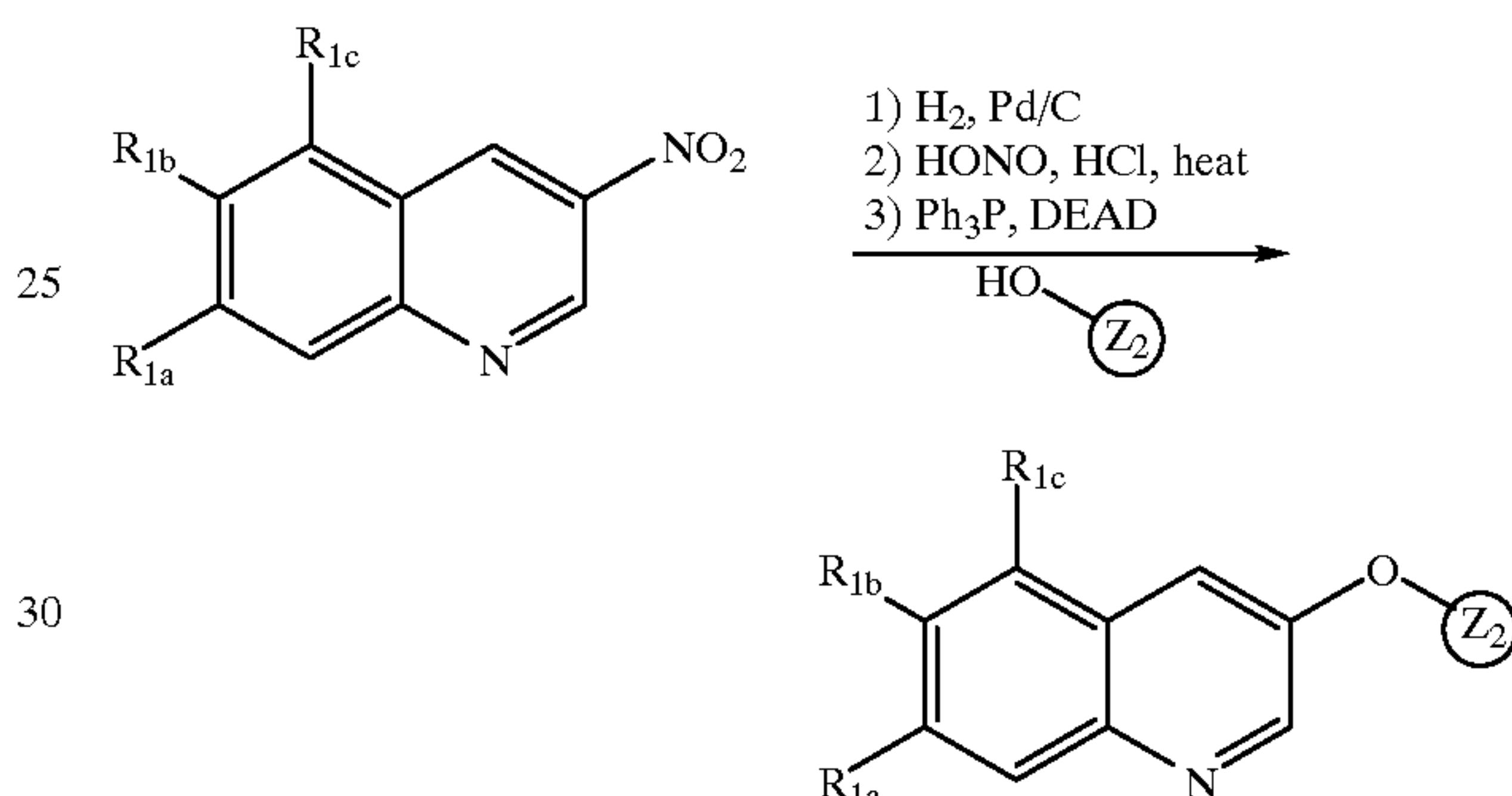
Scheme V
