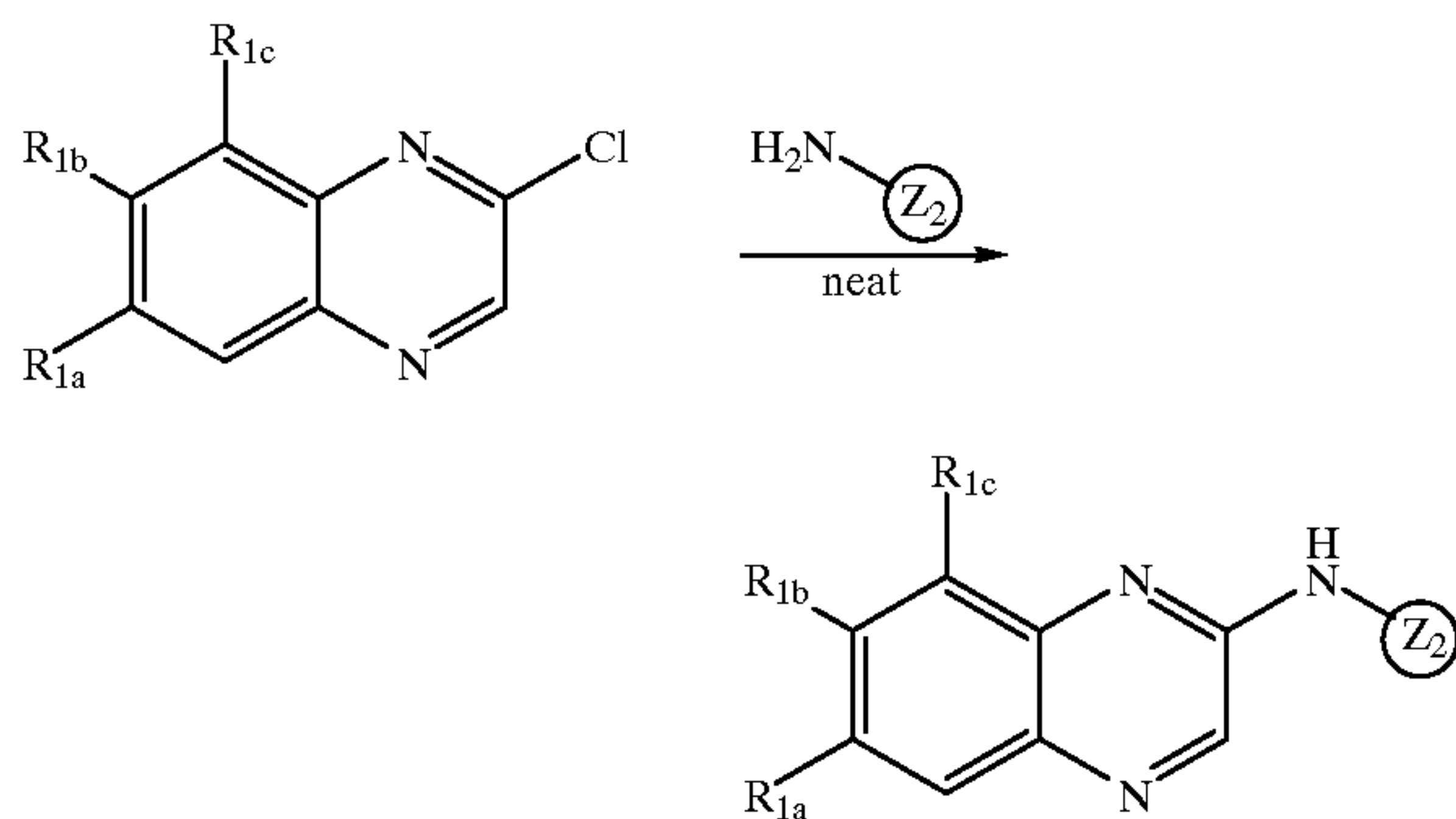
Scheme I
