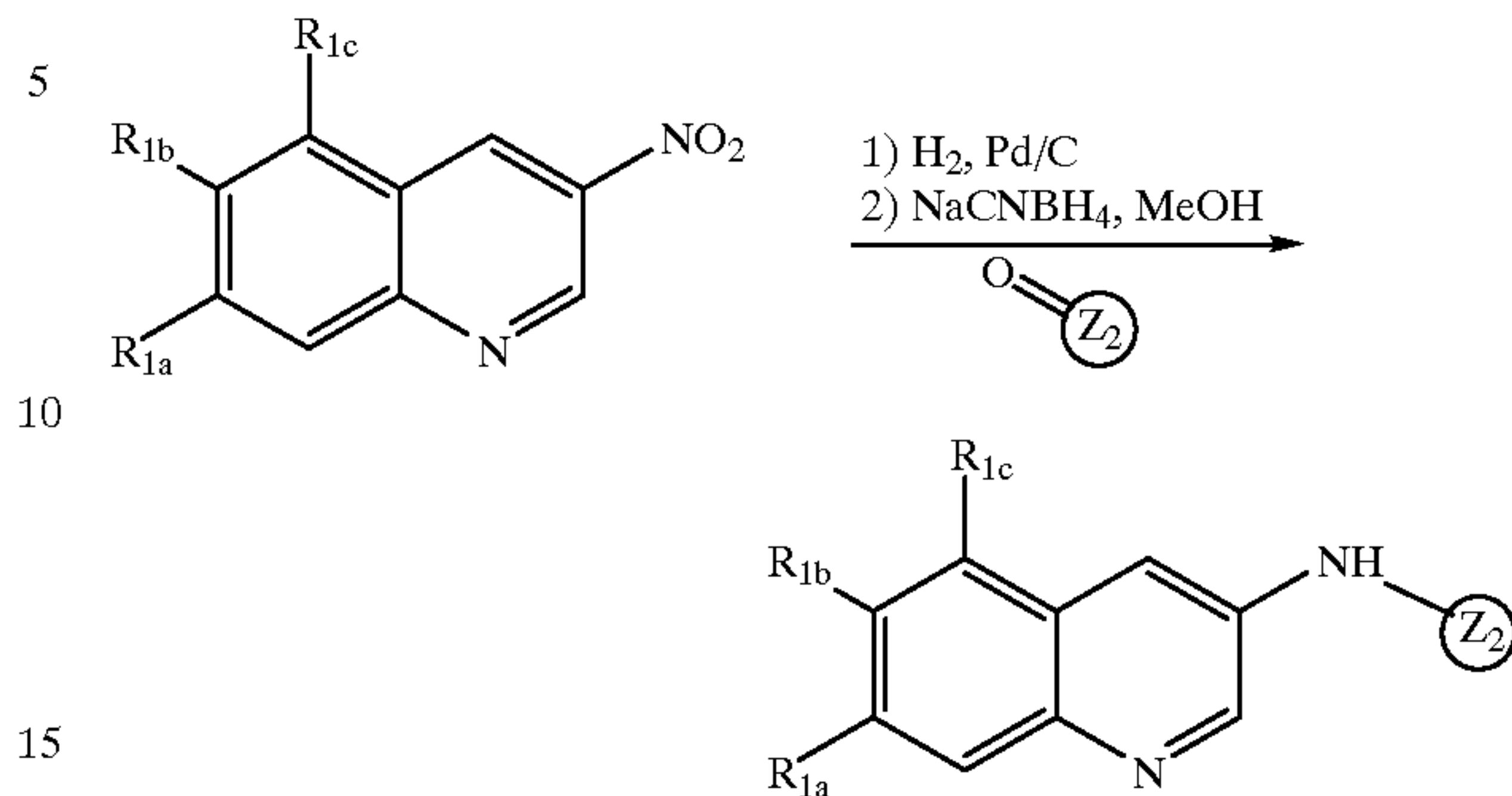
Scheme IV
