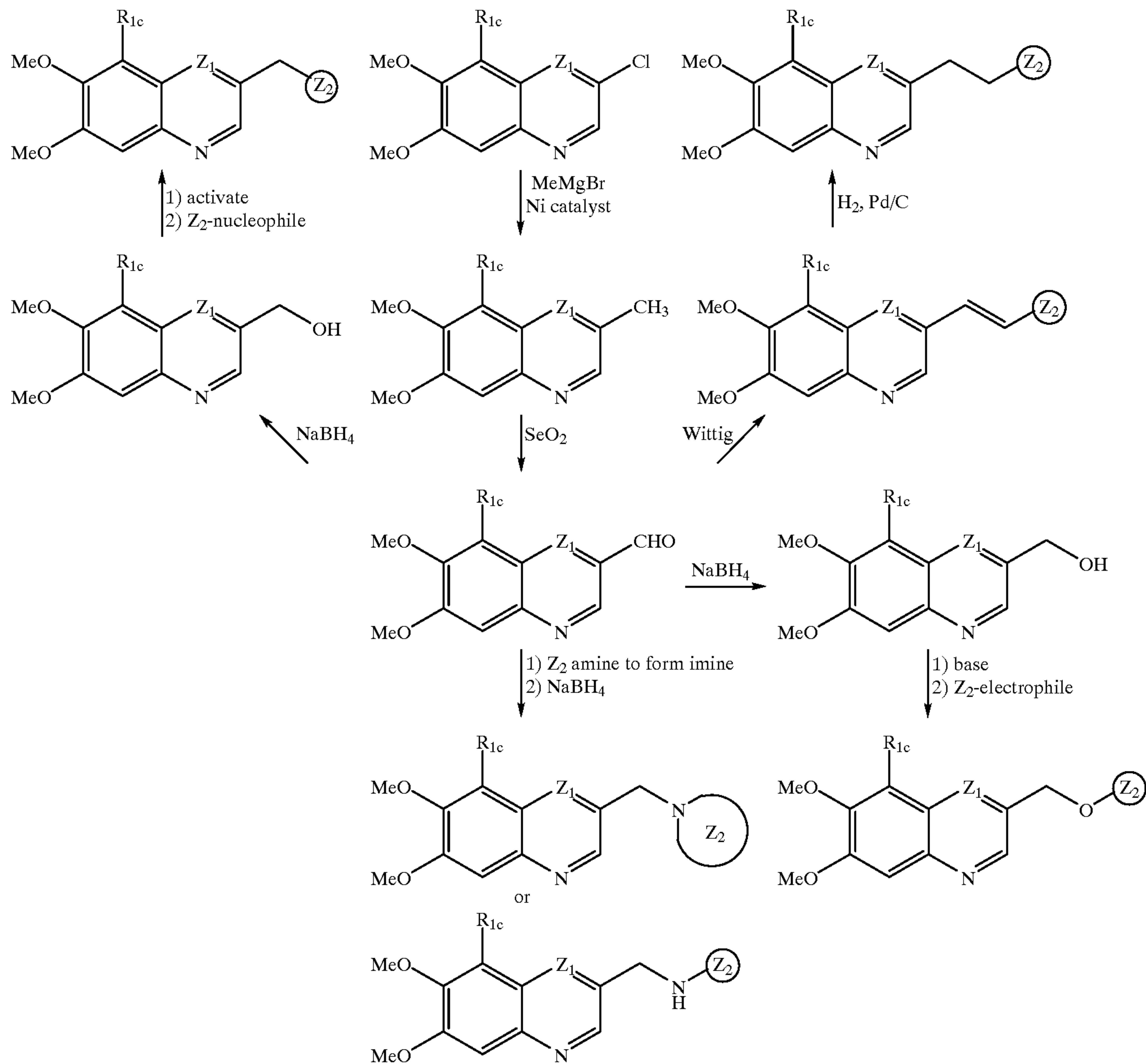
Scheme X
