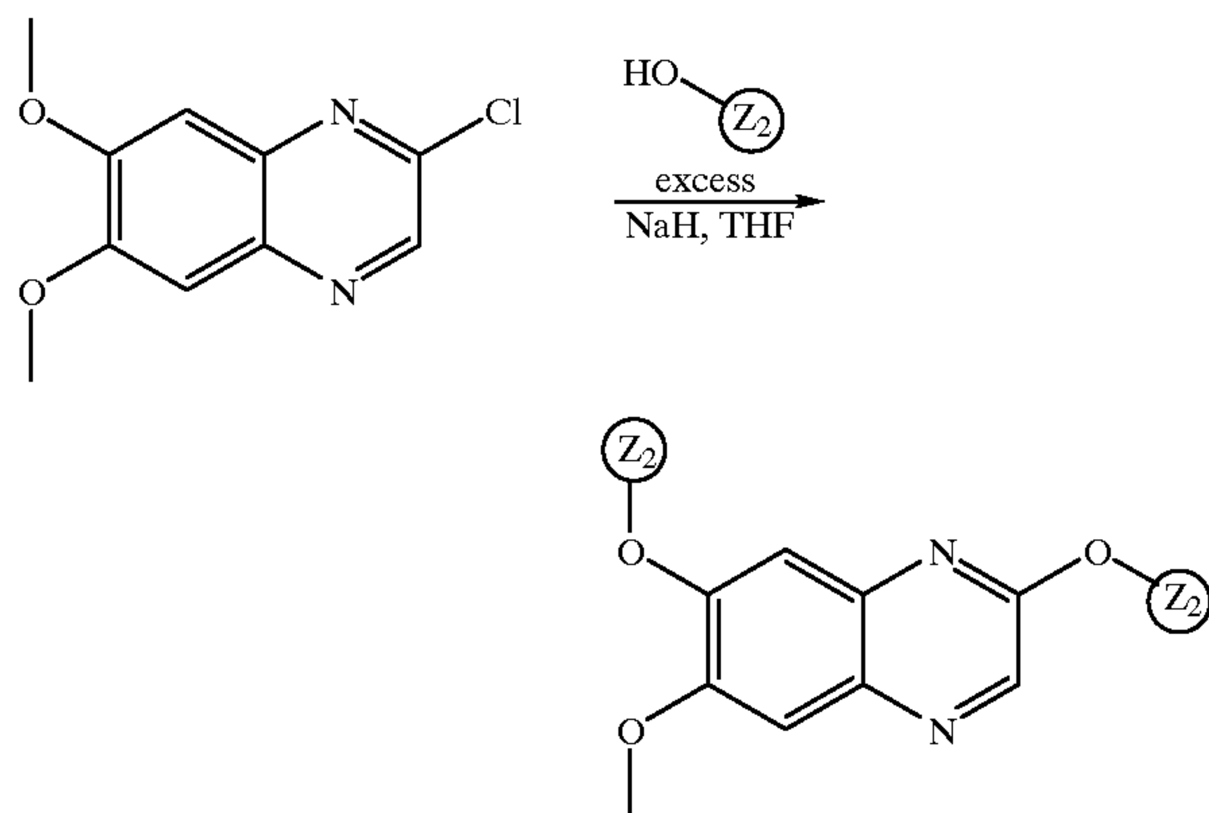
Scheme III
