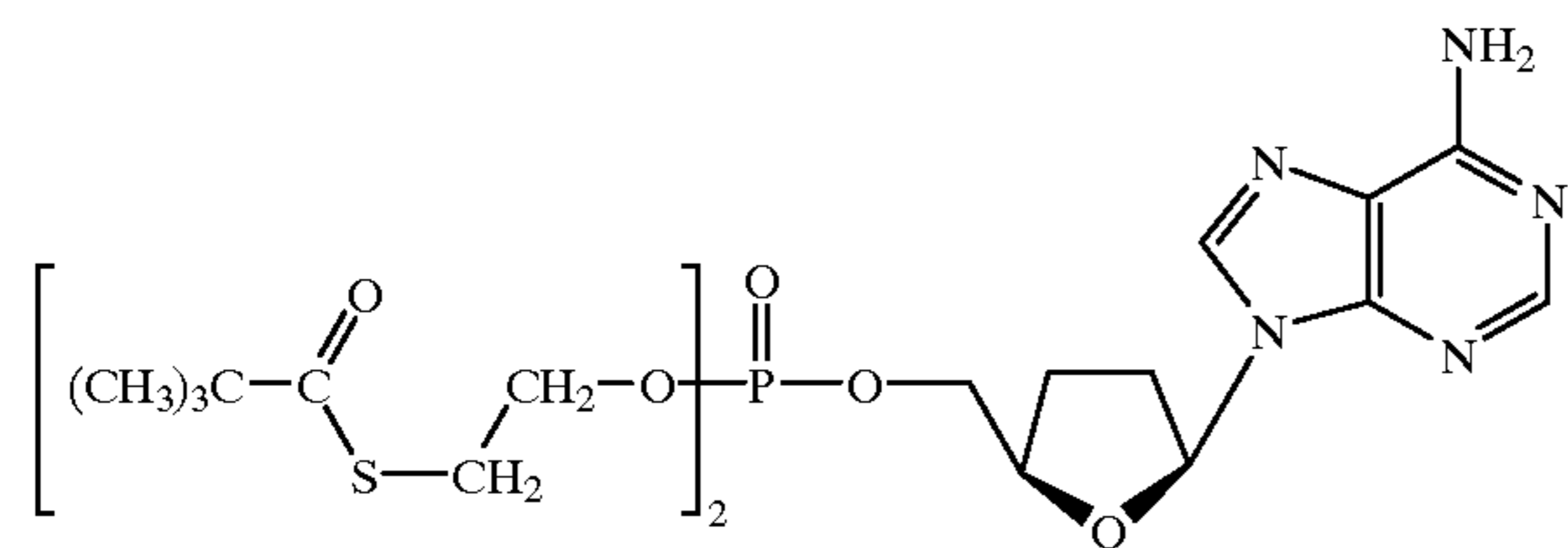
Bis(SATE) \beta -L-ddAMP
