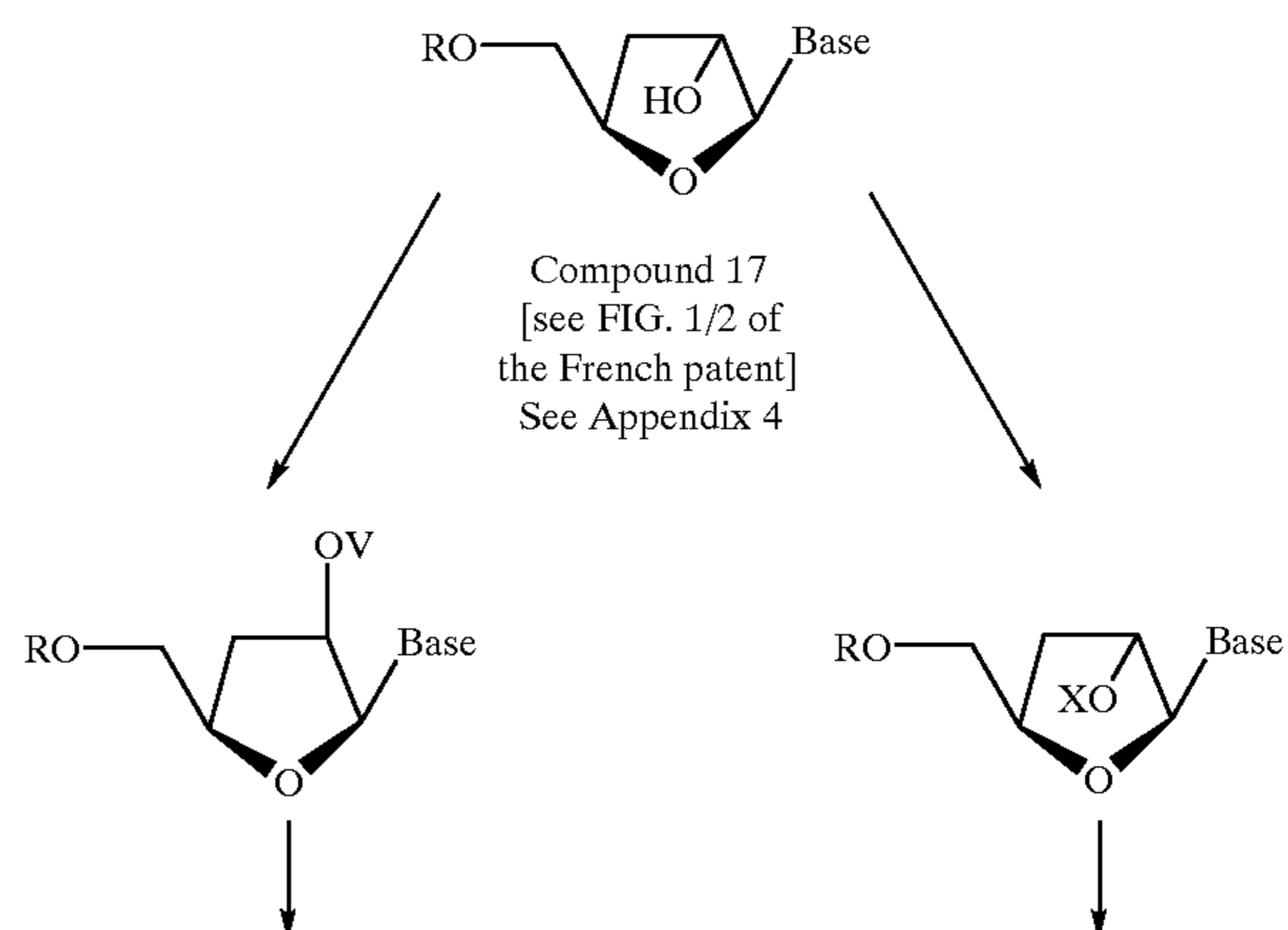
General Scheme for the Stereospecific Synthesis of 2'-substituted \beta -L-dideoxynucleosides
