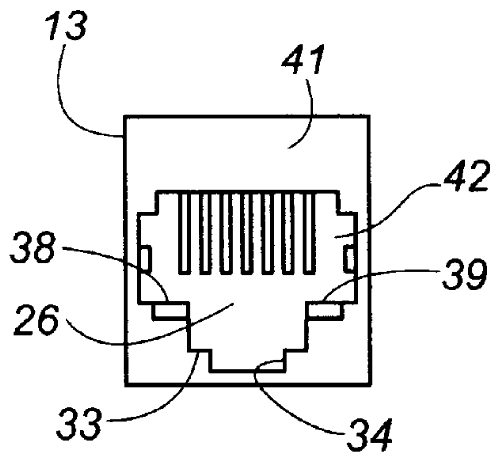
FIG. 3 (PRIOR ART)
