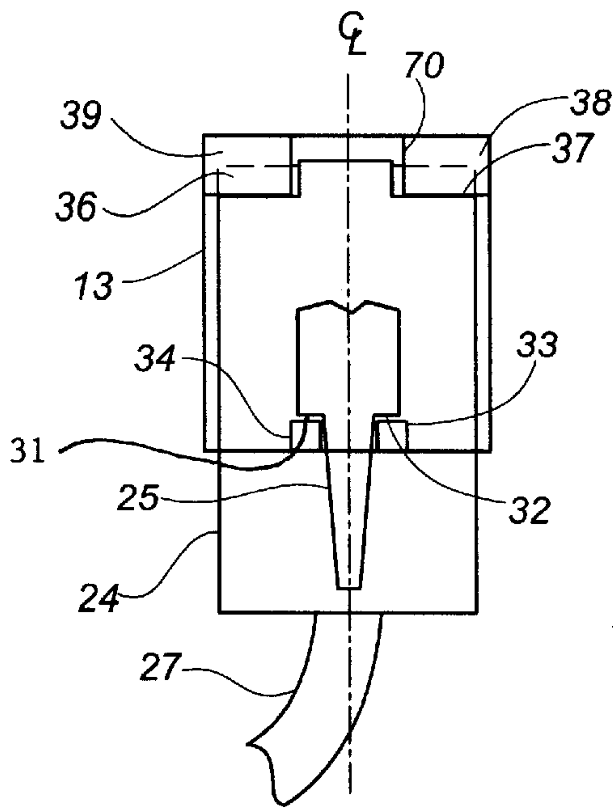
FIG. 6 (PRIOR ART)
