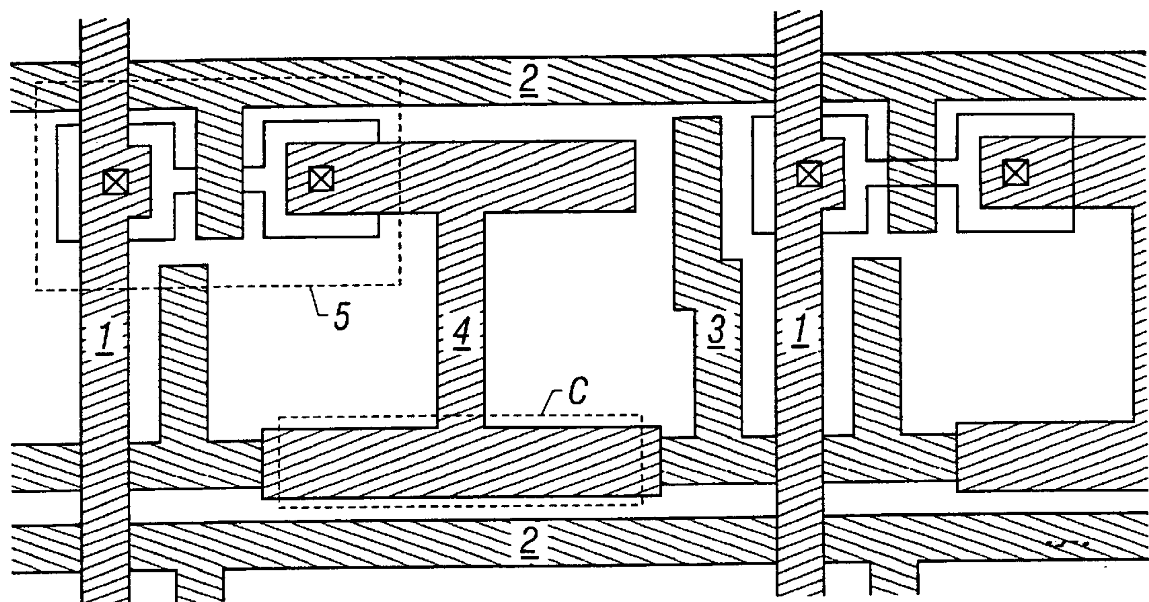
FIG. 6 (PRIOR ART)
