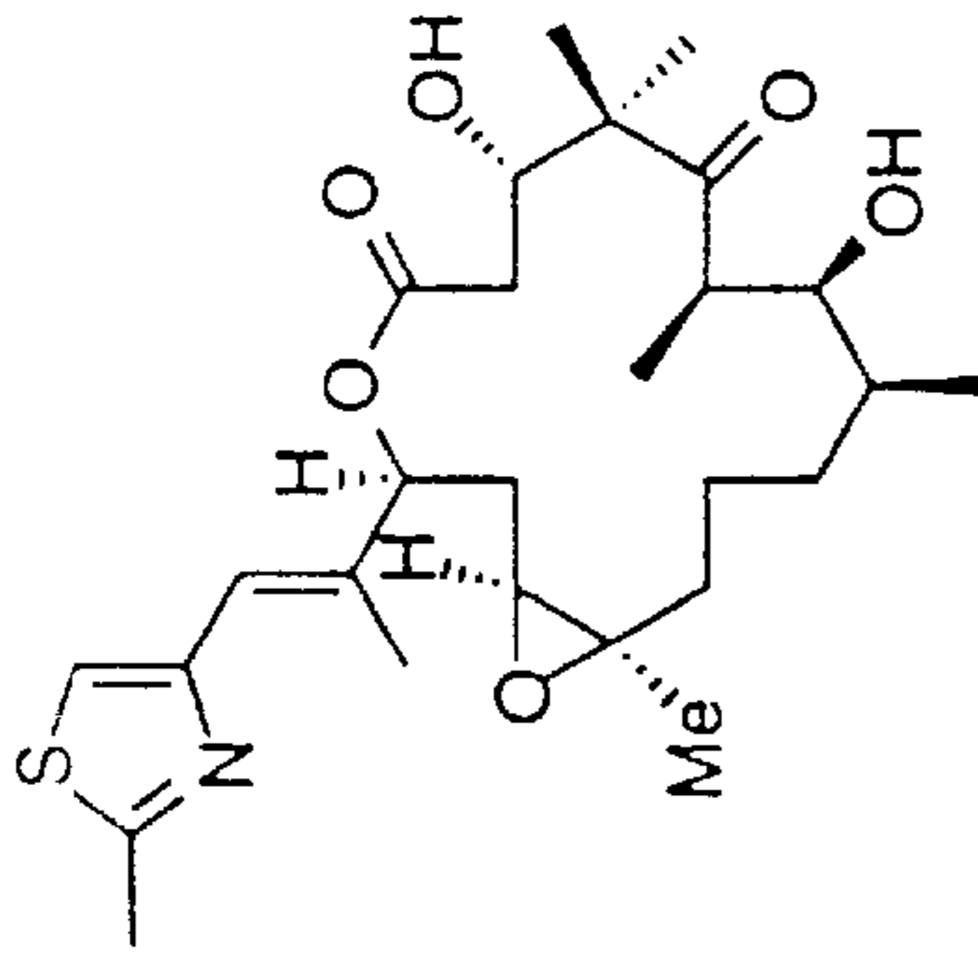
synthetic epothilone B
