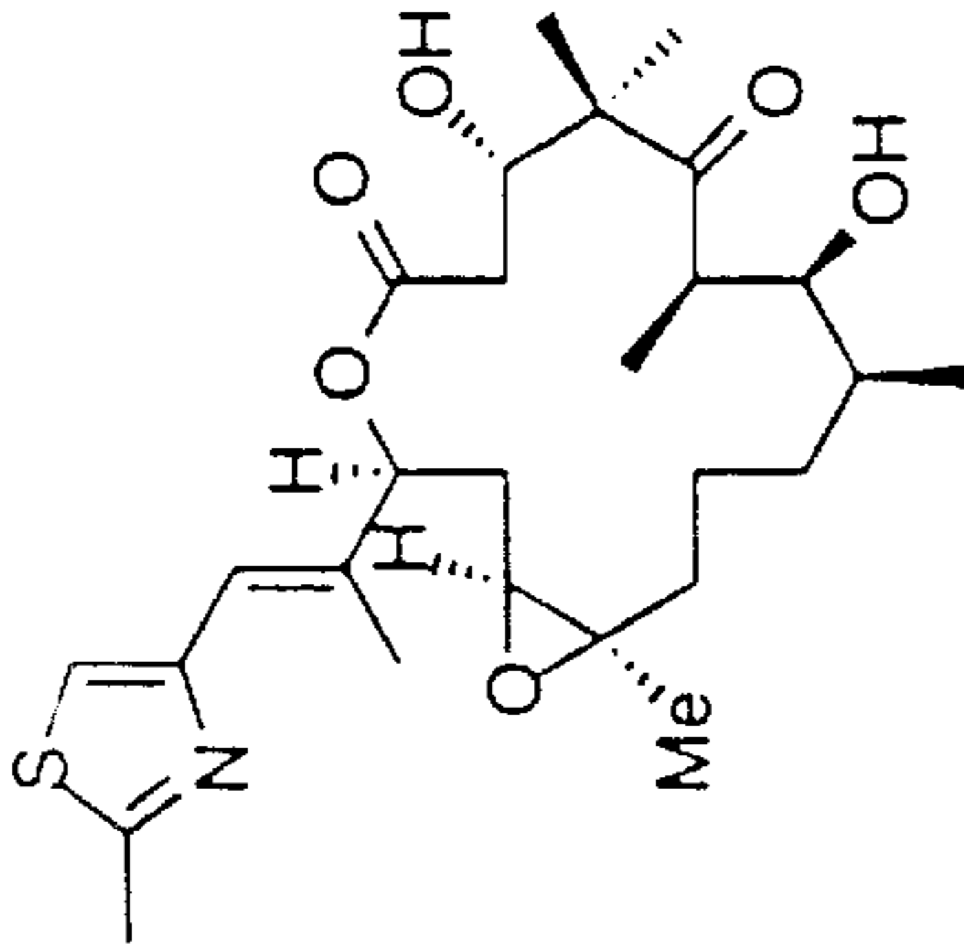
natural epothilone B
