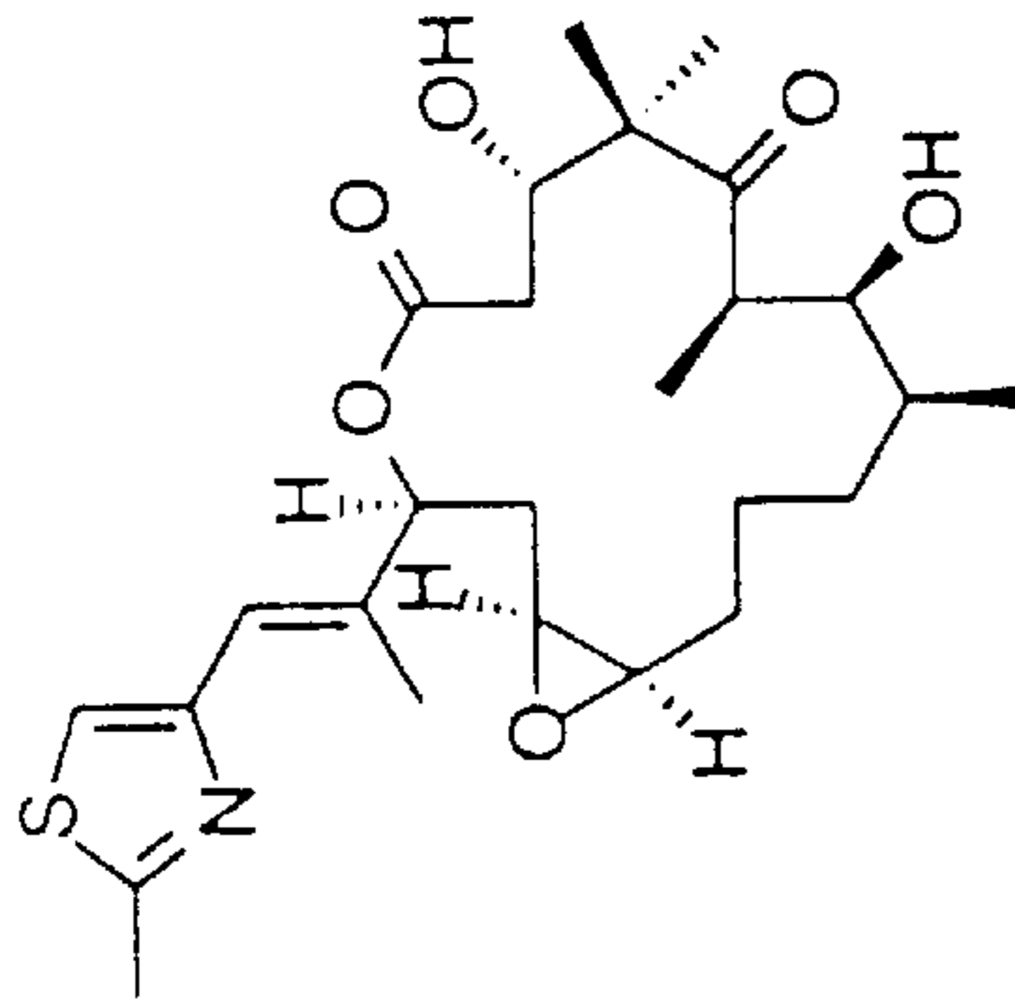
epothilone A
