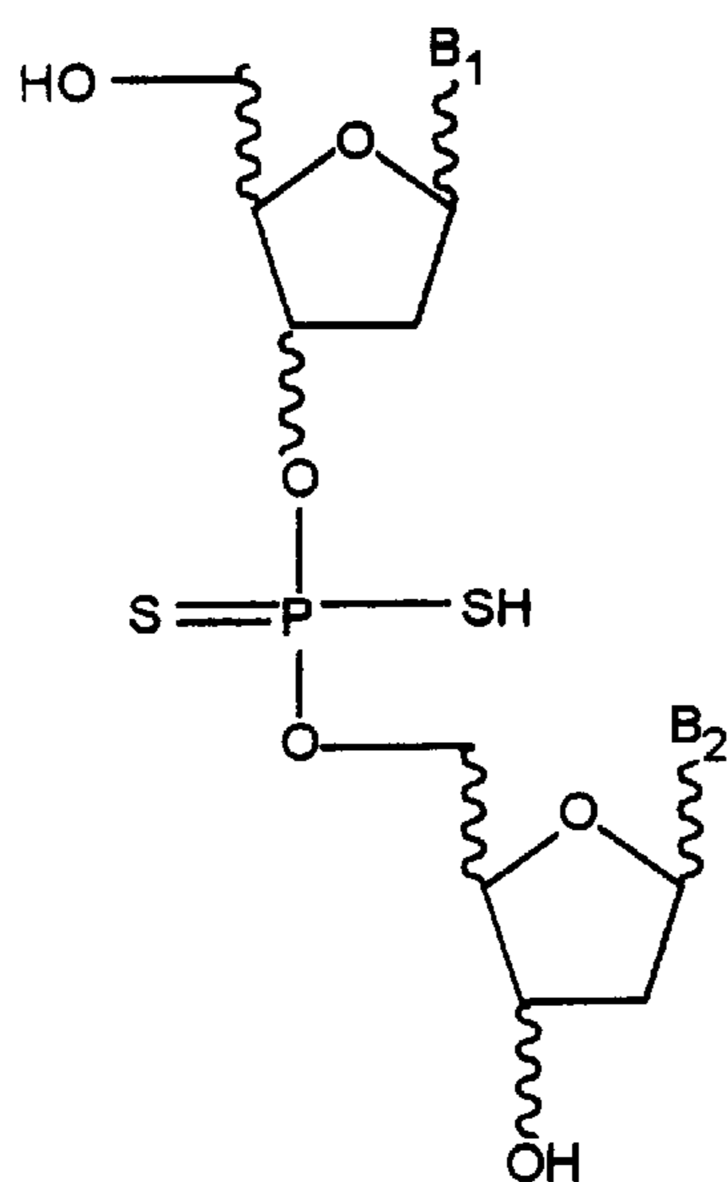
Phosphorodithioates
