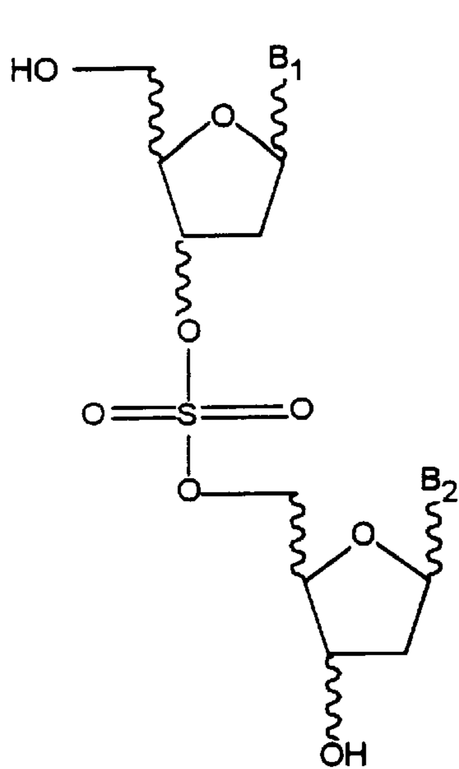
Sulfonates
