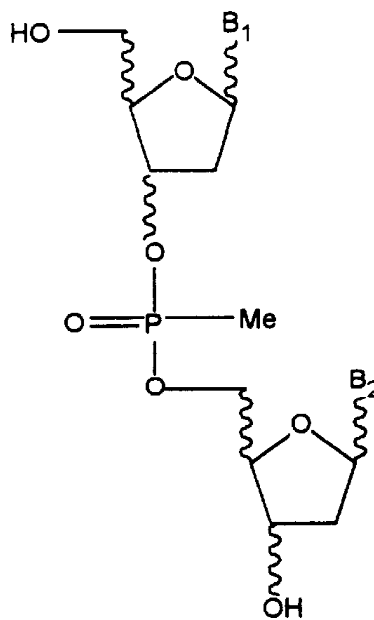
Methyl phosphonates
