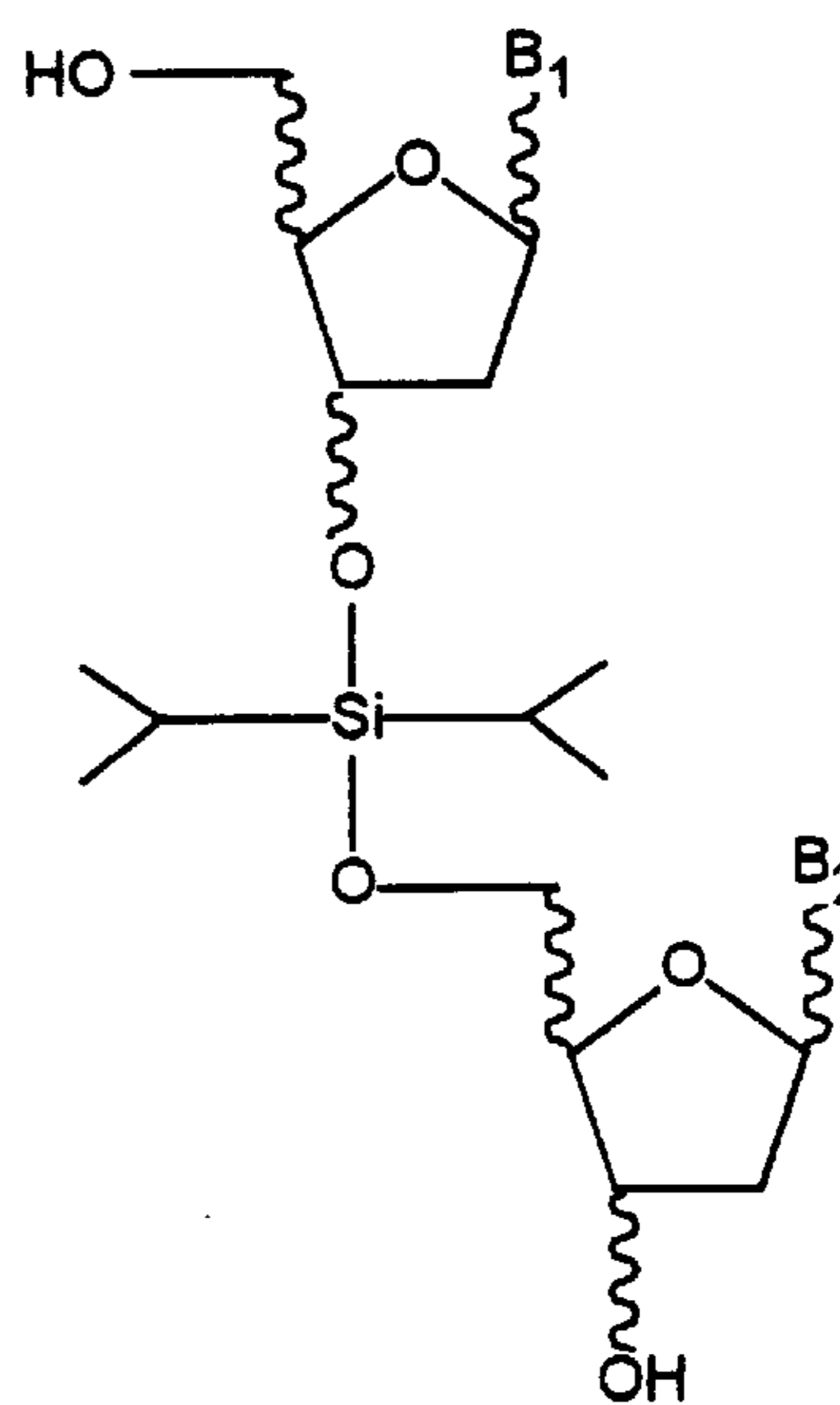
Silyl Ethers
