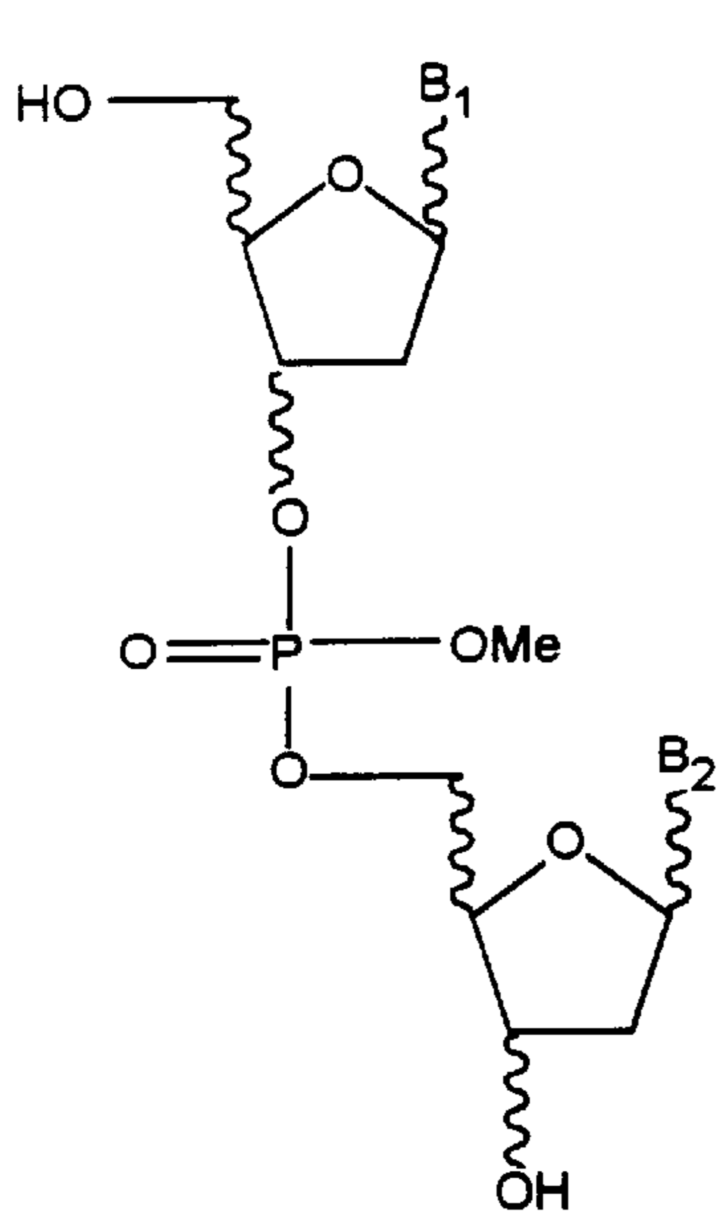
Methox phosphotriesters
