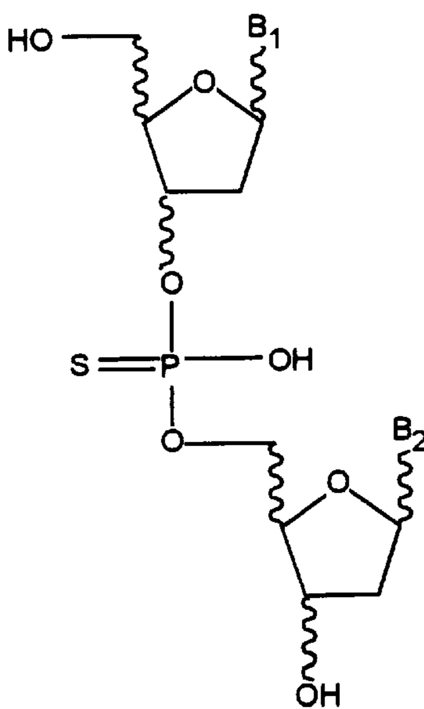
Phosphorothioates
