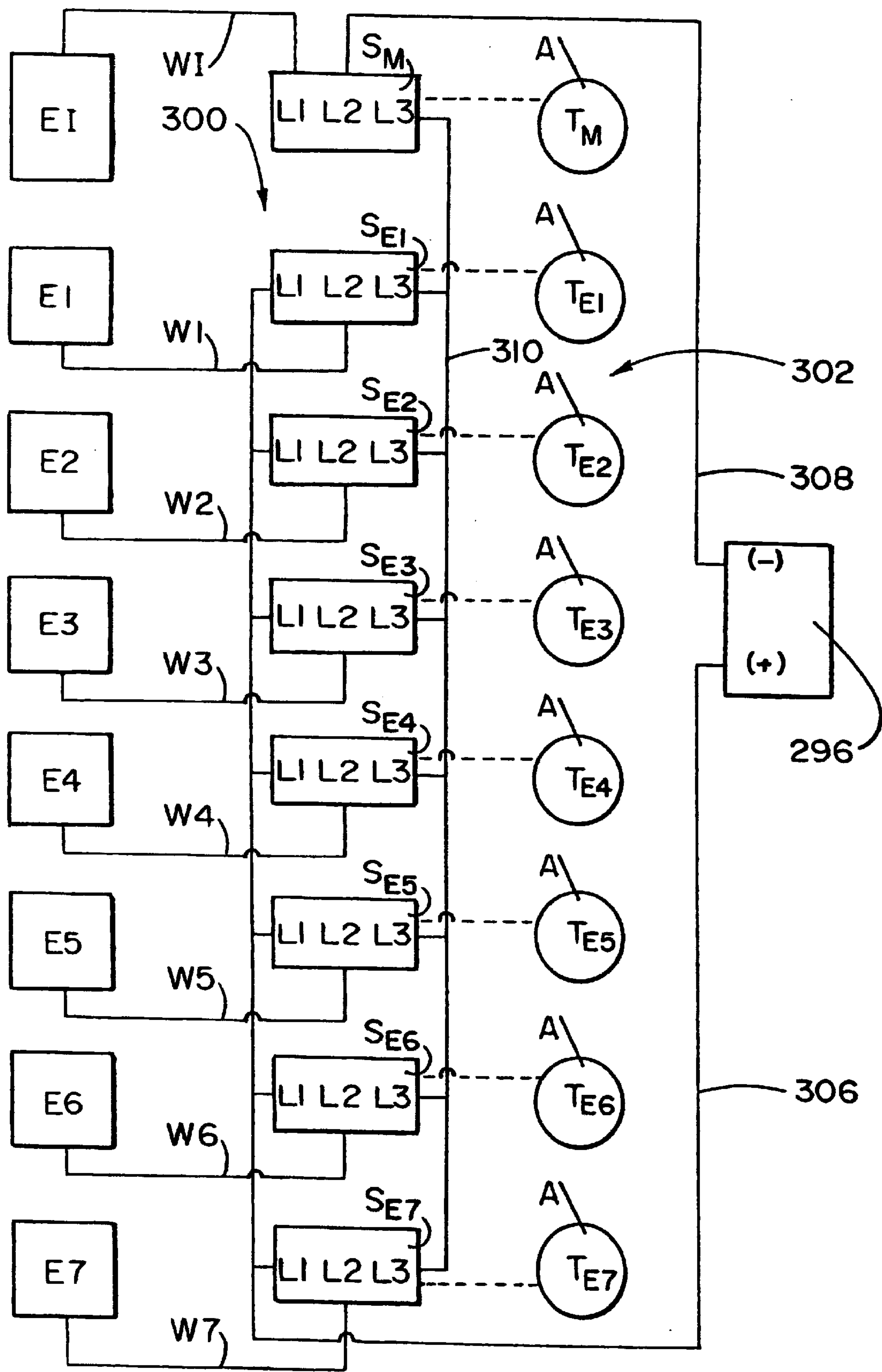
FIG. 63 UNIPOLAR CONTINUOUS
