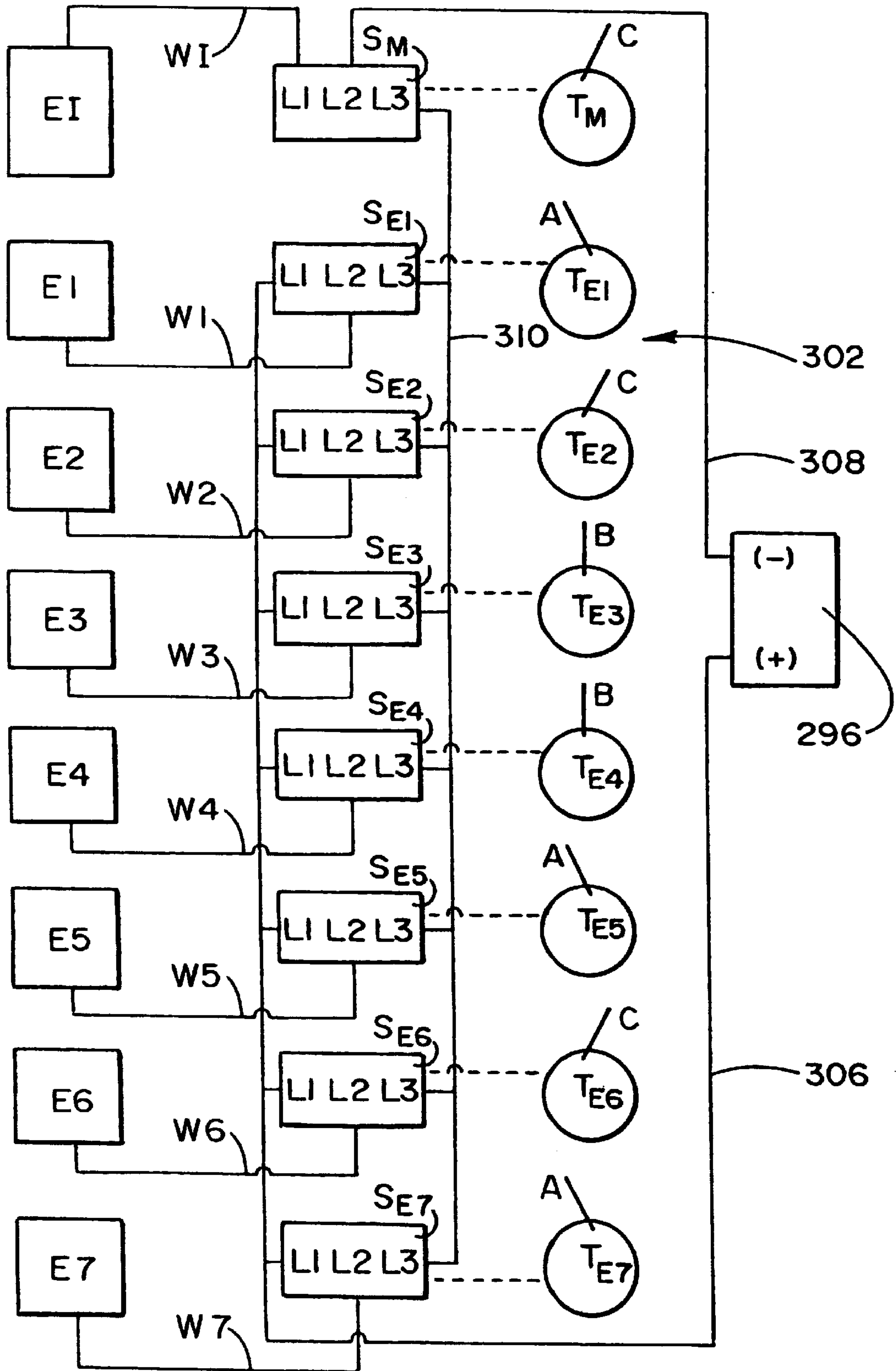
FIG. 66 BIPOlar INTERRUPTED
