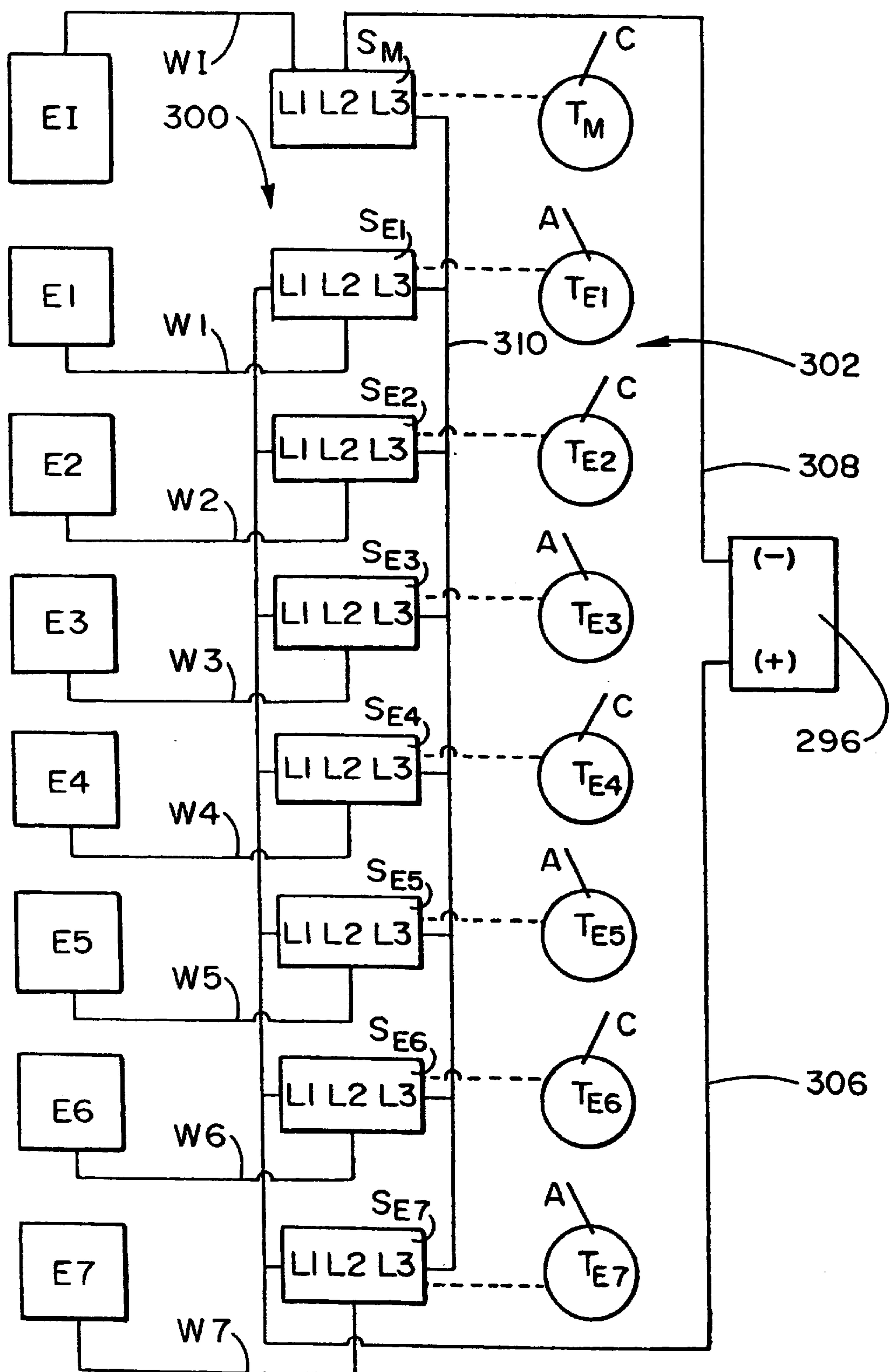
FIG. 65 BIPOLAR CONTINUOUS
