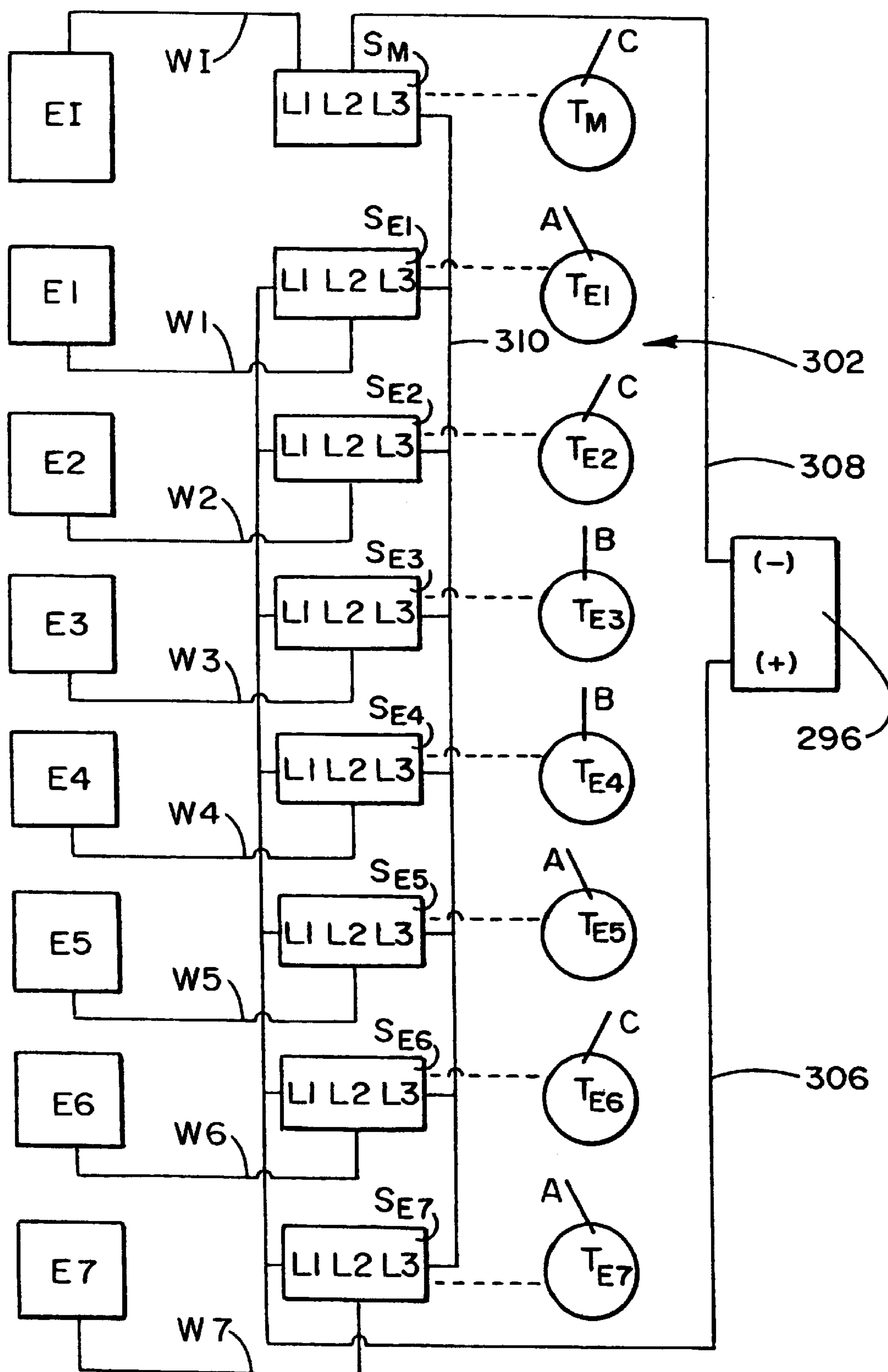
FIG. 66 BIPOLAR INTERRUPTED
