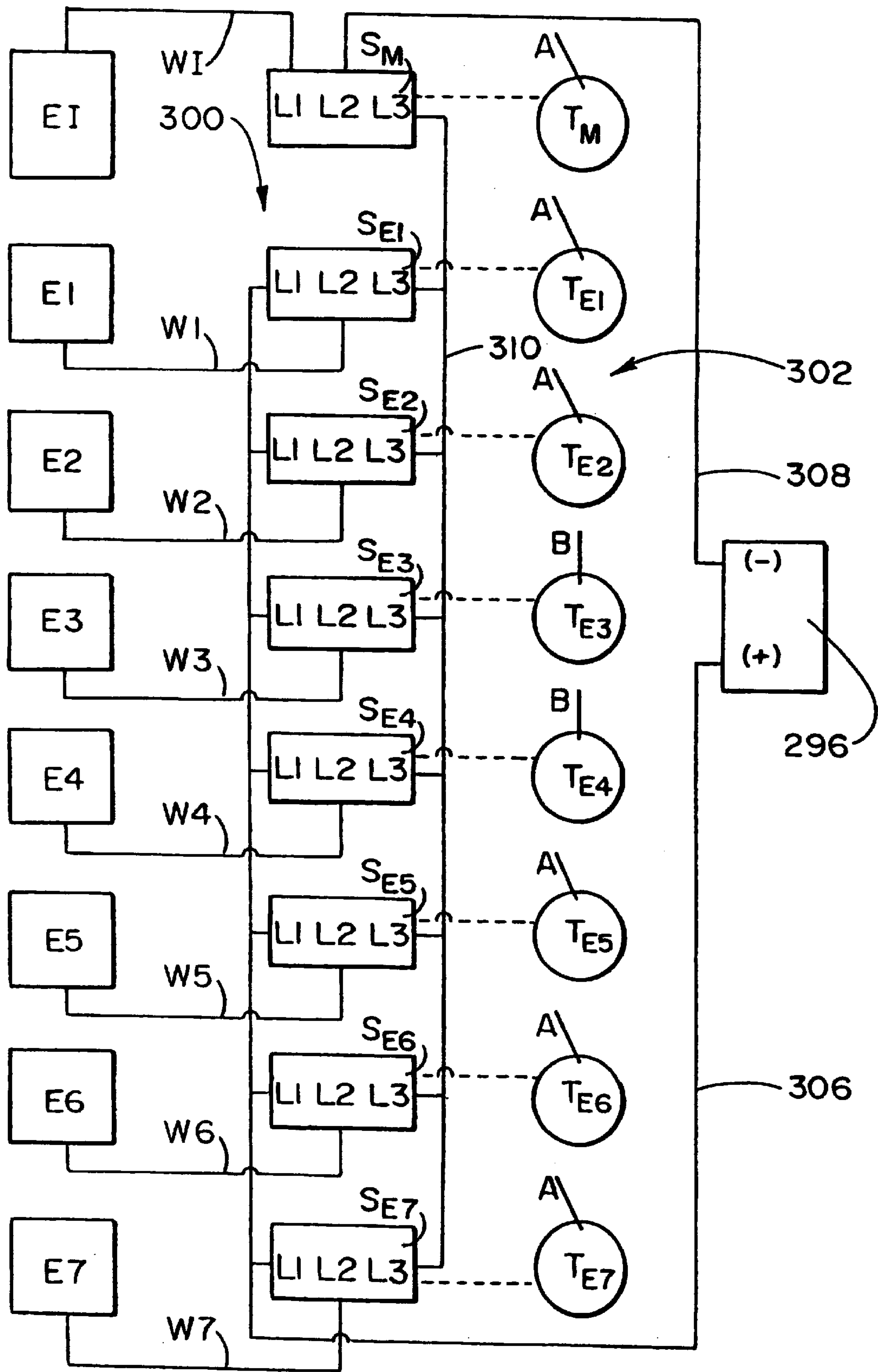
FIG. 64 UNIPOLAR INTERRUPTED
