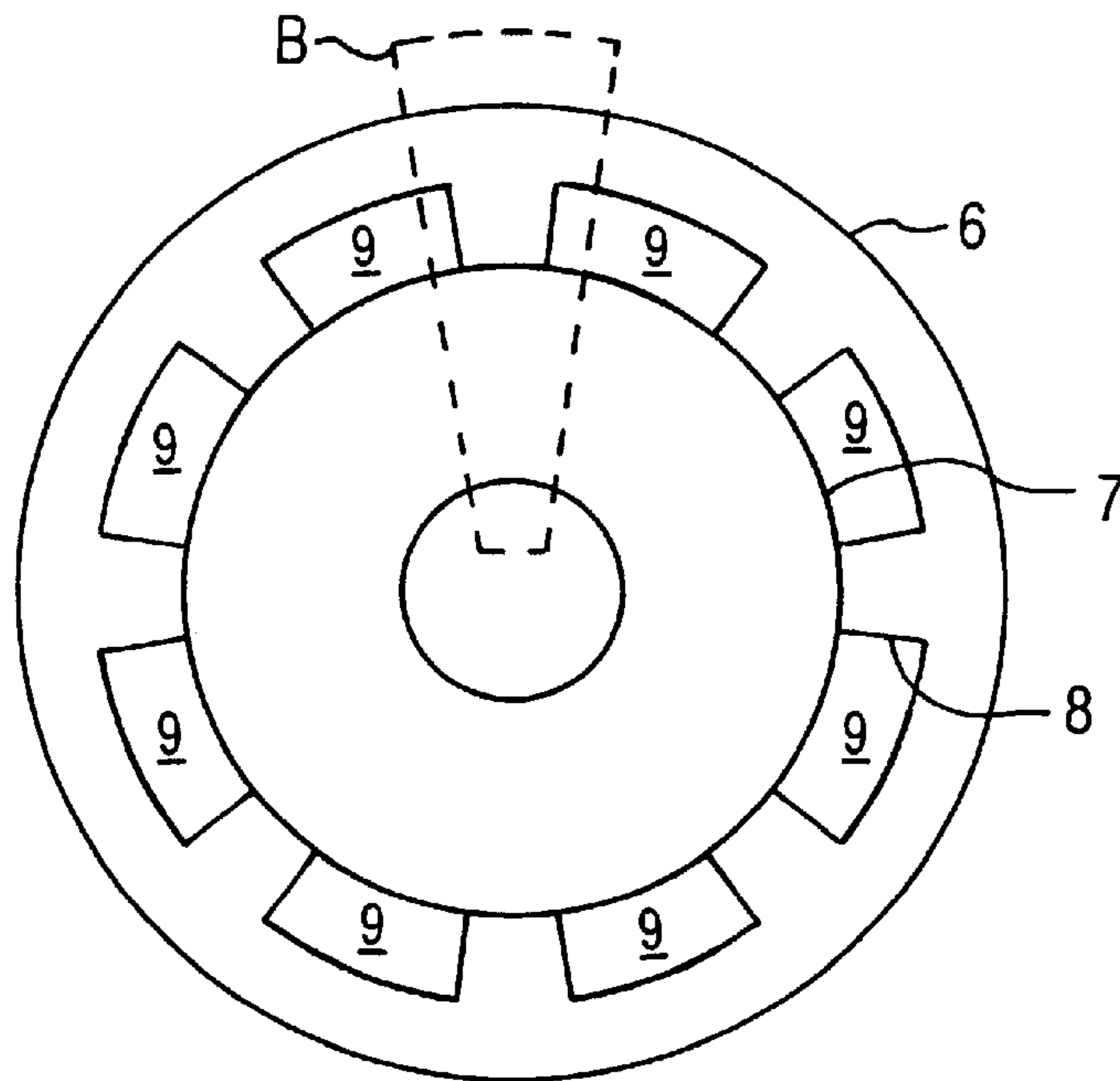
FIG. 3 (PRIOR ART)
