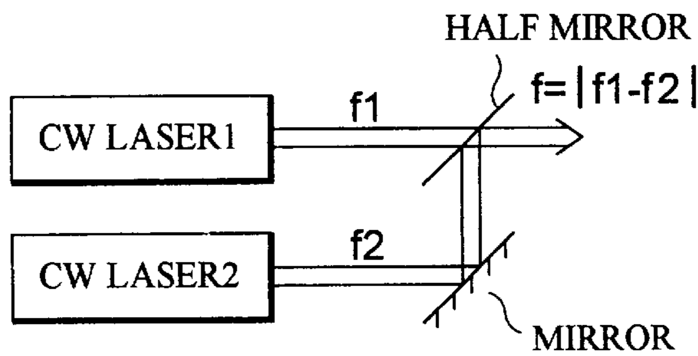
GENERATION OF MODULATED LIGHT BY USE OF BEAT (USING TWO CW LASERS)
