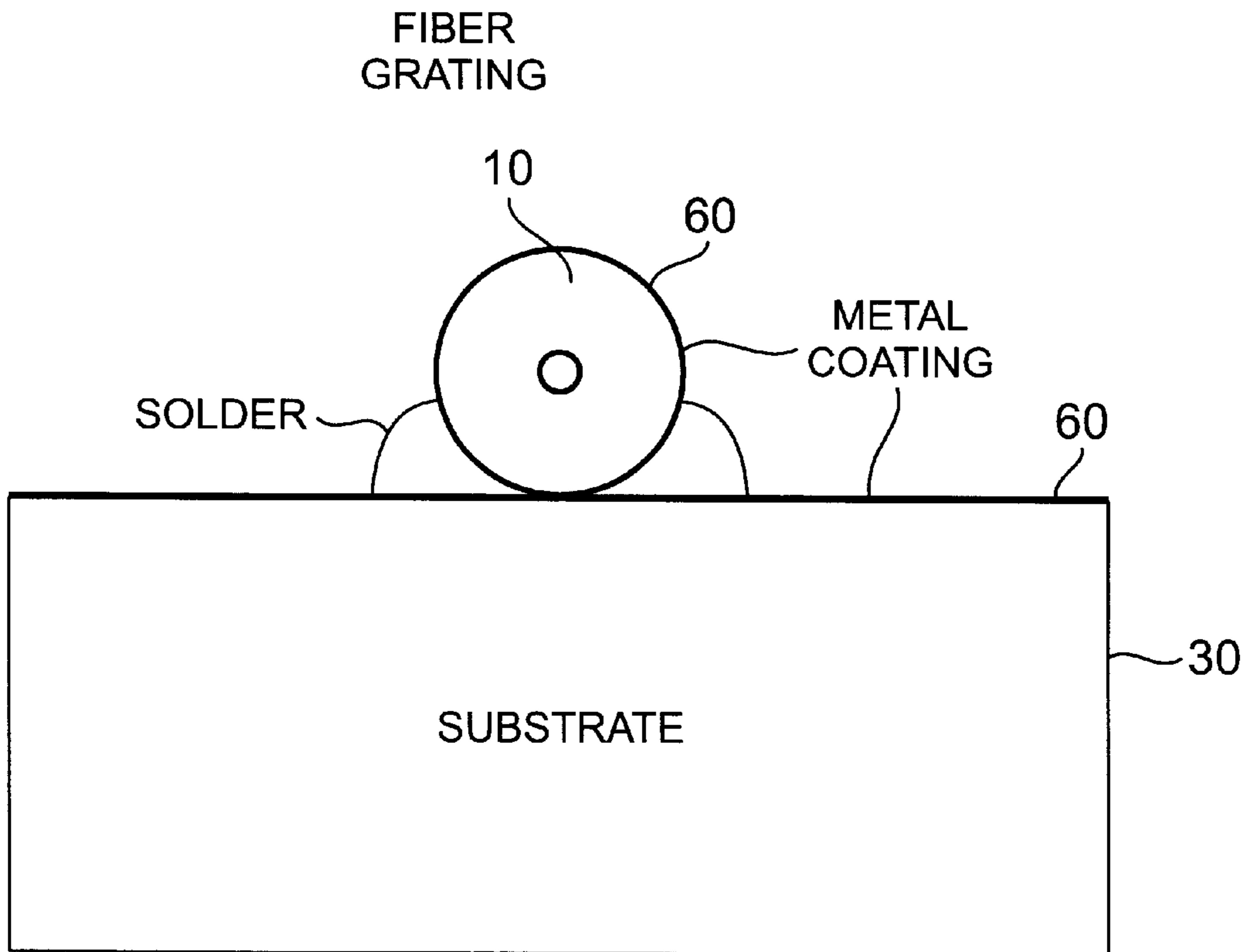
END VIEW
