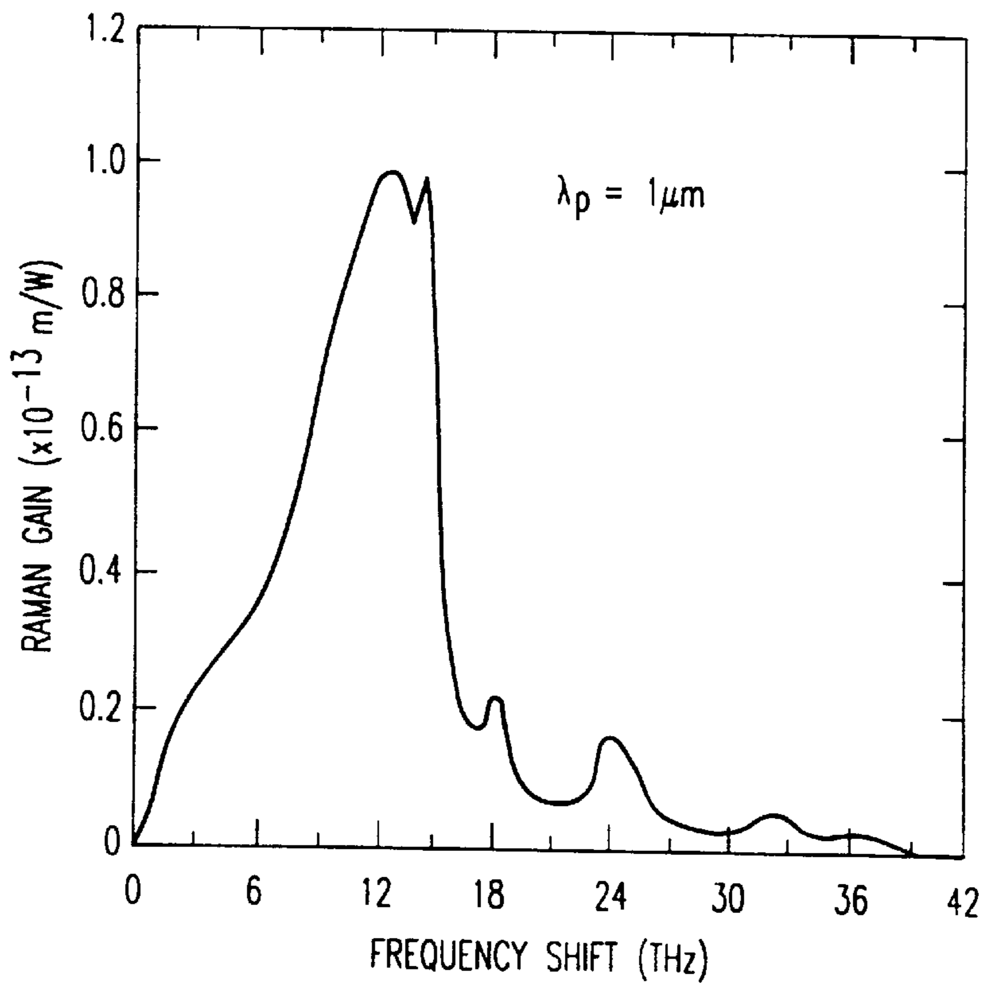
FIG.4 PRIOR ART
