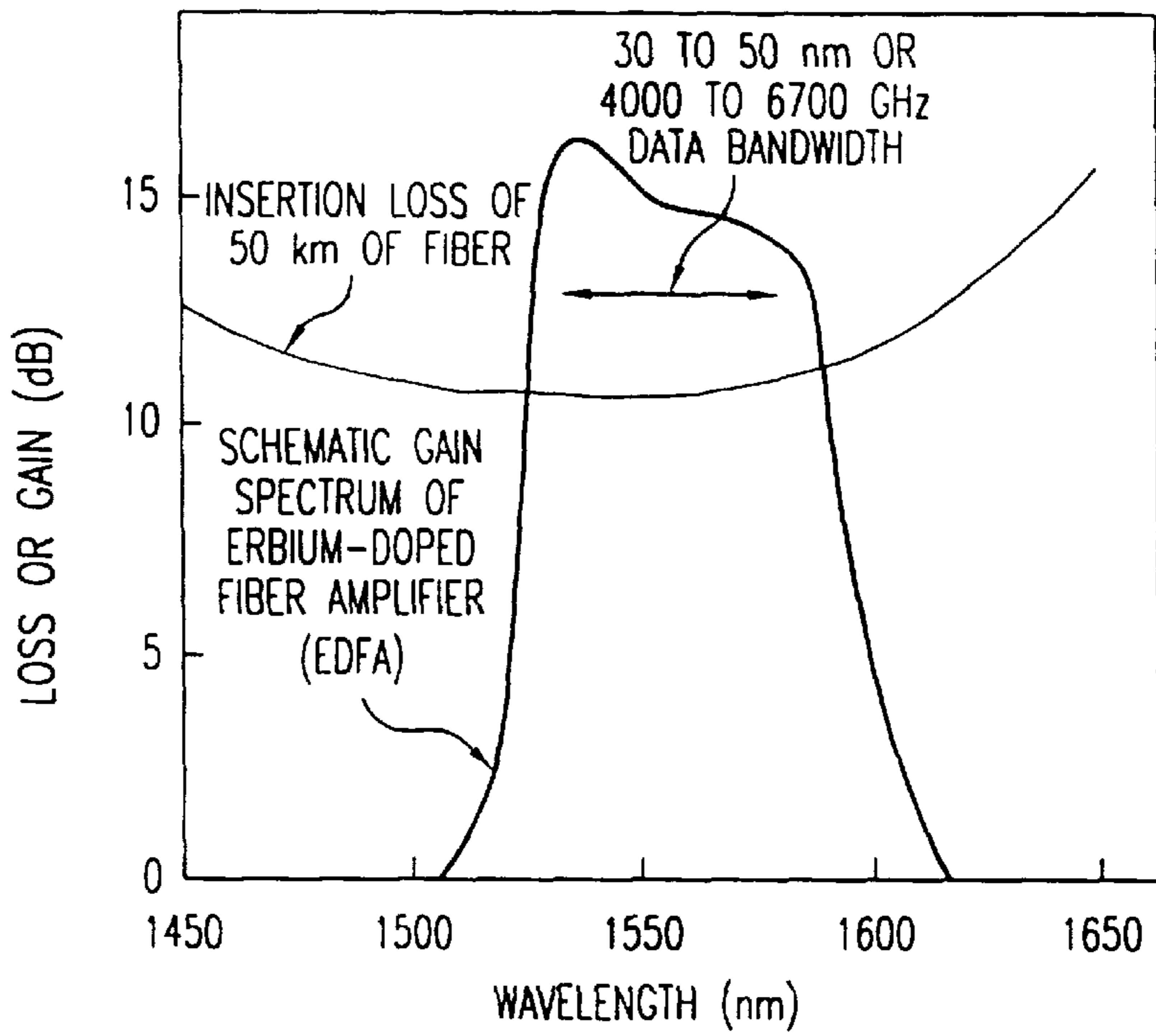
FIG. 1 PRIOR ART
